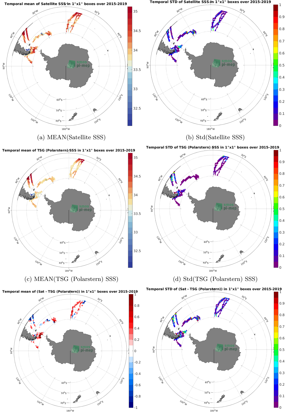
Figure 6: Temporal mean (left) and Std (right) of SSS from SMAP SSS L3 v5.0 - Monthly (JPL) (top), TSG (Polarstern) (middle), and of \Delta SSS (Satellite - TSG (Polarstern)). Only match-up pairs are used to generate these maps.
