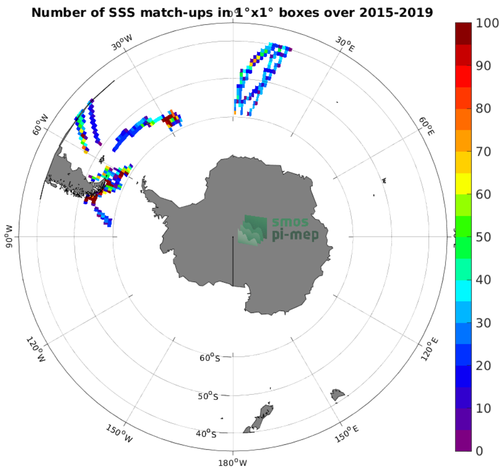
Figure 4: Number of SSS match-ups between TSG (Polarstern) SSS and the SMAP SSS L3 v5.0 - Monthly (JPL) SSS product for the Roaring Forties and Furious Fifties Pi-MEP region over 1^\circ \times 1^\circ boxes and for the full satellite product period.
