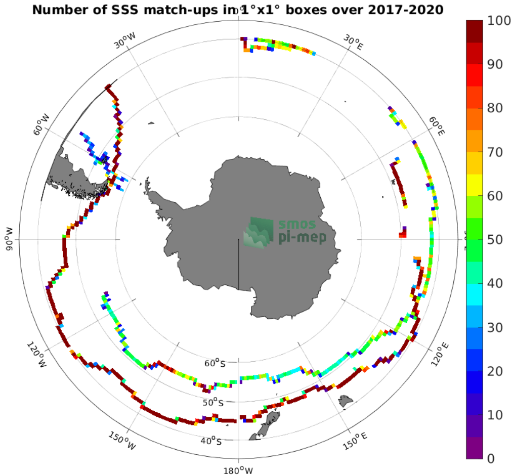
Figure 4: Number of SSS match-ups between TSG (GOSUD-Sailing-ship) SSS and the SMAP SSS L3 v5.0 - Monthly (JPL) SSS product for the Roaring Forties and Furious Fifties Pi-MEP region over 1^\circ \times 1^\circ boxes and for the full satellite product period.
