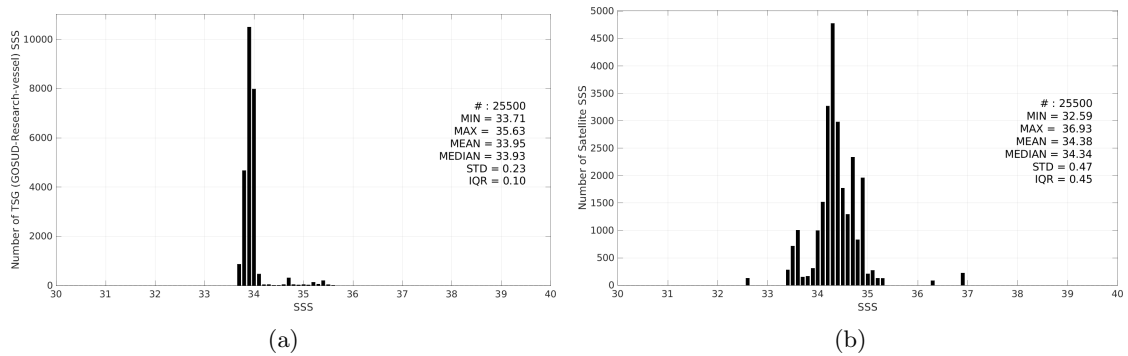
Figure 3: Histograms of SSS from TSG (GOSUD-Research-vessel) (a) and SMAP SSS L3 v5.0 - Monthly (JPL) (b) considering all match-up pairs per bins of 0.1 over the Roaring Forties and Furious Fifties Pi-MEP region and for the full satellite product period.
