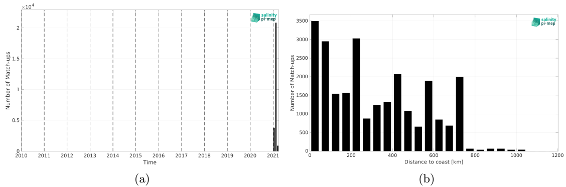
Figure 2: Number of match-ups between TSG (GOSUD-Research-vessel) and SMAP SSS L3 v5.0 - Monthly (JPL) SSS as a function of time (a) and as function of the distance to coast (b) over the Roaring Forties and Furious Fifties Pi-MEP region and for the full satellite product period.
