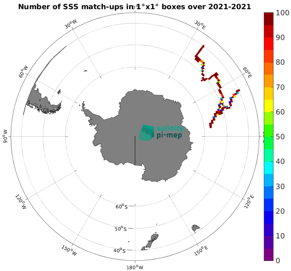
Figure 5: Number of SSS match-ups between TSG (GOSUD-Research-vessel) SSS and the SMAP SSS L3 v5.0 - Monthly (JPL) SSS product for the Roaring Forties and Furious Fifties Pi-MEP region over 1^{\circ} \times 1^{\circ} boxes and for the full satellite product period.
