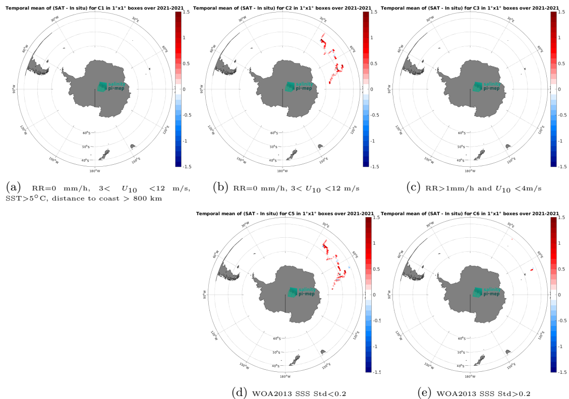
Figure 14: Temporal mean gridded over spatial boxes of size 1^\circ \times 1^\circ of \Delta SSS (SMAP SSS L3 v5.0 - Monthly (JPL) - TSG (GOSUD-Research-vessel)) for 5 different subdatasets corresponding to:RR=0 mm/h, 3 < U_{10} < 12 m/s, SST >5^\circ C, distance to coast > 800 km (a), RR=0 mm/h, 3 < U_{10} < 12 m/s (b), RR >1 mm/h and U_{10} < 4 m/s (c), WOA2013 SSS Std <0.2 (d), WOA2013 SSS Std >0.2 (e).
