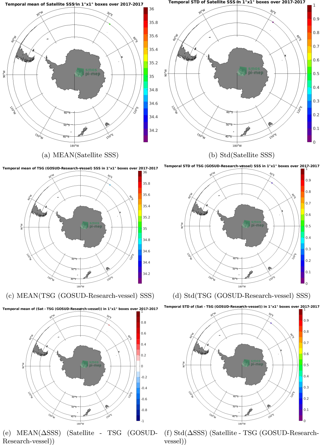
Figure 6: Temporal mean (left) and Std (right) of SSS from SMAP SSS L3 v5.0 - Monthly (JPL) (top), TSG (GOSUD-Research-vessel) (middle), and of \Delta SSS (Satellite - TSG (GOSUD-Research-vessel)). Only match-up pairs are used to generate these maps.
