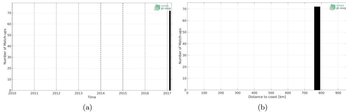
Figure 1: Number of match-ups between TSG (GOSUD-Research-vessel) and SMAP SSS L3 v5.0 - Monthly (JPL) SSS as a function of time (a) and as function of the distance to coast (b) over the Roaring Forties and Furious Fifties Pi-MEP region and for the full satellite product period.
