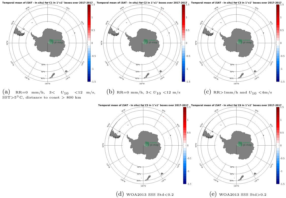
Figure 12: Temporal mean gridded over spatial boxes of size 1°x1° of \Delta SSS (SMAP SSS L3 v5.0 - Monthly (JPL) - TSG (GOSUD-Research-vessel)) for 5 different subdatasets corresponding to:RR=0 mm/h, 3 < U_{10} < 12 m/s, SST>5°C, distance to coast > 800 km (a), RR=0 mm/h, 3 < U_{10} < 12 m/s (b), RR>1mm/h and U_{10} < 4 m/s (c), WOA2013 SSS Std<0.2 (d), WOA2013 SSS Std>0.2 (e).
