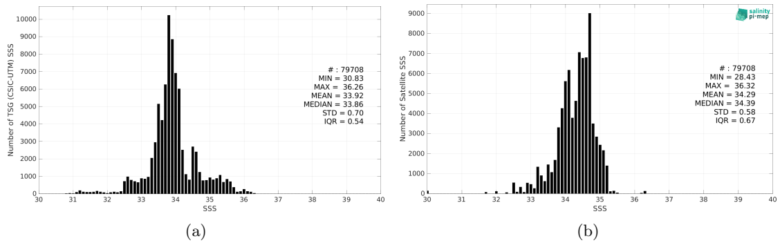
Figure 2: Histograms of SSS from TSG (CSIC-UTM) (a) and SMAP SSS L3 v5.0 - Monthly (JPL) (b) considering all match-up pairs per bins of 0.1 over the Roaring Forties and Furious Fifties Pi-MEP region and for the full satellite product period.
