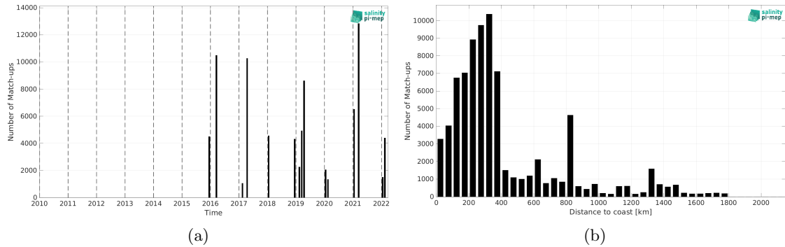
Figure 1: Number of match-ups between TSG (CSIC-UTM) and SMAP SSS L3 v5.0 - Monthly (JPL) SSS as a function of time (a) and as function of the distance to coast (b) over the Roaring Forties and Furious Fifties Pi-MEP region and for the full satellite product period.
