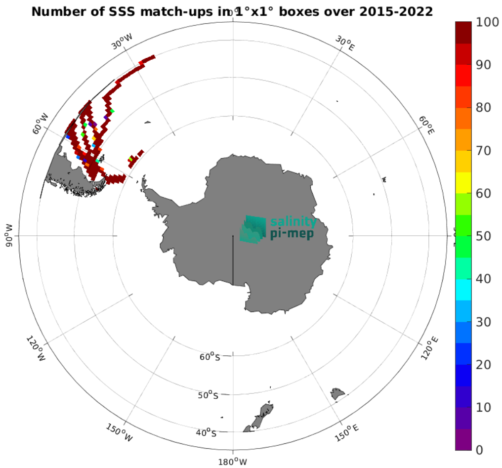
Figure 4: Number of SSS match-ups between TSG (CSIC-UTM) SSS and the SMAP SSS L3 v5.0 - Monthly (JPL) SSS product for the Roaring Forties and Furious Fifties Pi-MEP region over 1^\circ \times 1^\circ boxes and for the full satellite product period.
