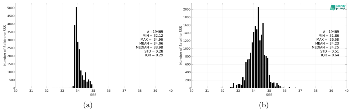
Figure 2: Histograms of SSS from Saildrone (a) and SMAP SSS L3 v5.0 - Monthly (JPL) (b) considering all match-up pairs per bins of 0.1 over the Roaring Forties and Furious Fifties Pi-MEP region and for the full satellite product period.
