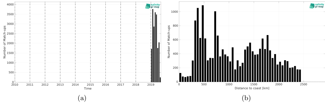
Figure 1: Number of match-ups between Saildrone and SMAP SSS L3 v5.0 - Monthly (JPL) SSS as a function of time (a) and as function of the distance to coast (b) over the Roaring Forties and Furious Fifties Pi-MEP region and for the full satellite product period.
