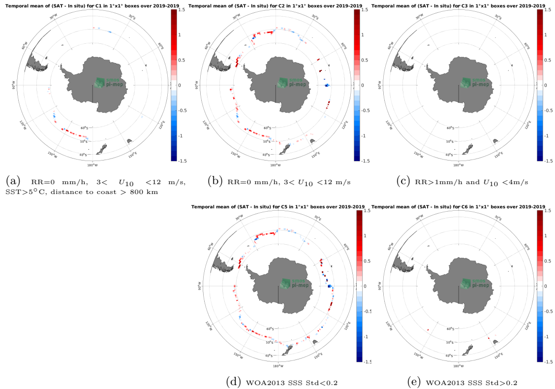
Figure 12: Temporal mean gridded over spatial boxes of size 1^{\circ}\times 1^{\circ} of \Delta\text{SSS} (SMAP SSS L3 v5.0 - Monthly (JPL) - Saicdrone) for 5 different subdatasets corresponding to:RR=0 mm/h, 3 < U_{10} < 12 m/s, SST >5^{\circ}\text{C} , distance to coast > 800 km (a), RR=0 mm/h, 3 < U_{10} < 12 m/s (b), RR >1 mm/h and U_{10} < 4 m/s (c), WOA2013 SSS Std <0.2 (d), WOA2013 SSS Std >0.2 (e).
