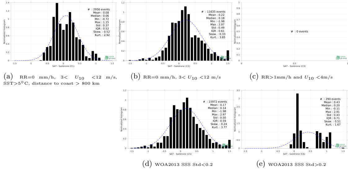
Figure 13: Normalized histogram of \Delta SSS (SMAP SSS L3 v5.0 - Monthly (JPL) - Salldrone) for 5 different subdatasets corresponding to: RR=0 mm/h, 3 < U_{10} < 12 m/s, SST > 5°C, distance to coast > 800 km (a), RR=0 mm/h, 3 < U_{10} < 12 m/s (b), RR > 1mm/h and U_{10} < 4 m/s (c), WOA2013 SSS Std < 0.2 (d), WOA2013 SSS Std > 0.2 (e).
