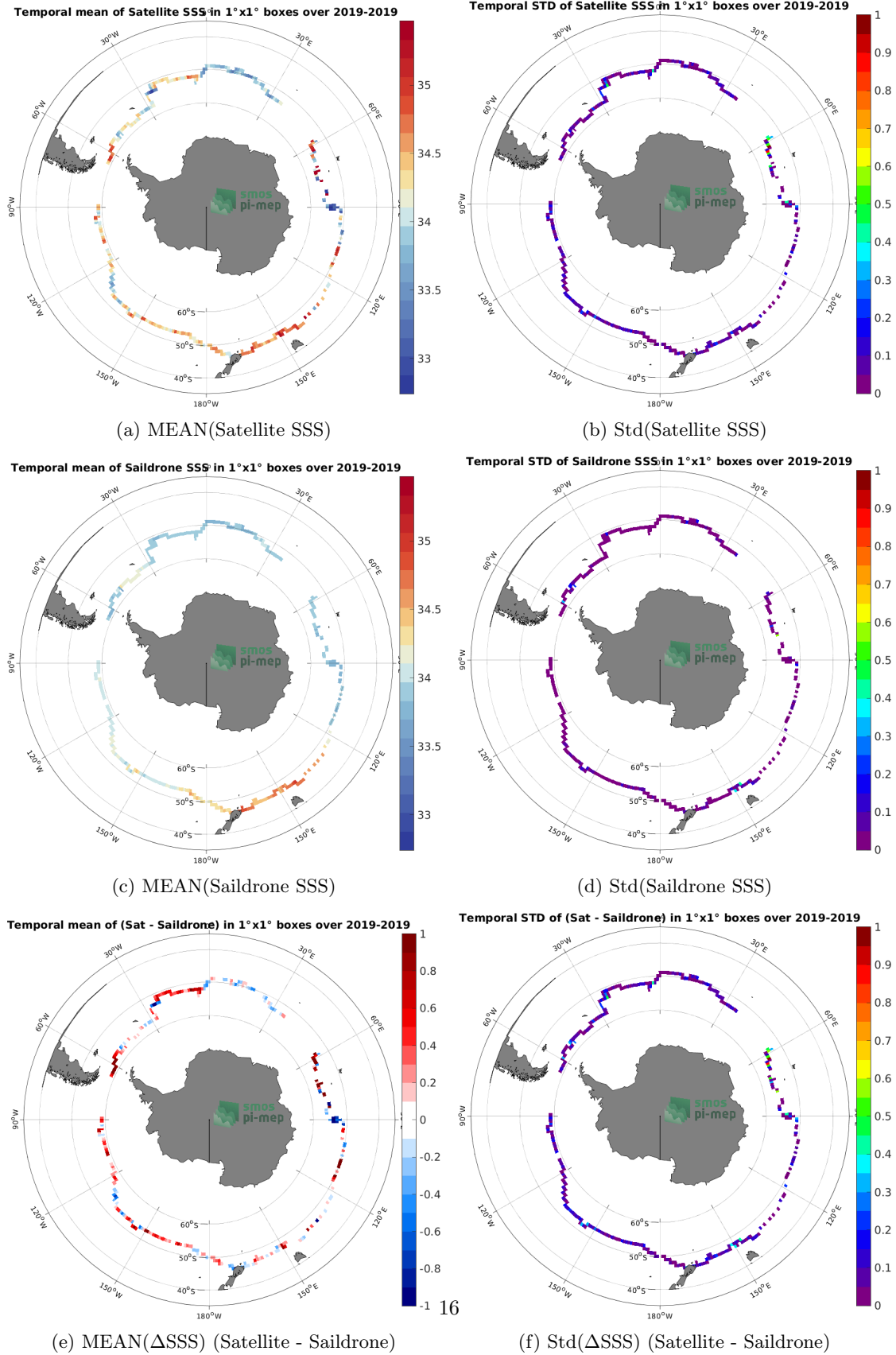
Figure 6: Temporal mean (left) and Std (right) of SSS from SMAP SSS L3 v5.0 - Monthly (JPL) (top), Saildrone (middle), and of \Delta SSS (Satellite - Saildrone). Only match-up pairs are used to generate these maps.
