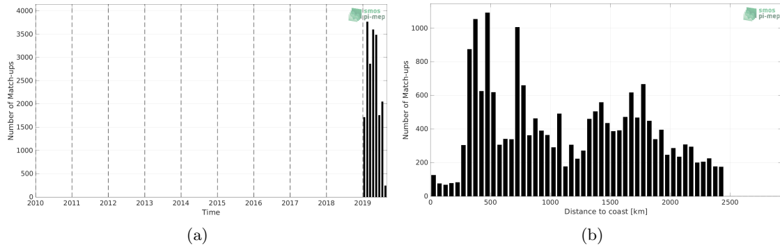
Figure 1: Number of match-ups between Sairdrone and SMAP SSS L3 v5.0 - Monthly (JPL) SSS as a function of time (a) and as function of the distance to coast (b) over the Roaring Forties and Furious Fifties Pi-MEP region and for the full satellite product period.
