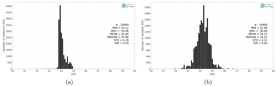
Figure 2: Histograms of SSS from Sairdrone (a) and SMAP SSS L3 v5.0 - Monthly (JPL) (b) considering all match-up pairs per bins of 0.1 over the Roaring Forties and Furious Fifties Pi-MEP region and for the full satellite product period.
