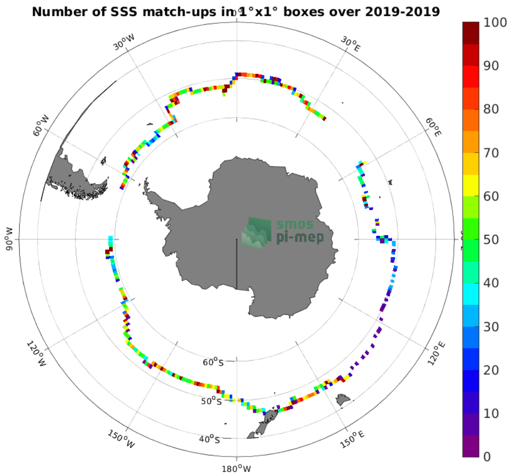
Figure 4: Number of SSS match-ups between Saildrone SSS and the SMAP SSS L3 v5.0 - Monthly (JPL) SSS product for the Roaring Forties and Furious Fifties Pi-MEP region over 1^\circ \times 1^\circ boxes and for the full satellite product period.
