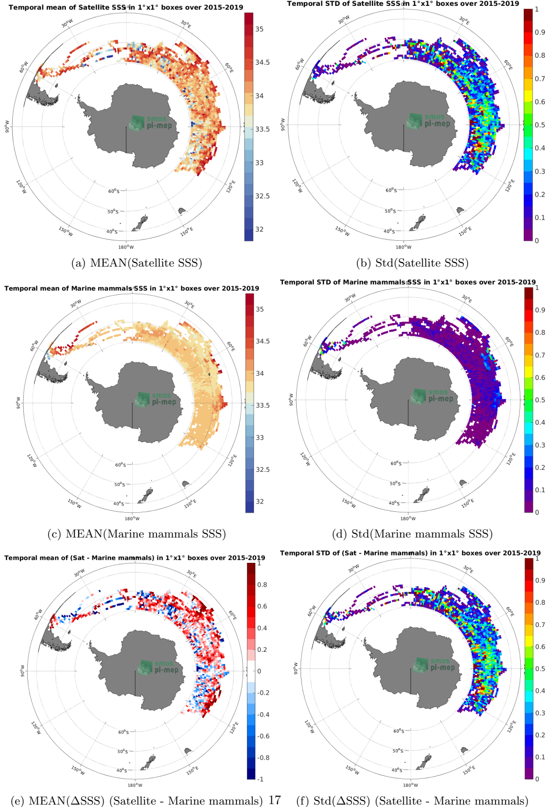
Figure 6: Temporal mean (left) and Std (right) of SSS from SMAP SSS L3 v5.0 - Monthly (JPL) (top), Marine mammals (middle), and of \Delta SSS (Satellite - Marine mammals). Only match-up pairs are used to generate these maps.
