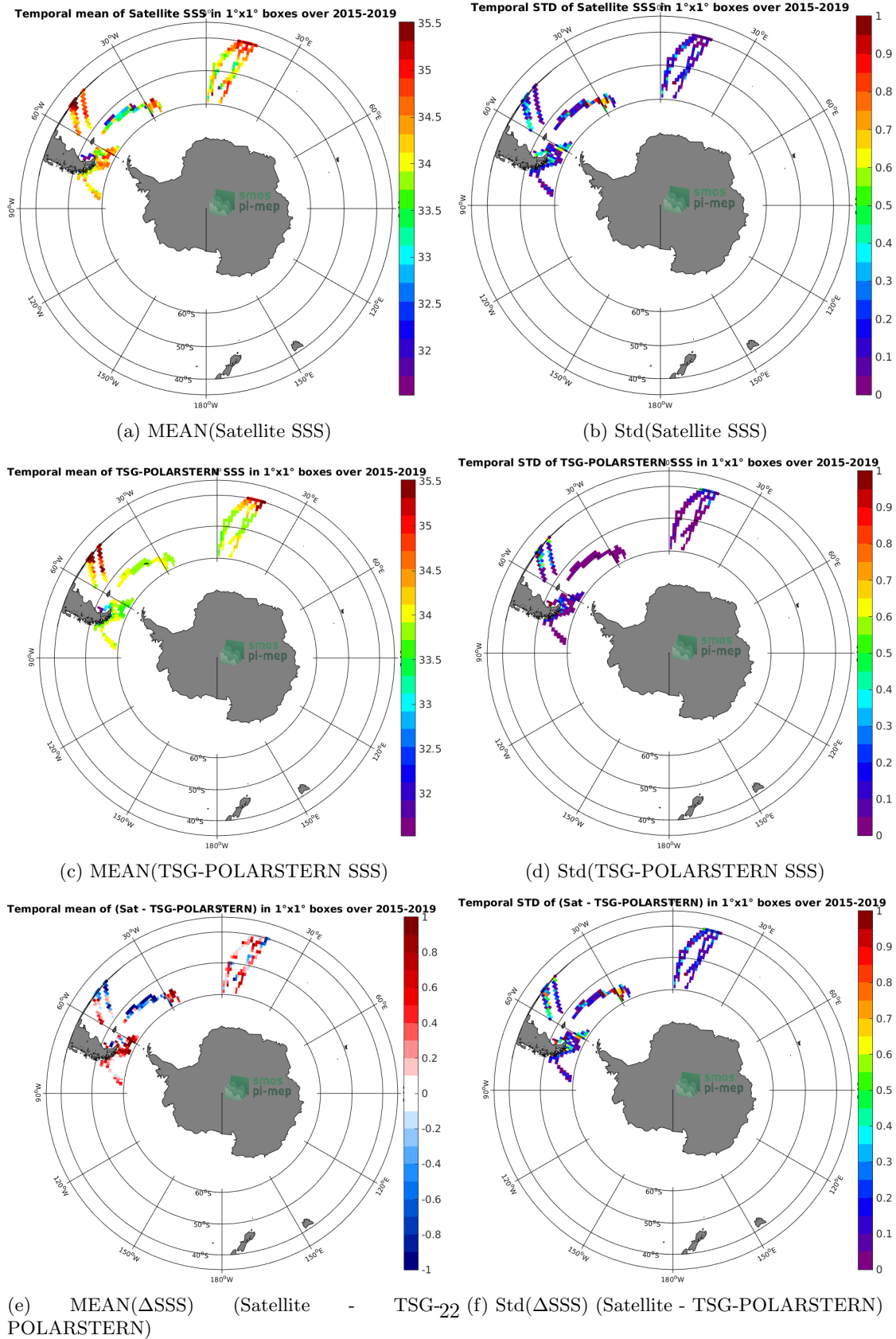
Figure 6: Temporal mean (left) and Std (right) of SSS from SMAP-L3-JPL-V4.3-8DAY-RUNNING-60KM (top), TSG-POLARSTERN (middle), and of \Delta SSS (Satellite - TSG-POLARSTERN). Only match-up pairs are used to generate these maps.
