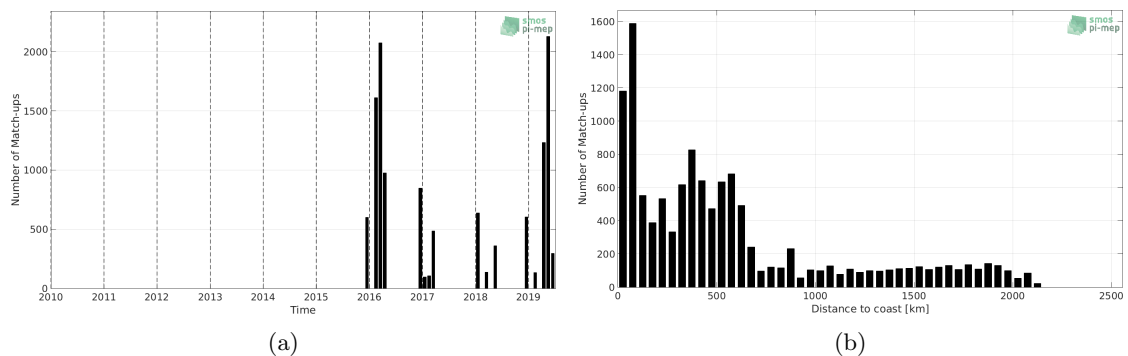
Figure 1: Number of match-ups between TSG-POLARSTERN and SMAP-L3-JPL-V4.3-8DAY-RUNNING-60KM SSS as a function of time (a) and as function of the distance to coast (b) over the Roaring Forties and Furious Fifties Pi-MEP region and for the full satellite product period.
