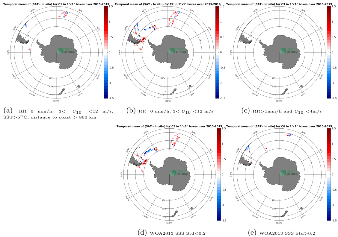
Figure 12: Temporal mean gridded over spatial boxes of size 1^{\circ}\times 1^{\circ} of \Delta\text{SSS} (SMAP-L3-JPL-V4.3-8DAY-RUNNING-60KM - TSG-POLARSTERN) for 5 different subdatasets corresponding to:RR=0 mm/h, 3 < U_{10} < 12 m/s, SST >5^{\circ}\text{C} , distance to coast > 800 km (a), RR=0 mm/h, 3 < U_{10} < 12 m/s (b), RR >1 mm/h and U_{10} < 4 m/s (c), WOA2013 SSS Std <0.2 (d), WOA2013 SSS Std >0.2 (e).
