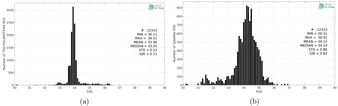
Figure 2: Histograms of SSS from TSG-POLARSTERN (a) and SMAP-L3-JPL-V4.3-8DAY-RUNNING-60KM (b) considering all match-up pairs per bins of 0.1 over the Roaring Forties and Furious Fifties Pi-MEP region and for the full satellite product period.
