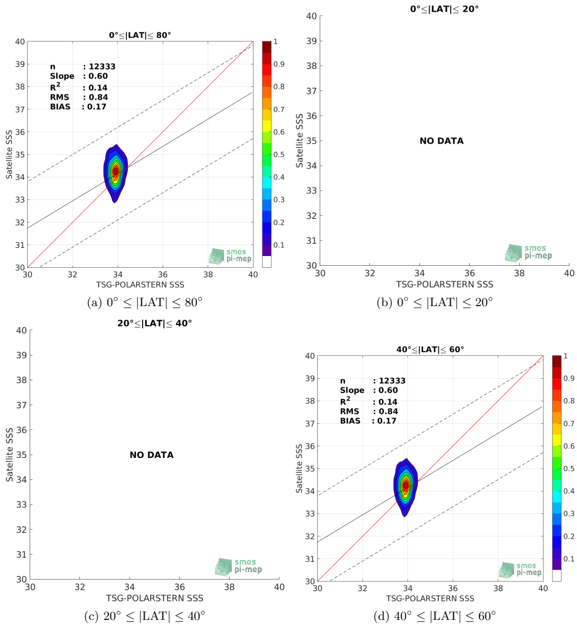
Figure 9: Contour maps of the concentration of SMAP-L3-JPL-V4.3-8DAY-RUNNING-60KM SSS (y-axis) versus TSG-POLARSTERN SSS (x-axis) at match-up pairs for different latitude bands. For each plot, the red line shows x=y . The black thin and dashed lines indicate a linear fit through the data cloud and the \pm 95\% confidence levels, respectively. The number match-up pairs n , the slope and R^2 coefficient of the linear fit, the root mean square (RMS) and the mean bias between satellite and in situ data are indicated for each latitude band in each plots.
