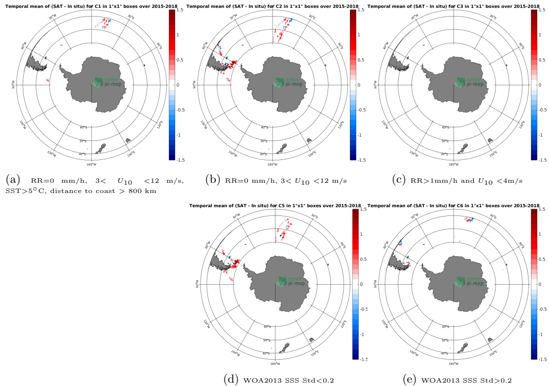
Figure 12: Temporal mean gridded over spatial boxes of size 1^\circ \times 1^\circ of \Delta SSS (SMAP-L3-JPL-V4.3-8DAY-RUNNING-60KM - TSG-POLARSTERN) for 5 different subdatasets corresponding to:RR=0 mm/h, 3 < U_{10} < 12 m/s, SST >5^\circ\text{C} , distance to coast > 800 km (a), RR=0 mm/h, 3 < U_{10} < 12 m/s (b), RR >1 mm/h and U_{10} < 4 m/s (c), WOA2013 SSS Std <0.2 (d), WOA2013 SSS Std >0.2 (e).
