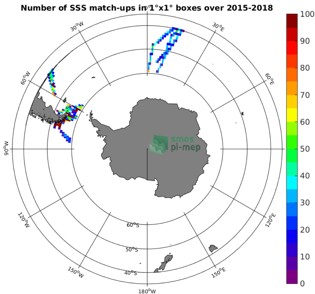
Figure 4: Number of SSS match-ups between TSG-POLARSTERN SSS and the SMAP-L3-JPL-V4.3-8DAY-RUNNING-60KM SSS product for the Roaring Forties and Furious Fifties Pi-MEP region over 1°x1° boxes and for the full satellite product period.
