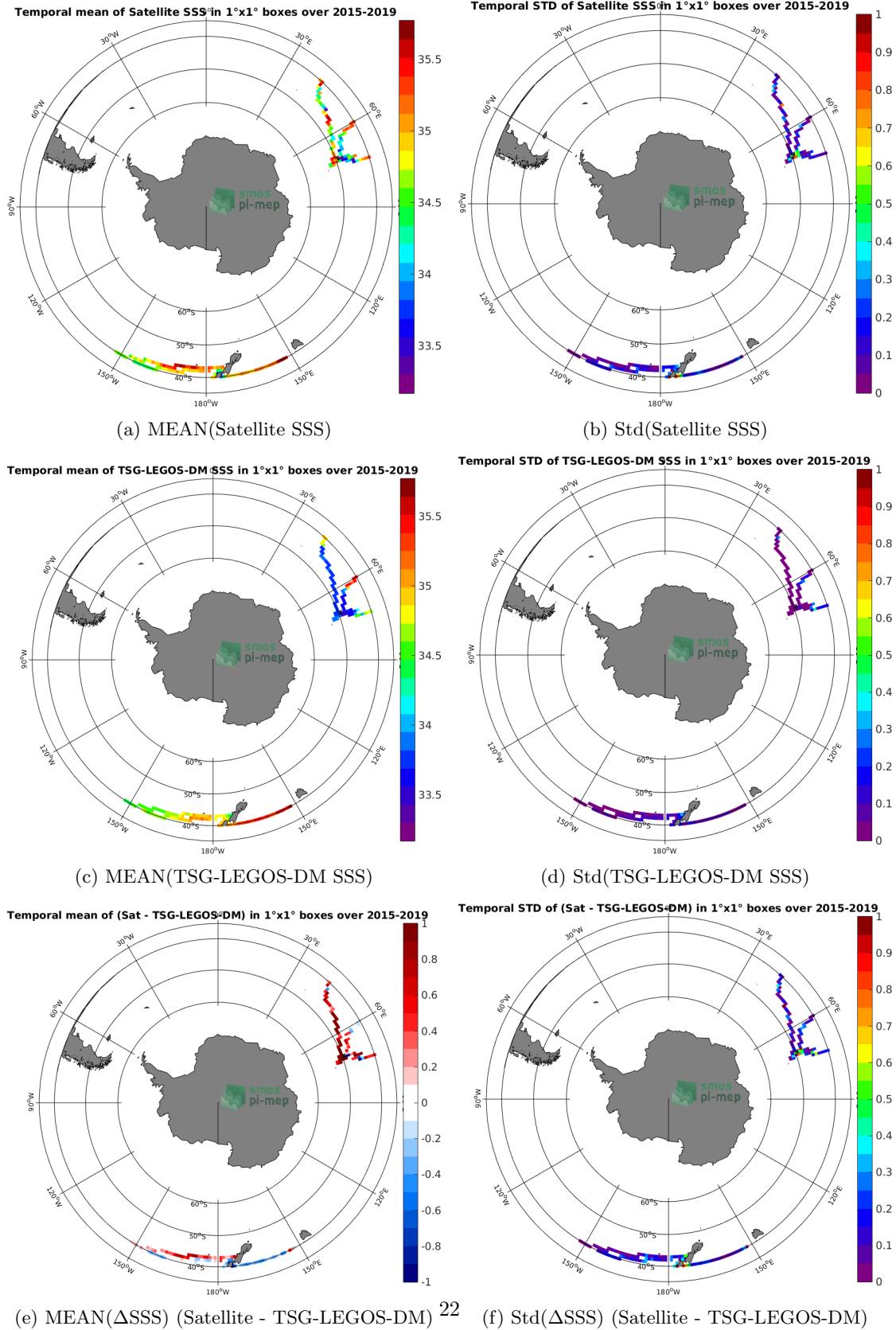
Figure 6: Temporal mean (left) and Std (right) of SSS from SMAP-L3-JPL-V4.3-8DAY-RUNNING-60KM (top), TSG-LEGOS-DM (middle), and of \Delta SSS (Satellite - TSG-LEGOS-DM). Only match-up pairs are used to generate these maps.
