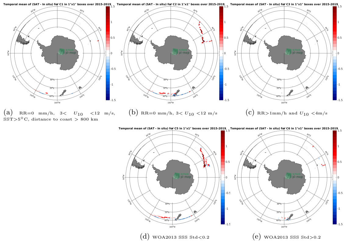
Figure 12: Temporal mean gridded over spatial boxes of size 1^{\circ}\times 1^{\circ} of \Delta\text{SSS} (SMAP-L3-JPL-V4.3-8DAY-RUNNING-60KM - TSG-LEGOS-DM) for 5 different subdatasets corresponding to:RR=0 mm/h, 3 < U_{10} < 12 m/s, SST > 5^{\circ}\text{C} , distance to coast > 800 km (a), RR=0 mm/h, 3 < U_{10} < 12 m/s (b), RR > 1 mm/h and U_{10} < 4 m/s (c), WOA2013 SSS Std < 0.2 (d), WOA2013 SSS Std > 0.2 (e).
