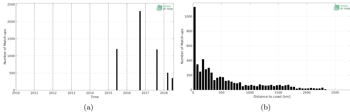
Figure 1: Number of match-ups between TSG-LEGOS-DM and SMAP-L3-JPL-V4.3-8DAY-RUNNING-60KM SSS as a function of time (a) and as function of the distance to coast (b) over the Roaring Forties and Furious Fifties Pi-MEP region and for the full satellite product period.
