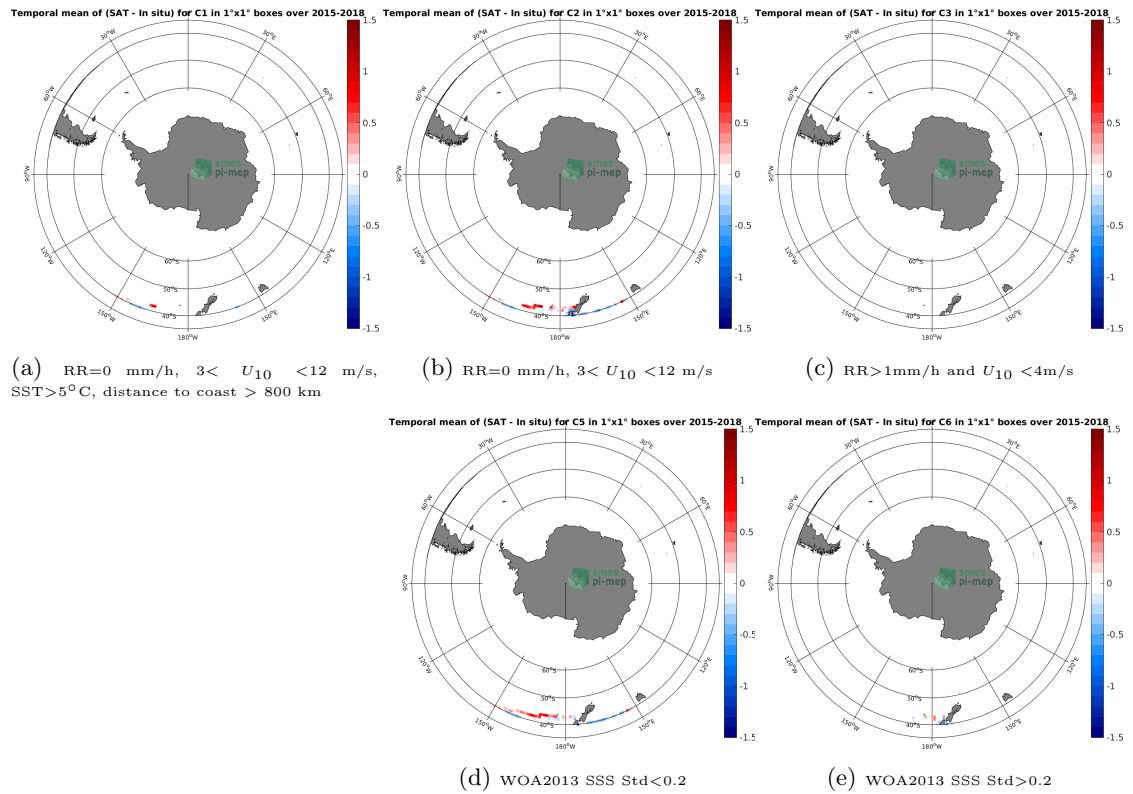
Figure 12: Temporal mean gridded over spatial boxes of size 1^\circ \times 1^\circ of \Delta SSS (SMAP-L3-JPL-V4.3-8DAY-RUNNING-60KM - TSG-LEGOS-DM) for 5 different subdatasets corresponding to:RR=0 mm/h, 3 < U_{10} < 12 m/s, SST>5°C, distance to coast > 800 km (a), RR=0 mm/h, 3 < U_{10} < 12 m/s (b), RR>1mm/h and U_{10} < 4 m/s (c), WOA2013 SSS Std<0.2 (d), WOA2013 SSS Std>0.2 (e).
