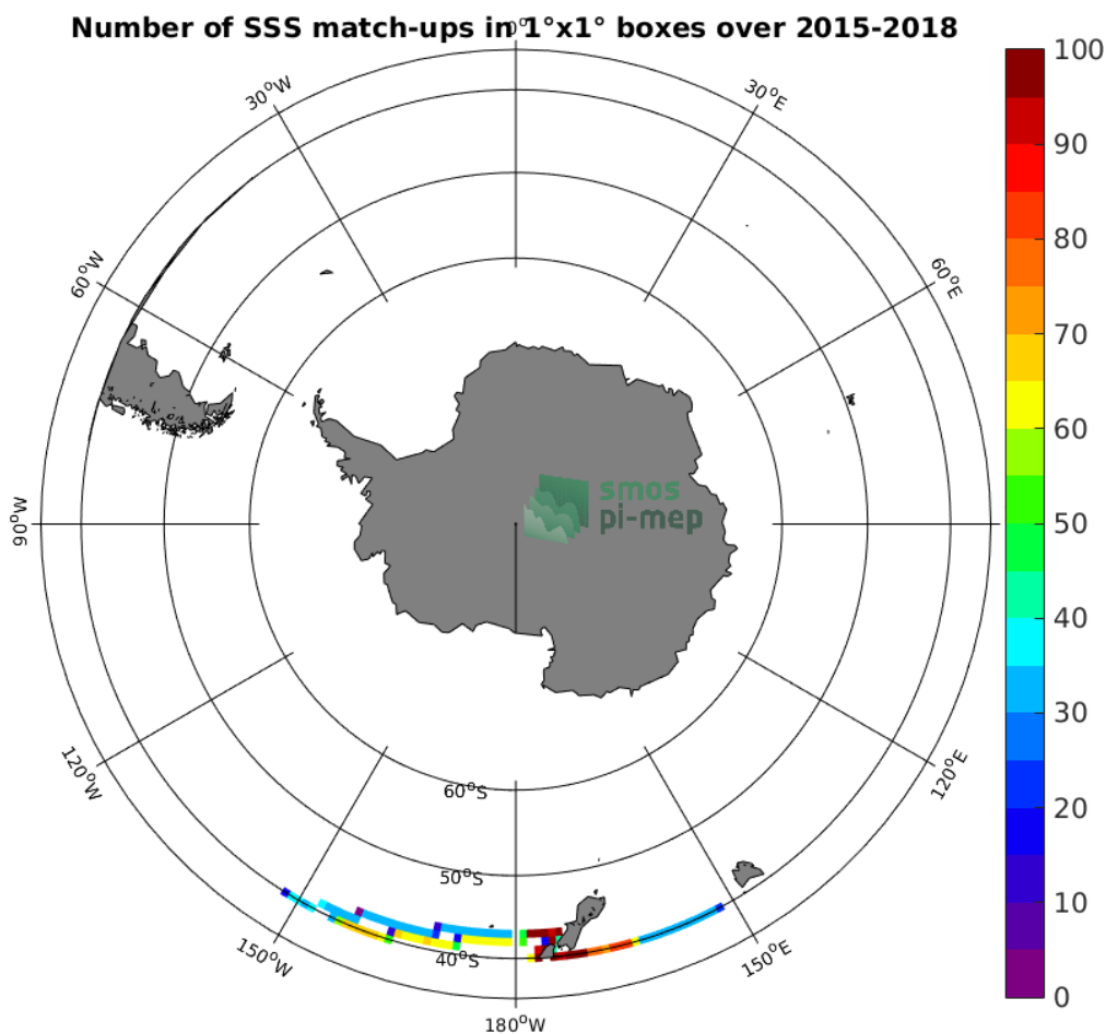
Figure 4: Number of SSS match-ups between TSG-LEGOS-DM SSS and the SMAP-L3-JPL-V4.3-8DAY-RUNNING-60KM SSS product for the Roaring Forties and Furious Fifties Pi-MEP region over 1°x1° boxes and for the full satellite product period.
