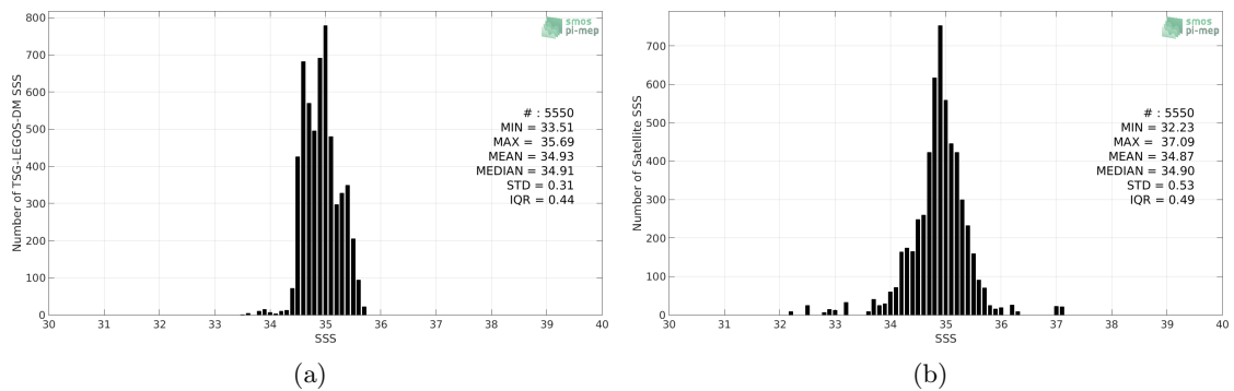
Figure 2: Histograms of SSS from TSG-LEGOS-DM (a) and SMAP-L3-JPL-V4.3-8DAY-RUNNING-60KM (b) considering all match-up pairs per bins of 0.1 over the Roaring Forties and Furious Fifties Pi-MEP region and for the full satellite product period.
