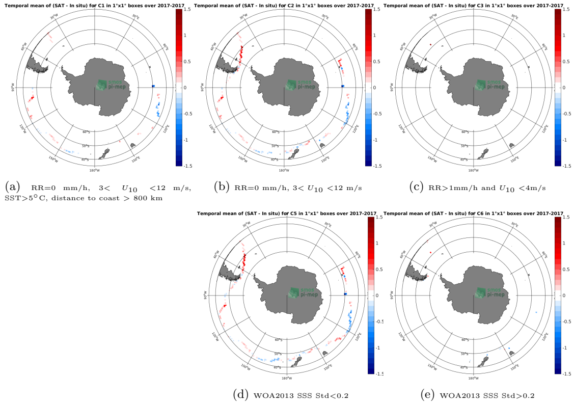
Figure 12: Temporal mean gridded over spatial boxes of size 1°x1° of \Delta SSS (SMAP-L3-JPL-V4.3-8DAY-RUNNING-60KM - TSG-GOSUD-Sailing-ship) for 5 different subdatasets corresponding to:RR=0 mm/h, 3 < U_{10} < 12 m/s, SST>5°C, distance to coast > 800 km (a), RR=0 mm/h, 3 < U_{10} < 12 m/s (b), RR>1mm/h and U_{10} < 4 m/s (c), WOA2013 SSS Std<0.2 (d), WOA2013 SSS Std>0.2 (e).
