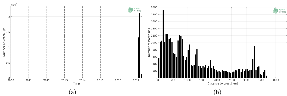
Figure 1: Number of match-ups between TSG-GOSUD-Sailing-ship and SMAP-L3-JPL-V4.3-8DAY-RUNNING-60KM SSS as a function of time (a) and as function of the distance to coast (b) over the Roaring Forties and Furious Fifties Pi-MEP region and for the full satellite product period.
