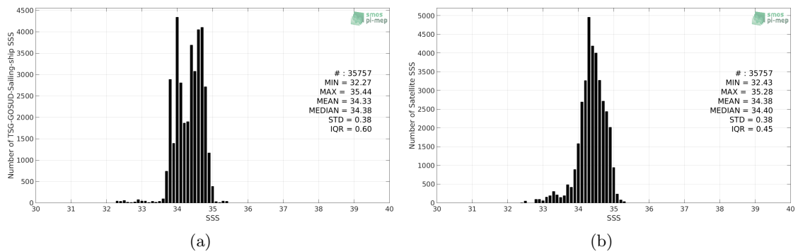
Figure 2: Histograms of SSS from TSG-GOSUD-Sailing-ship (a) and SMAP-L3-JPL-V4.3-8DAY-RUNNING-60KM (b) considering all match-up pairs per bins of 0.1 over the Roaring Forties and Furious Fifties Pi-MEP region and for the full satellite product period.
