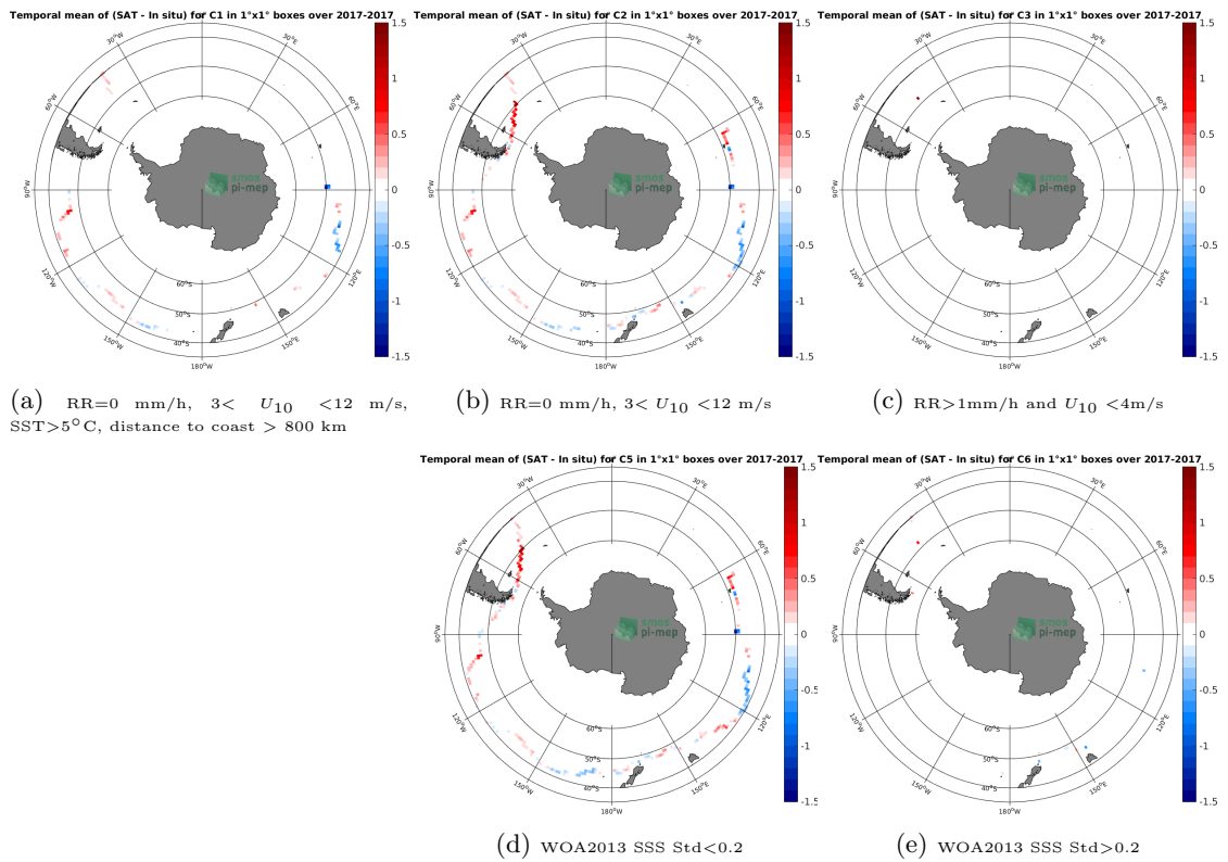
Figure 12: Temporal mean gridded over spatial boxes of size 1^\circ \times 1^\circ of \Delta SSS (SMAP-L3-JPL-V4.3-8DAY-RUNNING-60KM - TSG-GOSUD-Sailing-ship) for 5 different subdatasets corresponding to:RR=0 mm/h, 3 < U_{10} < 12 m/s, SST>5°C, distance to coast > 800 km (a), RR=0 mm/h, 3 < U_{10} < 12 m/s (b), RR>1mm/h and U_{10} < 4 m/s (c), WOA2013 SSS Std<0.2 (d), WOA2013 SSS Std>0.2 (e).
