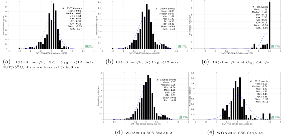
Figure 13: Normalized histogram of \Delta\text{SSS} (SMAP-L3-JPL-V4.3-8DAY-RUNNING-60KM - TSG-GOSUD-Sailing-ship) for 5 different subdatasets corresponding to: RR=0 mm/h, 3 < U_{10} < 12 m/s, SST > 5^\circ\text{C} , distance to coast > 800 km (a), RR=0 mm/h, 3 < U_{10} < 12 m/s (b), RR > 1\text{mm/h} and U_{10} < 4\text{m/s} (c), WOA2013 SSS Std < 0.2 (d), WOA2013 SSS Std > 0.2 (e).
