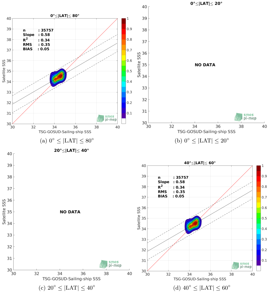
Figure 9: Contour maps of the concentration of SMAP-L3-JPL-V4.3-8DAY-RUNNING-60KM SSS (y-axis) versus TSG-GOSUD-Sailing-ship SSS (x-axis) at match-up pairs for different latitude bands. For each plot, the red line shows x=y . The black thin and dashed lines indicate a linear fit through the data cloud and the \pm 95\% confidence levels, respectively. The number match-up pairs n , the slope and R^2 coefficient of the linear fit, the root mean square (RMS) and the mean bias between satellite and in situ data are indicated for each latitude band in each plots.
