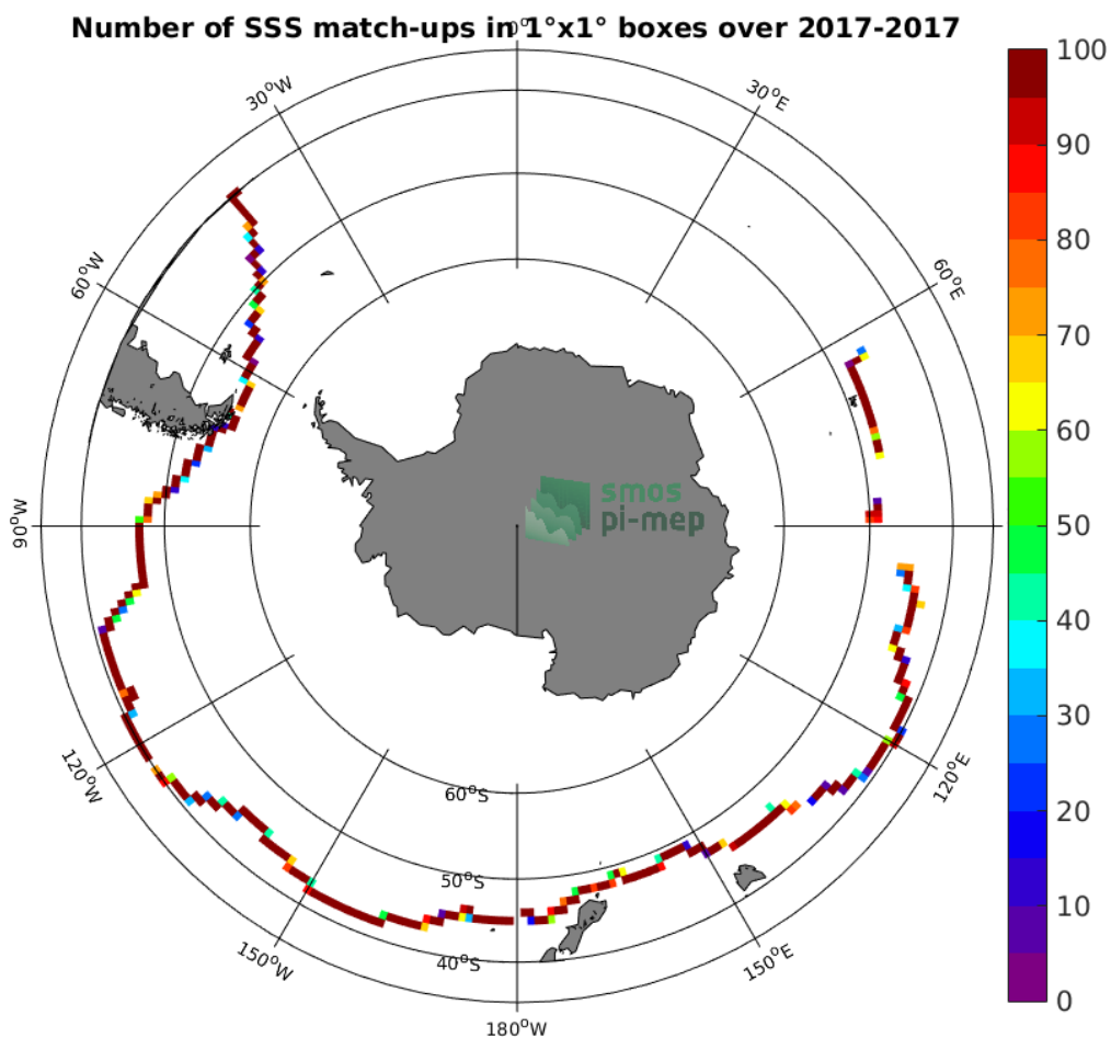
Figure 4: Number of SSS match-ups between TSG-GOSUD-Sailing-ship SSS and the SMAP-L3-JPL-V4.3-8DAY-RUNNING-60KM SSS product for the Roaring Forties and Furious Fifties Pi-MEP region over 1^{\circ} \times 1^{\circ} boxes and for the full satellite product period.
