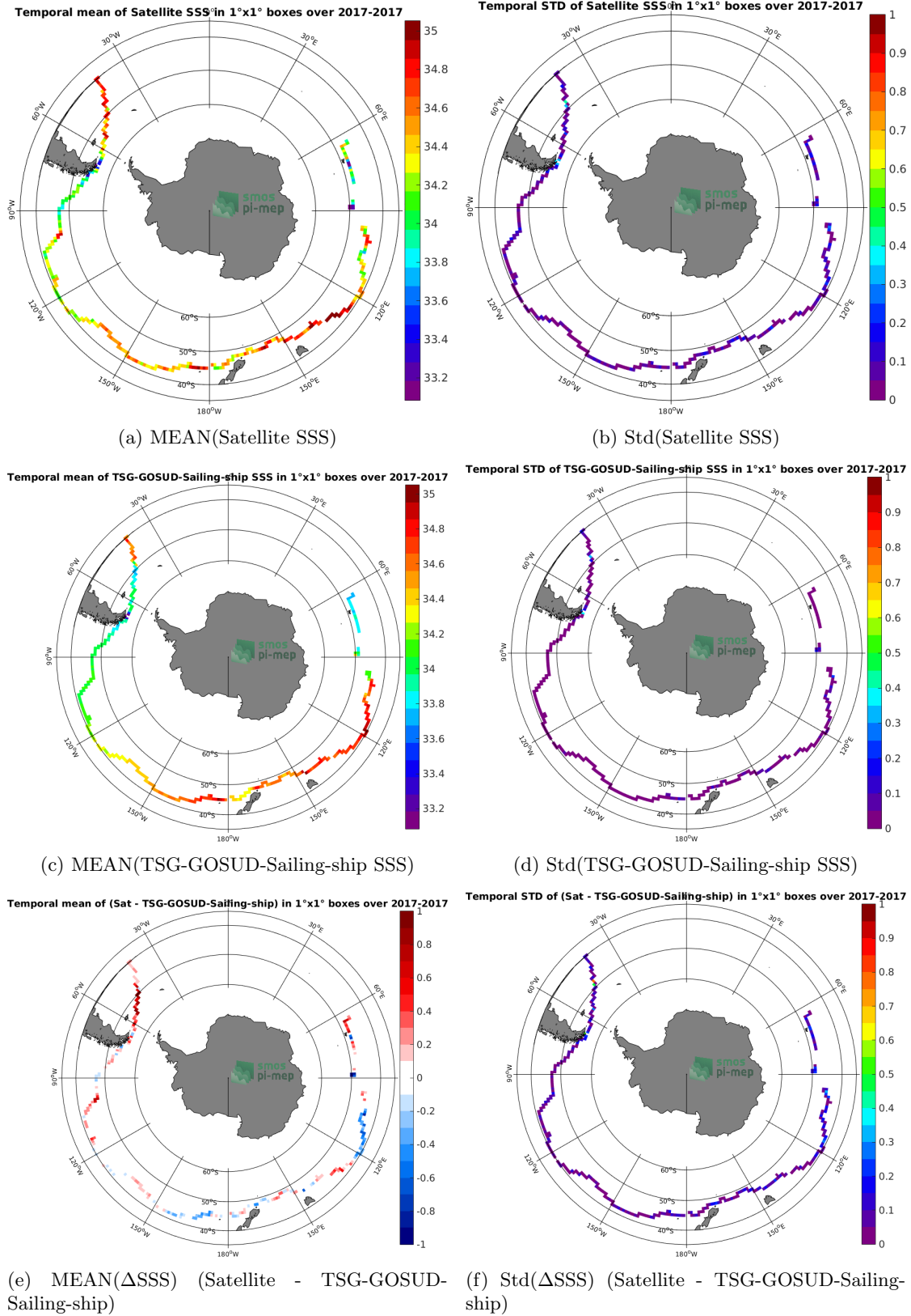
Figure 6: Temporal mean (left) and Std (right) of SSS from SMAP-L3-JPL-V4.3-8DAY-RUNNING-60KM (top), TSG-GOSUD-Sailing-ship (middle), and of \Delta SSS (Satellite - TSG-GOSUD-Sailing-ship). Only match-up pairs are used to generate these maps.
