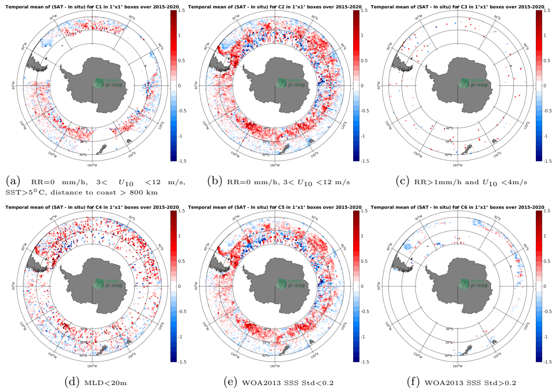
Figure 12: Temporal mean gridded over spatial boxes of size 1^{\circ}\times 1^{\circ} of \Delta\text{SSS} (SMAP-L3-JPL-V4.3-8DAY-RUNNING-60KM - Argo) for 6 different subdatasets corresponding to:RR=0 mm/h, 3 < U_{10} < 12 m/s, SST > 5^{\circ}\text{C} , distance to coast > 800 km (a), RR=0 mm/h, 3 < U_{10} < 12 m/s (b), RR > 1 mm/h and U_{10} < 4 m/s (c),MLD < 20 m (d),WOA2013 SSS Std < 0.2 (e),WOA2013 SSS Std > 0.2 (f).
