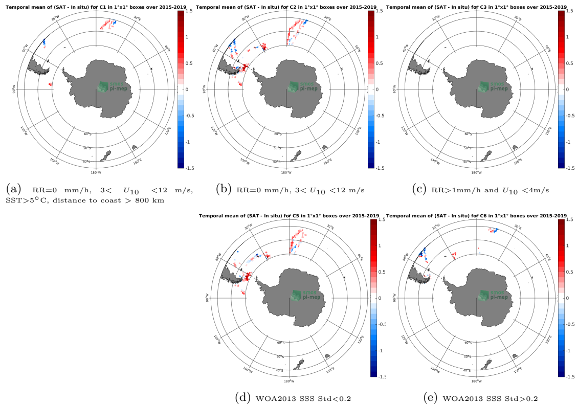
Figure 12: Temporal mean gridded over spatial boxes of size 1^{\circ}\times 1^{\circ} of \Delta\text{SSS} (SMAP-L3-JPL-V4.3-MONTHLY-60KM - TSG-POLARSTERN) for 5 different subdatasets corresponding to:RR=0 mm/h, 3 < U_{10} < 12 m/s, SST >5^{\circ}\text{C} , distance to coast > 800 km (a), RR=0 mm/h, 3 < U_{10} < 12 m/s (b), RR >1 mm/h and U_{10} < 4 m/s (c), WOA2013 SSS Std <0.2 (d), WOA2013 SSS Std >0.2 (e).
