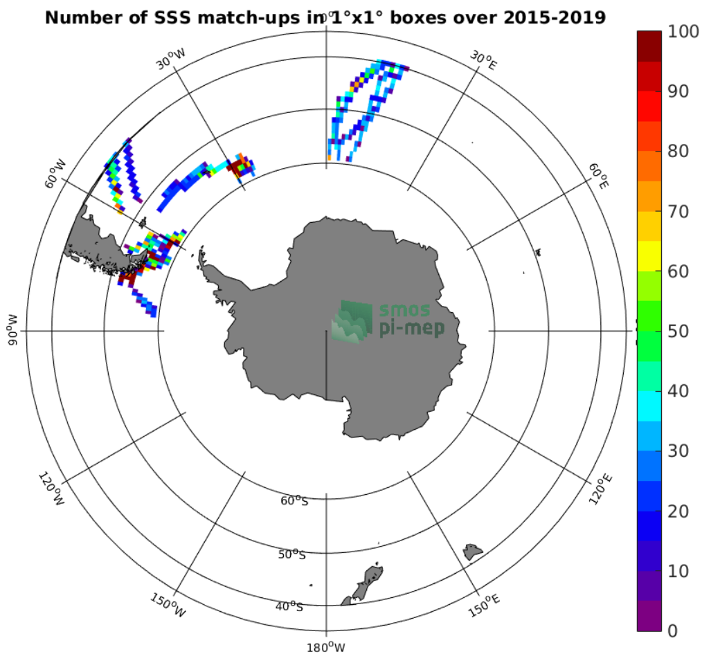
Figure 4: Number of SSS match-ups between TSG-POLARSTERN SSS and the SMAP-L3-JPL-V4.3-MONTHLY-60KM SSS product for the Roaring Forties and Furious Fifties Pi-MEP region over 1^\circ \times 1^\circ boxes and for the full satellite product period.
