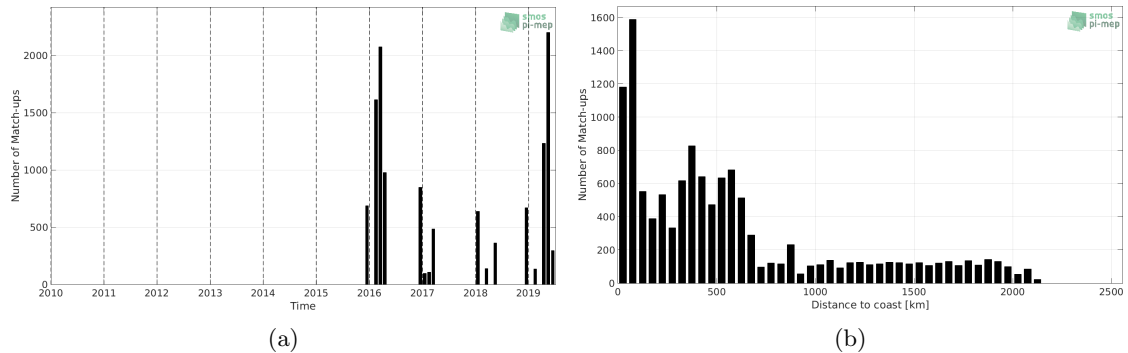
Figure 1: Number of match-ups between TSG-POLARSTERN and SMAP-L3-JPL-V4.3-MONTHLY-60KM SSS as a function of time (a) and as function of the distance to coast (b) over the Roaring Forties and Furious Fifties Pi-MEP region and for the full satellite product period.
