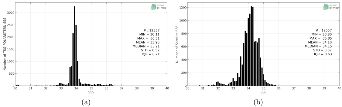
Figure 2: Histograms of SSS from TSG-POLARSTERN (a) and SMAP-L3-JPL-V4.3-MONTHLY-60KM (b) considering all match-up pairs per bins of 0.1 over the Roaring Forties and Furious Fifties Pi-MEP region and for the full satellite product period.
