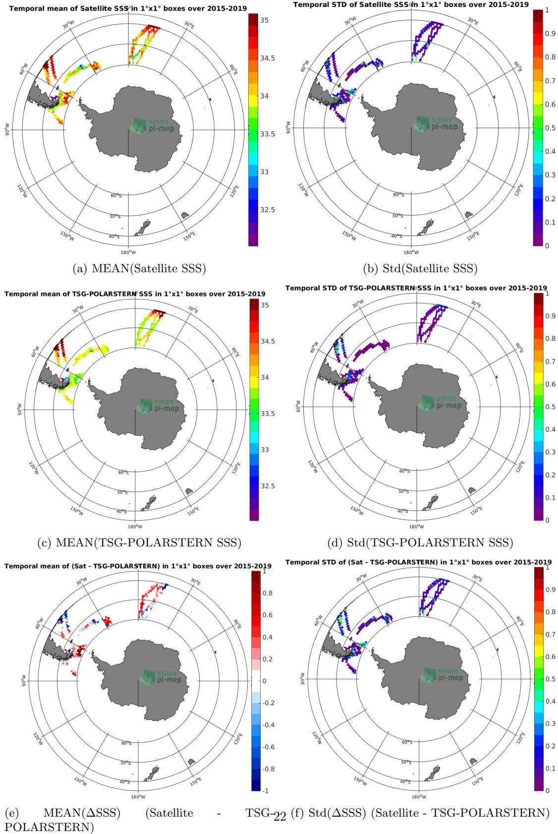
Figure 6: Temporal mean (left) and Std (right) of SSS from SMAP-L3-JPL-V4.3-MONTHLY-60KM (top), TSG-POLARSTERN (middle), and of \Delta SSS (Satellite - TSG-POLARSTERN). Only match-up pairs are used to generate these maps.
