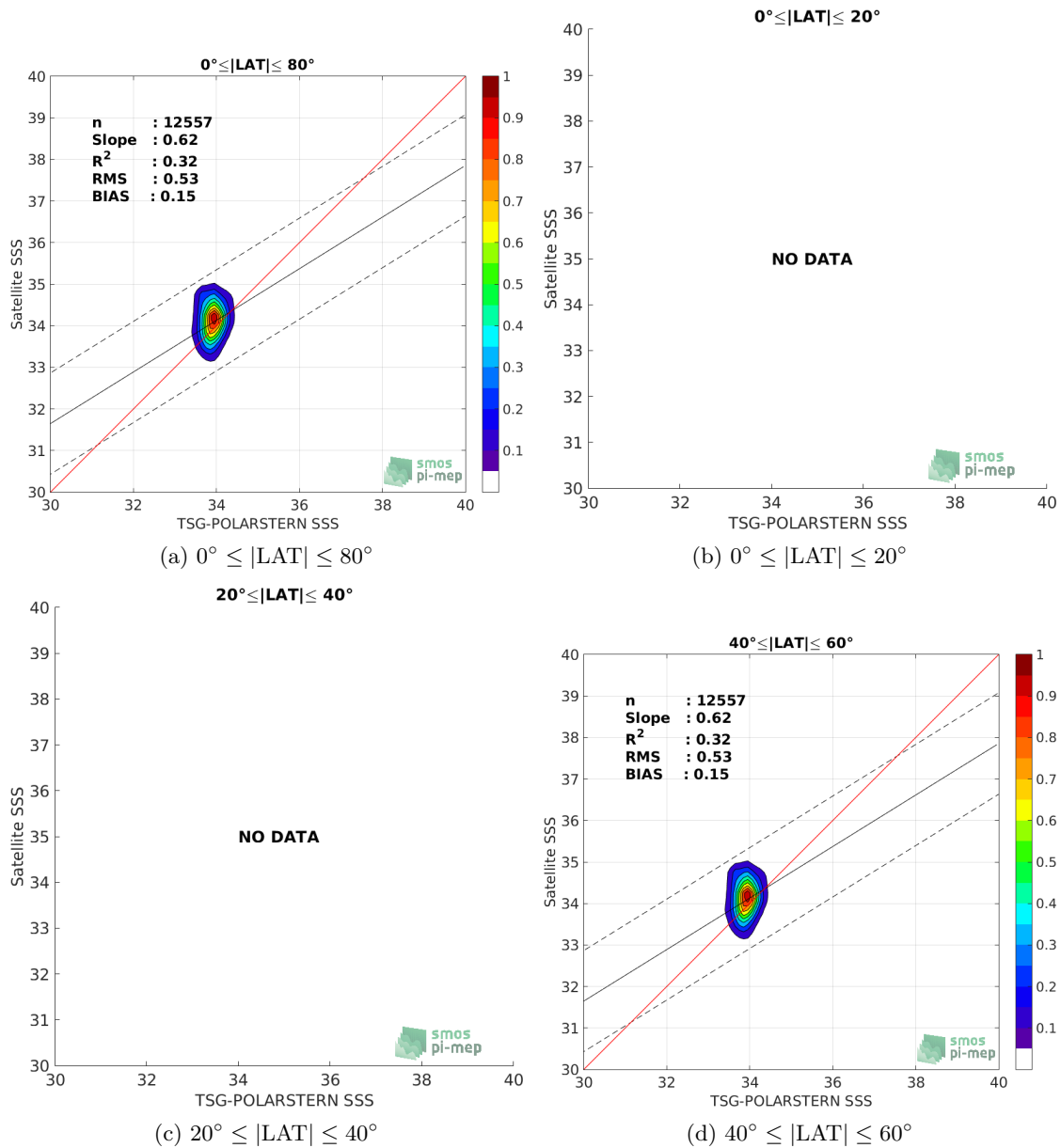
Figure 9: Contour maps of the concentration of SMAP-L3-JPL-V4.3-MONTHLY-60KM SSS (y-axis) versus TSG-POLARSTERN SSS (x-axis) at match-up pairs for different latitude bands. For each plot, the red line shows x=y . The black thin and dashed lines indicate a linear fit through the data cloud and the \pm 95\% confidence levels, respectively. The number match-up pairs n , the slope and R^2 coefficient of the linear fit, the root mean square (RMS) and the mean bias between satellite and in situ data are indicated for each latitude band in each plots.
