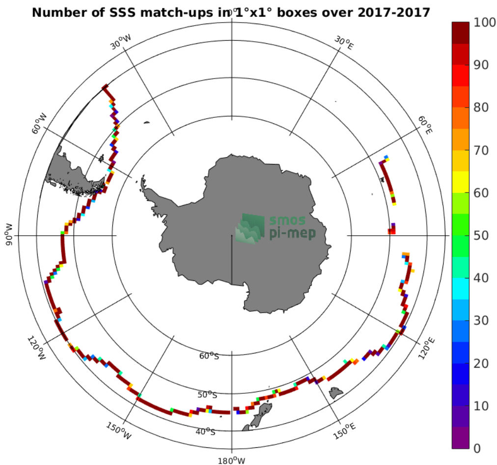
Figure 4: Number of SSS match-ups between TSG-GOSUD-Sailing-ship SSS and the SMAP-L3-JPL-V4.3-MONTHLY-60KM SSS product for the Roaring Forties and Furious Fifties Pi-MEP region over 1°x1° boxes and for the full satellite product period.
