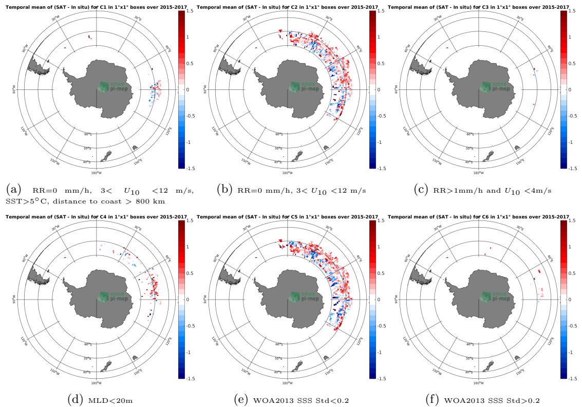
Figure 12: Temporal mean gridded over spatial boxes of size 1^{\circ}\times 1^{\circ} of \Delta\text{SSS} (SMAP-L3-JPL-V4.3-MONTHLY-60KM - Sea mammals) for 6 different subdatasets corresponding to:RR=0 mm/h, 3 < U_{10} < 12 m/s, SST >5^{\circ}\text{C} , distance to coast > 800 km (a), RR=0 mm/h, 3 < U_{10} < 12 m/s (b), RR >1 mm/h and U_{10} < 4 m/s (c),MLD <20 m (d),WOA2013 SSS Std <0.2 (e),WOA2013 SSS Std >0.2 (f).
