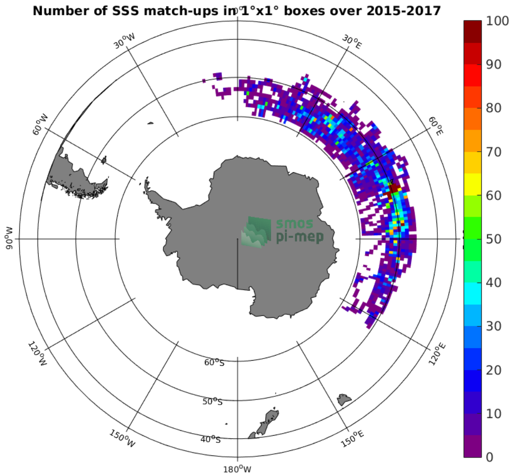
Figure 4: Number of SSS match-ups between Sea mammals SSS and the SMAP-L3-JPL-V4.3-MONTHLY-60KM SSS product for the Roaring Forties and Furious Fifties Pi-MEP region over 1°x1° boxes and for the full satellite product period.
