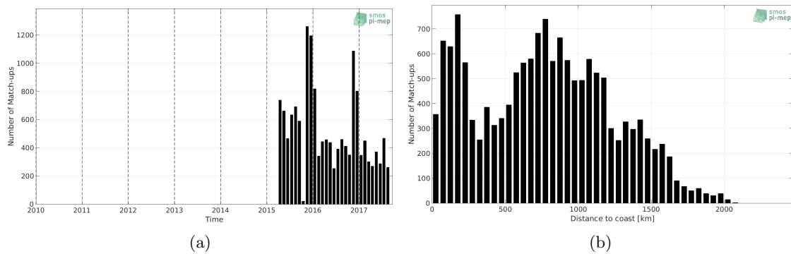
Figure 1: Number of match-ups between Sea mammals and SMAP-L3-JPL-V4.3-MONTHLY-60KM SSS as a function of time (a) and as function of the distance to coast (b) over the Roaring Forties and Furious Fifties Pi-MEP region and for the full satellite product period.
