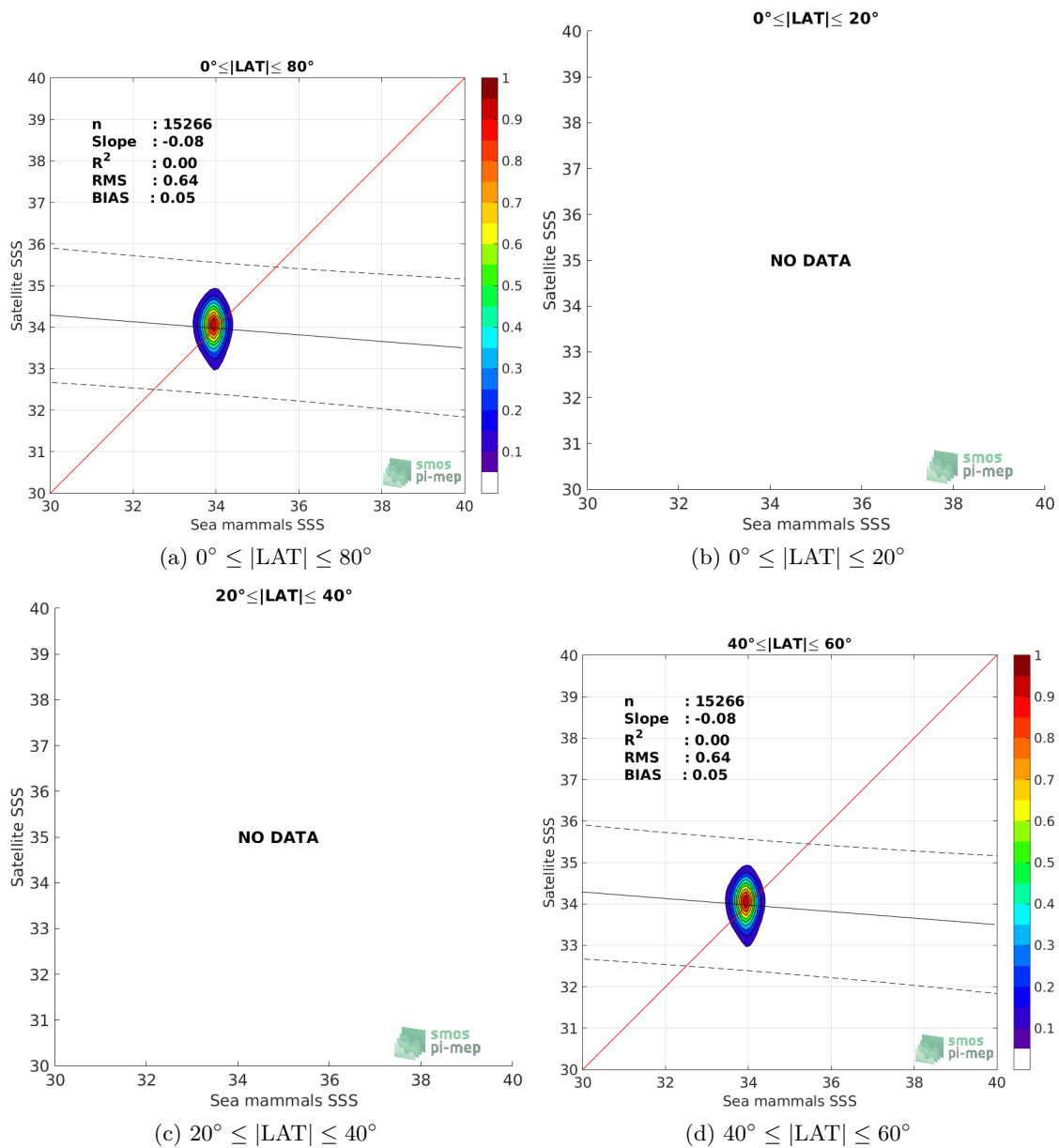
Figure 9: Contour maps of the concentration of SMAP-L3-JPL-V4.3-MONTHLY-60KM SSS (y-axis) versus Sea mammals SSS (x-axis) at match-up pairs for different latitude bands. For each plot, the red line shows x=y . The black thin and dashed lines indicate a linear fit through the data cloud and the \pm 95\% confidence levels, respectively. The number match-up pairs n , the slope and R^2 coefficient of the linear fit, the root mean square (RMS) and the mean bias between satellite and in situ data are indicated for each latitude band in each plots.
