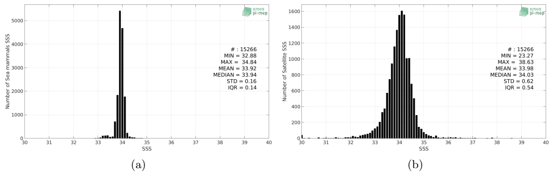
Figure 2: Histograms of SSS from Sea mammals (a) and SMAP-L3-JPL-V4.3-MONTHLY-60KM (b) considering all match-up pairs per bins of 0.1 over the Roaring Forties and Furious Fifties Pi-MEP region and for the full satellite product period.
