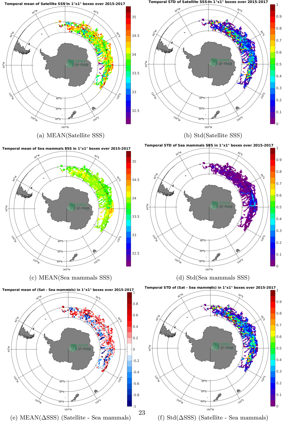
Figure 6: Temporal mean (left) and Std (right) of SSS from SMAP-L3-JPL-V4.3-MONTHLY-60KM (top), Sea mammals (middle), and of \Delta SSS (Satellite - Sea mammals). Only match-up pairs are used to generate these maps.
