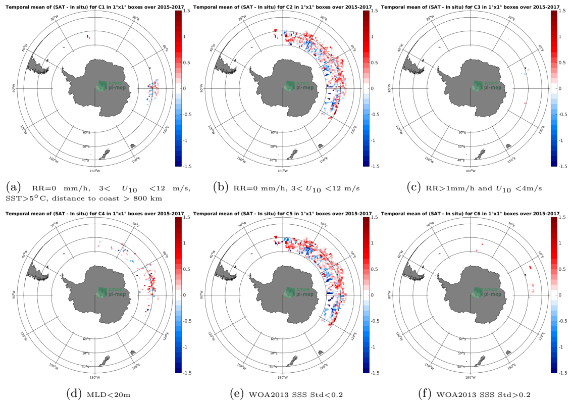
Figure 12: Temporal mean gridded over spatial boxes of size 1^\circ \times 1^\circ of \Delta SSS (SMAP-L3-JPL-V4.3-MONTHLY-60KM - Sea mammals) for 6 different subdatasets corresponding to:RR=0 mm/h, 3 < U_{10} < 12 m/s, SST > 5^\circ\text{C} , distance to coast > 800 km (a), RR=0 mm/h, 3 < U_{10} < 12 m/s (b), RR > 1 mm/h and U_{10} < 4 m/s (c),MLD < 20 m (d),WOA2013 SSS Std < 0.2 (e),WOA2013 SSS Std > 0.2 (f).
