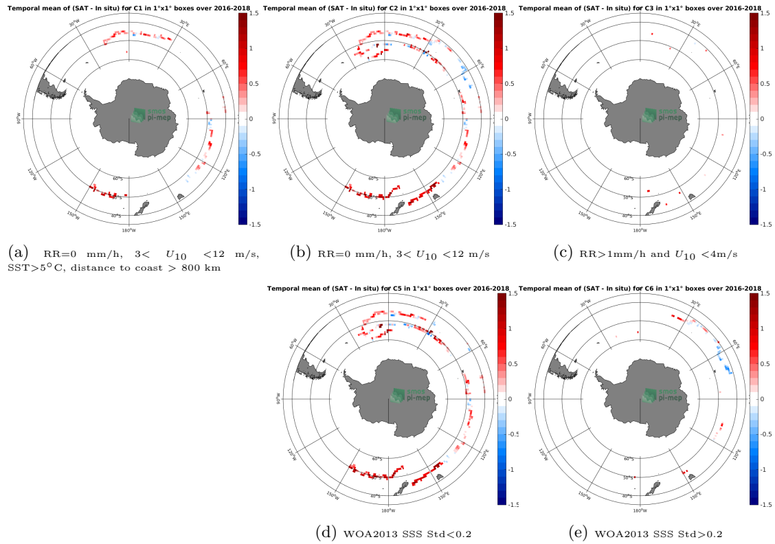
Figure 11: Temporal mean gridded over spatial boxes of size 1^{\circ}\times 1^{\circ} of \Delta\text{SSS} (SMAP-L3-JPL-V4.3-MONTHLY-60KM - Surface drifters) for 5 different subdatasets corresponding to:RR=0 mm/h, 3 < U_{10} < 12 m/s, SST >5^{\circ}\text{C} , distance to coast > 800 km (a), RR=0 mm/h, 3 < U_{10} < 12 m/s (b), RR >1 mm/h and U_{10} < 4 m/s (c), WOA2013 SSS Std <0.2 (d), WOA2013 SSS Std >0.2 (e).
