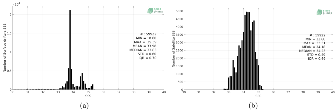
Figure 2: Histograms of SSS from Surface drifters (a) and SMAP-L3-JPL-V4.3-MONTHLY-60KM (b) considering all match-up pairs per bins of 0.1 over the Roaring Forties and Furious Fifties Pi-MEP region and for the full satellite product period.
