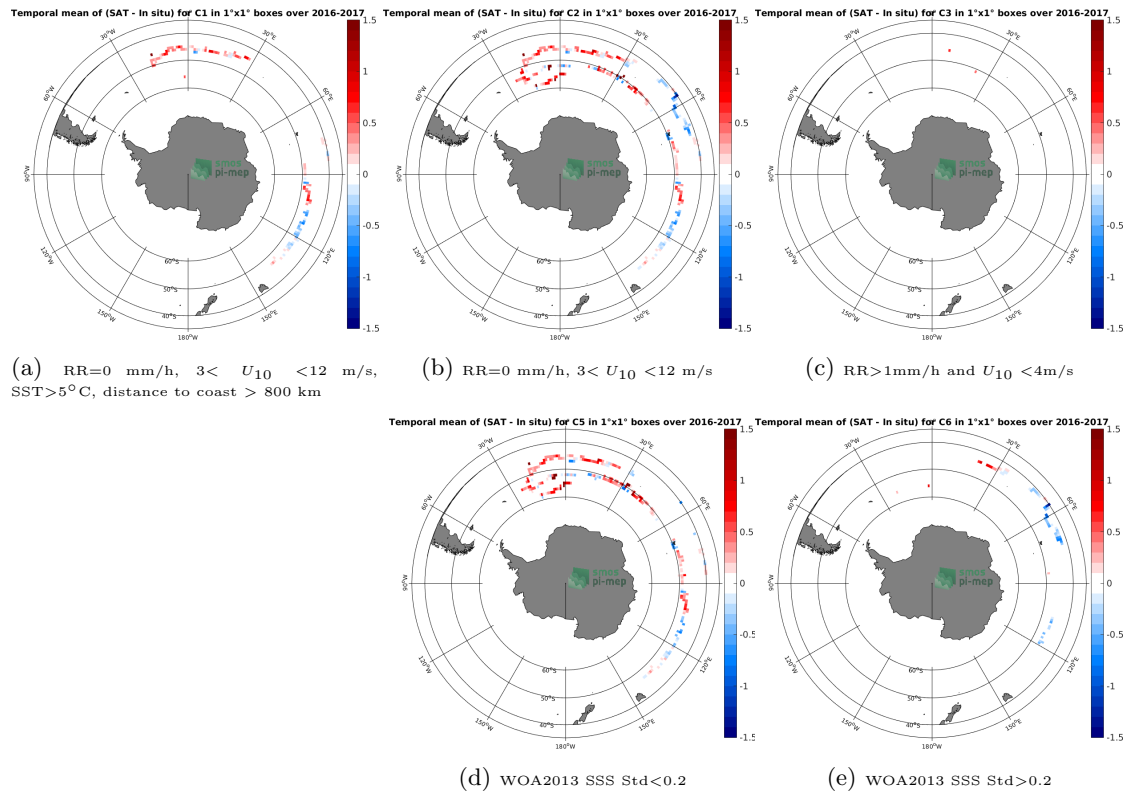
Figure 11: Temporal mean gridded over spatial boxes of size 1^\circ \times 1^\circ of \Delta SSS (SMAP-L3-JPL-V4.3-MONTHLY-60KM - Surface drifters) for 5 different subdatasets corresponding to:RR=0 mm/h, 3 < U_{10} < 12 m/s, SST >5^\circ C, distance to coast > 800 km (a), RR=0 mm/h, 3 < U_{10} < 12 m/s (b), RR >1 mm/h and U_{10} < 4 m/s (c), WOA2013 SSS Std <0.2 (d), WOA2013 SSS Std >0.2 (e).
