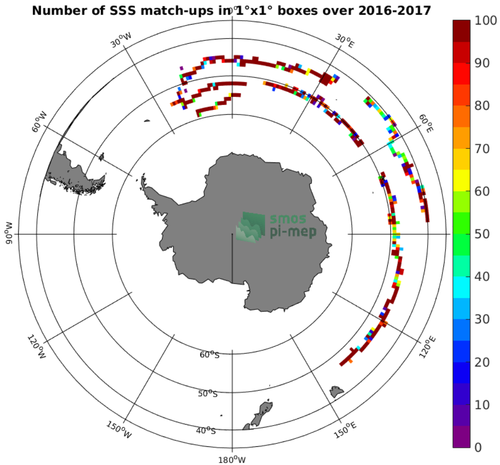
Figure 3: Number of SSS match-ups between Surface drifters SSS and the SMAP-L3-JPL-V4.3-MONTHLY-60KM SSS product for the Roaring Forties and Furious Fifties Pi-MEP region over 1^\circ \times 1^\circ boxes and for the full satellite product period.
