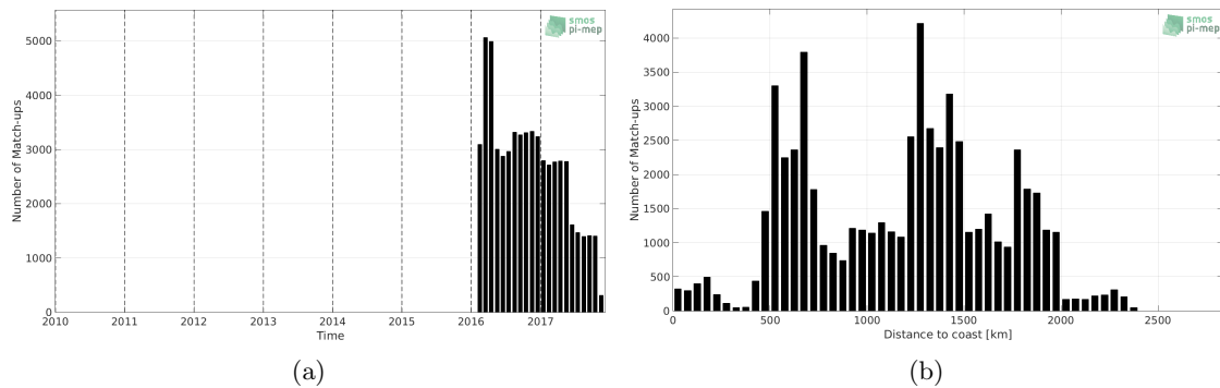
Figure 1: Number of match-ups between Surface drifters and SMAP-L3-JPL-V4.3-MONTHLY-60KM SSS as a function of time (a) and as function of the distance to coast (b) over the Roaring Forties and Furious Fifties Pi-MEP region and for the full satellite product period.
