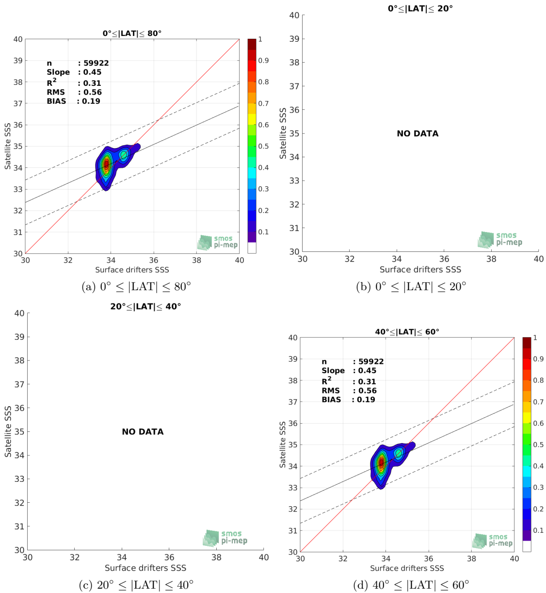
Figure 8: Contour maps of the concentration of SMAP-L3-JPL-V4.3-MONTHLY-60KM SSS (y-axis) versus Surface drifters SSS (x-axis) at match-up pairs for different latitude bands. For each plot, the red line shows x=y . The black thin and dashed lines indicate a linear fit through the data cloud and the \pm 95\% confidence levels, respectively. The number match-up pairs n , the slope and R^2 coefficient of the linear fit, the root mean square (RMS) and the mean bias between satellite and in situ data are indicated for each latitude band in each plots.
