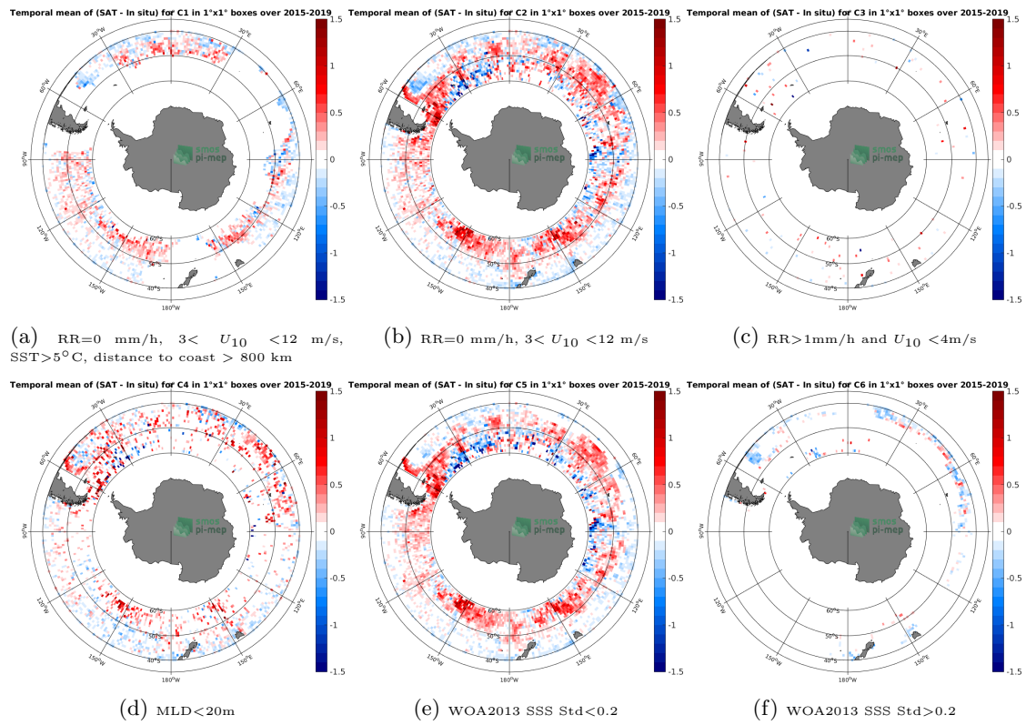
Figure 12: Temporal mean gridded over spatial boxes of size 1^\circ \times 1^\circ of \Delta SSS (SMAP-L3-JPL-V4.3-MONTHLY-60KM - Argo) for 6 different subdatasets corresponding to:RR=0 mm/h, 3 < U_{10} < 12 m/s, SST >5^\circ C, distance to coast > 800 km (a), RR=0 mm/h, 3 < U_{10} < 12 m/s (b), RR >1 mm/h and U_{10} < 4 m/s (c),MLD <20 m (d),WOA2013 SSS Std <0.2 (e),WOA2013 SSS Std >0.2 (f).
