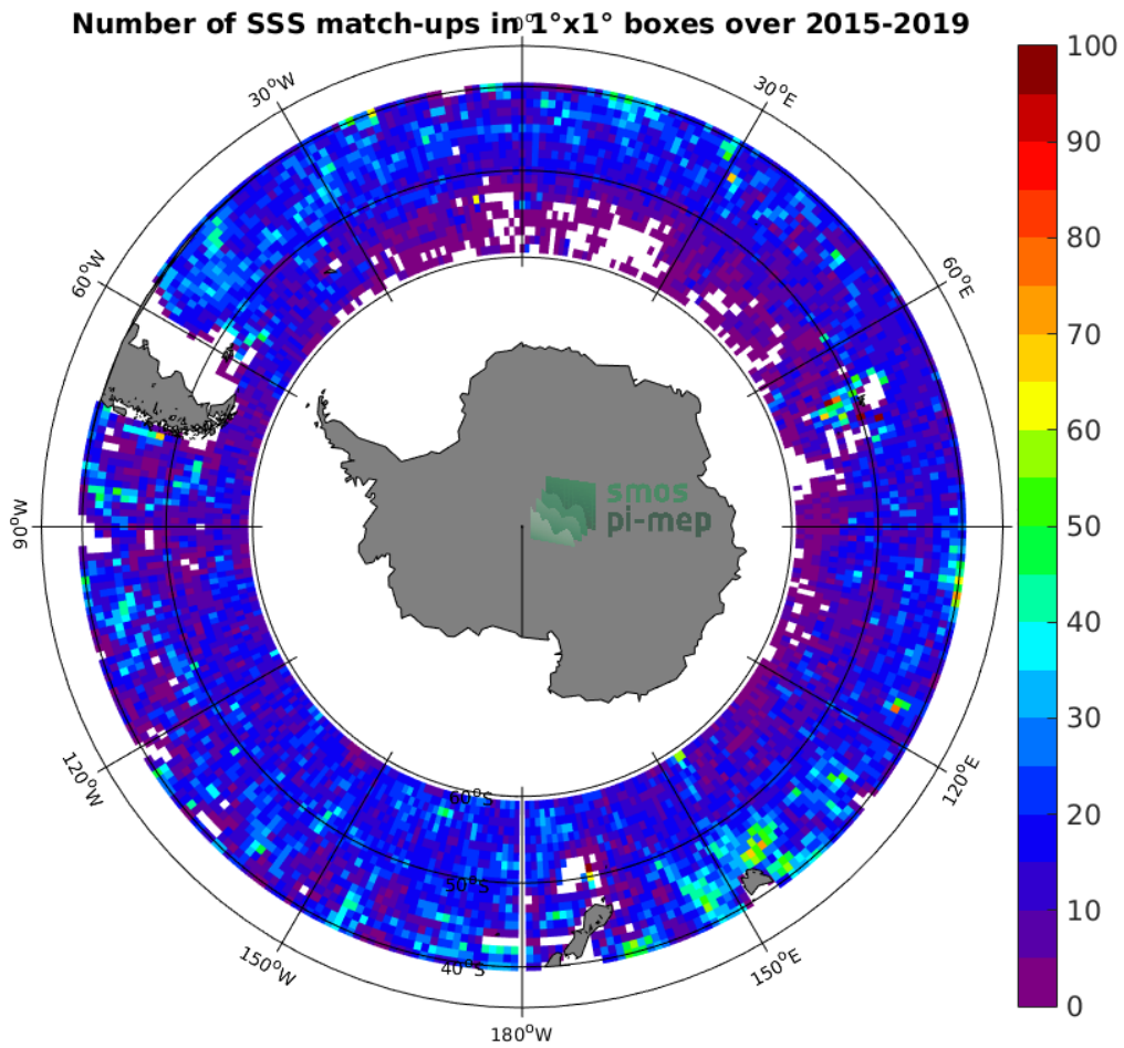
Figure 4: Number of SSS match-ups between Argo SSS and the SMAP-L3-JPL-V4.3-MONTHLY-60KM SSS product for the Roaring Forties and Furious Fifties Pi-MEP region over 1°x1° boxes and for the full satellite product period.
