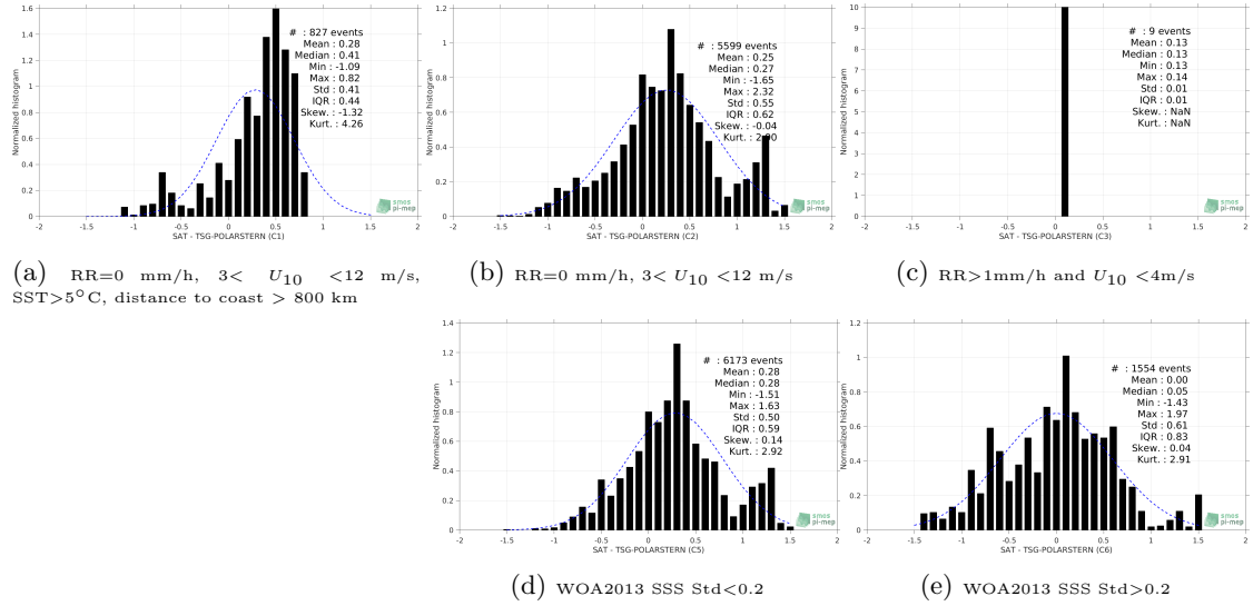
Figure 13: Normalized histogram of \Delta SSS (SMAP-L3-JPL-V4.2-MONTHLY-60KM - TSG-POLARSTERN) for 5 different subdatasets corresponding to: RR=0 mm/h, 3 < U_{10} < 12 m/s, SST > 5°C, distance to coast > 800 km (a), RR=0 mm/h, 3 < U_{10} < 12 m/s (b), RR > 1mm/h and U_{10} < 4 m/s (c), WOA2013 SSS Std < 0.2 (d), WOA2013 SSS Std > 0.2 (e).
