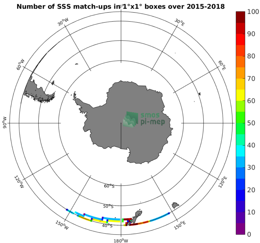
Figure 4: Number of SSS match-ups between TSG-LEGOS-DM SSS and the SMAP-L3-JPL-V4.2-MONTHLY-60KM SSS product for the Roaring Forties and Furious Fifties Pi-MEP region over 1^\circ \times 1^\circ boxes and for the full satellite product period.
