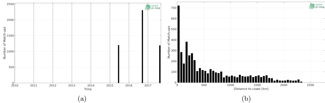
Figure 1: Number of match-ups between TSG-LEGOS-DM and SMAP-L3-JPL-V4.2-MONTHLY-60KM SSS as a function of time (a) and as function of the distance to coast (b) over the Roaring Forties and Furious Fifties Pi-MEP region and for the full satellite product period.
