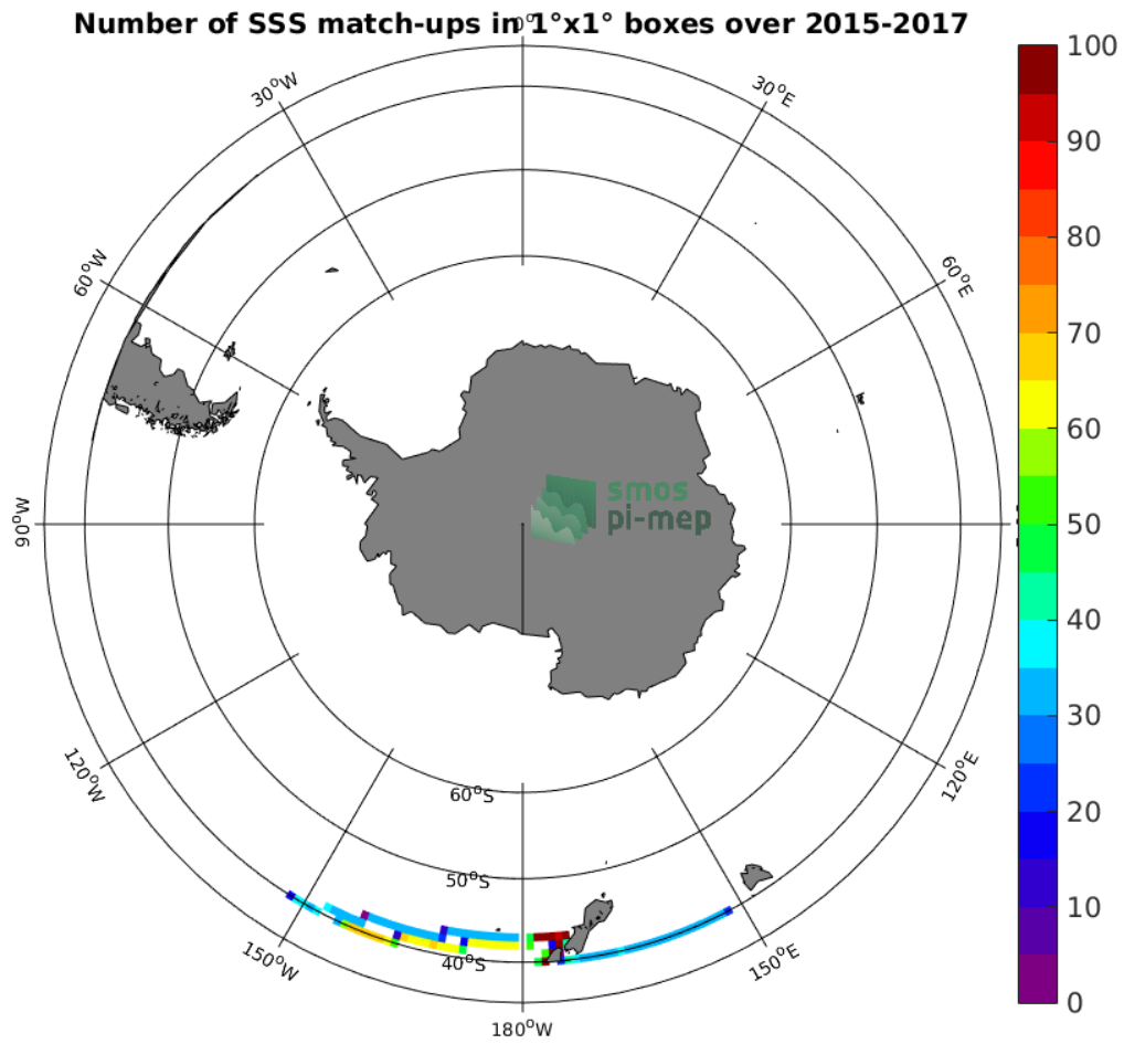
Figure 4: Number of SSS match-ups between TSG-LEGOS-DM SSS and the SMAP-L3-JPL-V4.2-MONTHLY-60KM SSS product for the Roaring Forties and Furious Fifties Pi-MEP region over 1°x1° boxes and for the full satellite product period.
