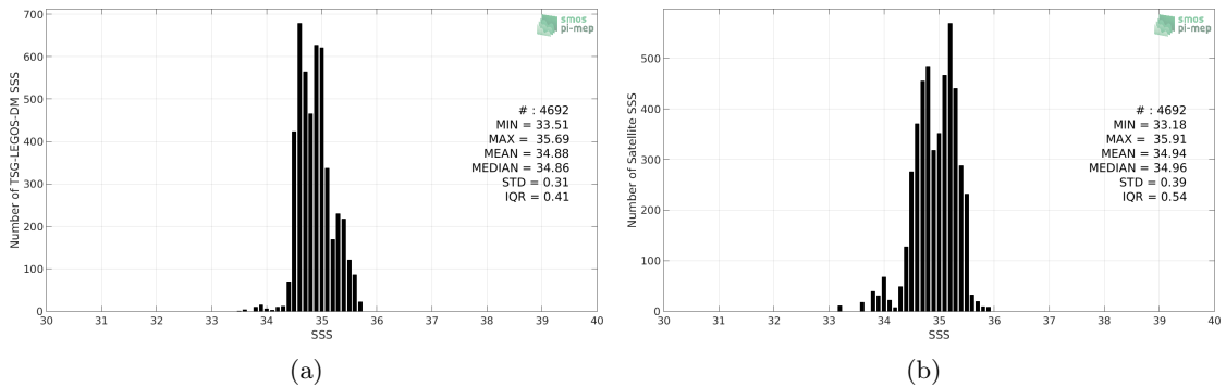
Figure 2: Histograms of SSS from TSG-LEGOS-DM (a) and SMAP-L3-JPL-V4.2-MONTHLY-60KM (b) considering all match-up pairs per bins of 0.1 over the Roaring Forties and Furious Fifties Pi-MEP region and for the full satellite product period.
