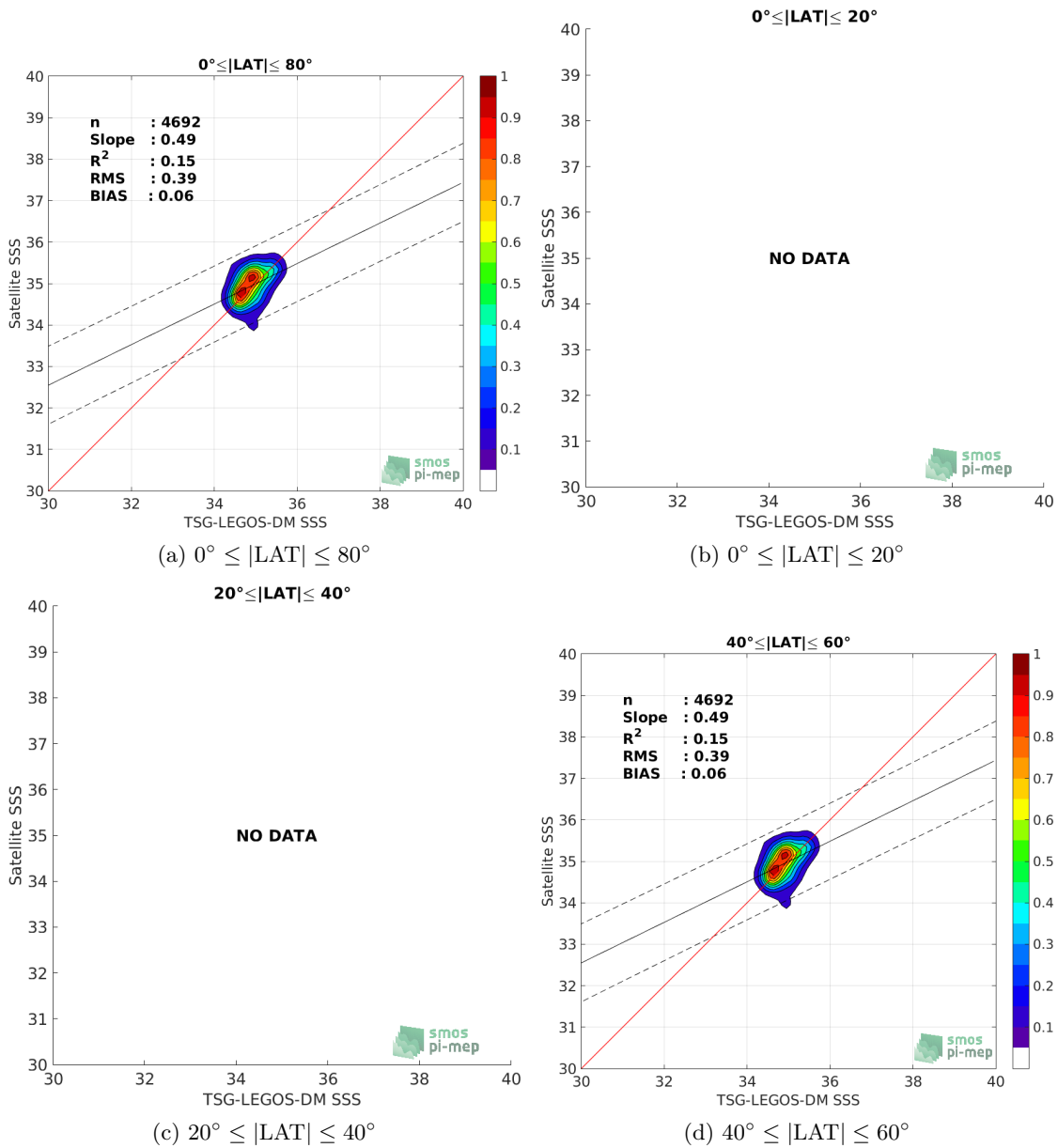
Figure 9: Contour maps of the concentration of SMAP-L3-JPL-V4.2-MONTHLY-60KM SSS (y-axis) versus TSG-LEGOS-DM SSS (x-axis) at match-up pairs for different latitude bands. For each plot, the red line shows x=y . The black thin and dashed lines indicate a linear fit through the data cloud and the \pm 95\% confidence levels, respectively. The number match-up pairs n , the slope and R^2 coefficient of the linear fit, the root mean square (RMS) and the mean bias between satellite and in situ data are indicated for each latitude band in each plots.
