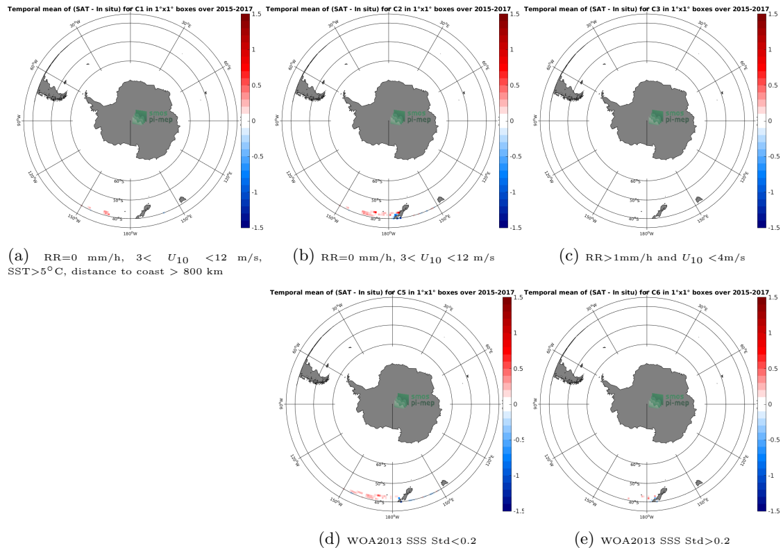
Figure 12: Temporal mean gridded over spatial boxes of size 1^\circ \times 1^\circ of \Delta SSS (SMAP-L3-JPL-V4.2-MONTHLY-60KM - TSG-LEGOS-DM) for 5 different subdatasets corresponding to:RR=0 mm/h, 3 < U_{10} < 12 m/s, SST >5^\circ C, distance to coast > 800 km (a), RR=0 mm/h, 3 < U_{10} < 12 m/s (b), RR >1 mm/h and U_{10} < 4 m/s (c), WOA2013 SSS Std <0.2 (d), WOA2013 SSS Std >0.2 (e).
