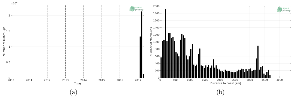
Figure 1: Number of match-ups between TSG-GOSUD-Sailing-ship and SMAP-L3-JPL-V4.2-MONTHLY-60KM SSS as a function of time (a) and as function of the distance to coast (b) over the Roaring Forties and Furious Fifties Pi-MEP region and for the full satellite product period.
