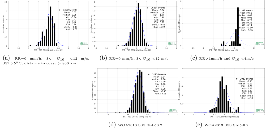
Figure 13: Normalized histogram of \Delta\text{SSS} (SMAP-L3-JPL-V4.2-MONTHLY-60KM - TSG-GOSUD-Sailing-ship) for 5 different subdatasets corresponding to: RR=0 mm/h, 3 < U_{10} < 12 m/s, SST > 5^\circ\text{C} , distance to coast > 800 km (a), RR=0 mm/h, 3 < U_{10} < 12 m/s (b), RR > 1\text{mm/h} and U_{10} < 4\text{m/s} (c), WOA2013 SSS Std < 0.2 (d), WOA2013 SSS Std > 0.2 (e).
