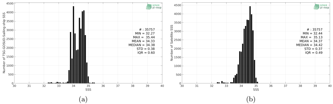
Figure 2: Histograms of SSS from TSG-GOSUD-Sailing-ship (a) and SMAP-L3-JPL-V4.2-MONTHLY-60KM (b) considering all match-up pairs per bins of 0.1 over the Roaring Forties and Furious Fifties Pi-MEP region and for the full satellite product period.
