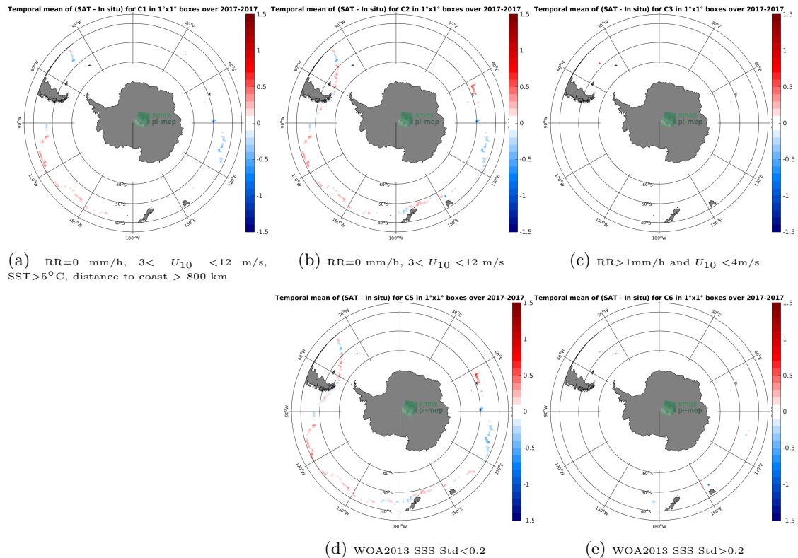
Figure 12: Temporal mean gridded over spatial boxes of size 1^\circ \times 1^\circ of \Delta SSS (SMAP-L3-JPL-V4.2-MONTHLY-60KM - TSG-GOSUD-Sailing-ship) for 5 different subdatasets corresponding to:RR=0 mm/h, 3 < U_{10} < 12 m/s, SST >5^\circ C, distance to coast > 800 km (a), RR=0 mm/h, 3 < U_{10} < 12 m/s (b), RR >1 mm/h and U_{10} < 4 m/s (c), WOA2013 SSS Std <0.2 (d), WOA2013 SSS Std >0.2 (e).
