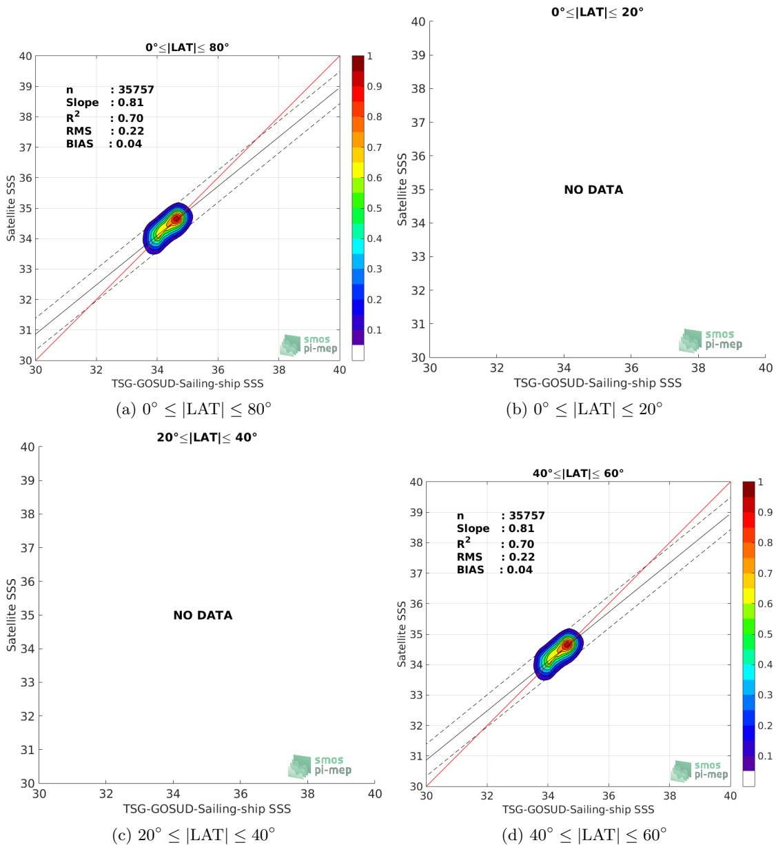
Figure 9: Contour maps of the concentration of SMAP-L3-JPL-V4.2-MONTHLY-60KM SSS (y-axis) versus TSG-GOSUD-Sailing-ship SSS (x-axis) at match-up pairs for different latitude bands. For each plot, the red line shows x=y . The black thin and dashed lines indicate a linear fit through the data cloud and the \pm 95\% confidence levels, respectively. The number match-up pairs n , the slope and R^2 coefficient of the linear fit, the root mean square (RMS) and the mean bias between satellite and in situ data are indicated for each latitude band in each plots.
