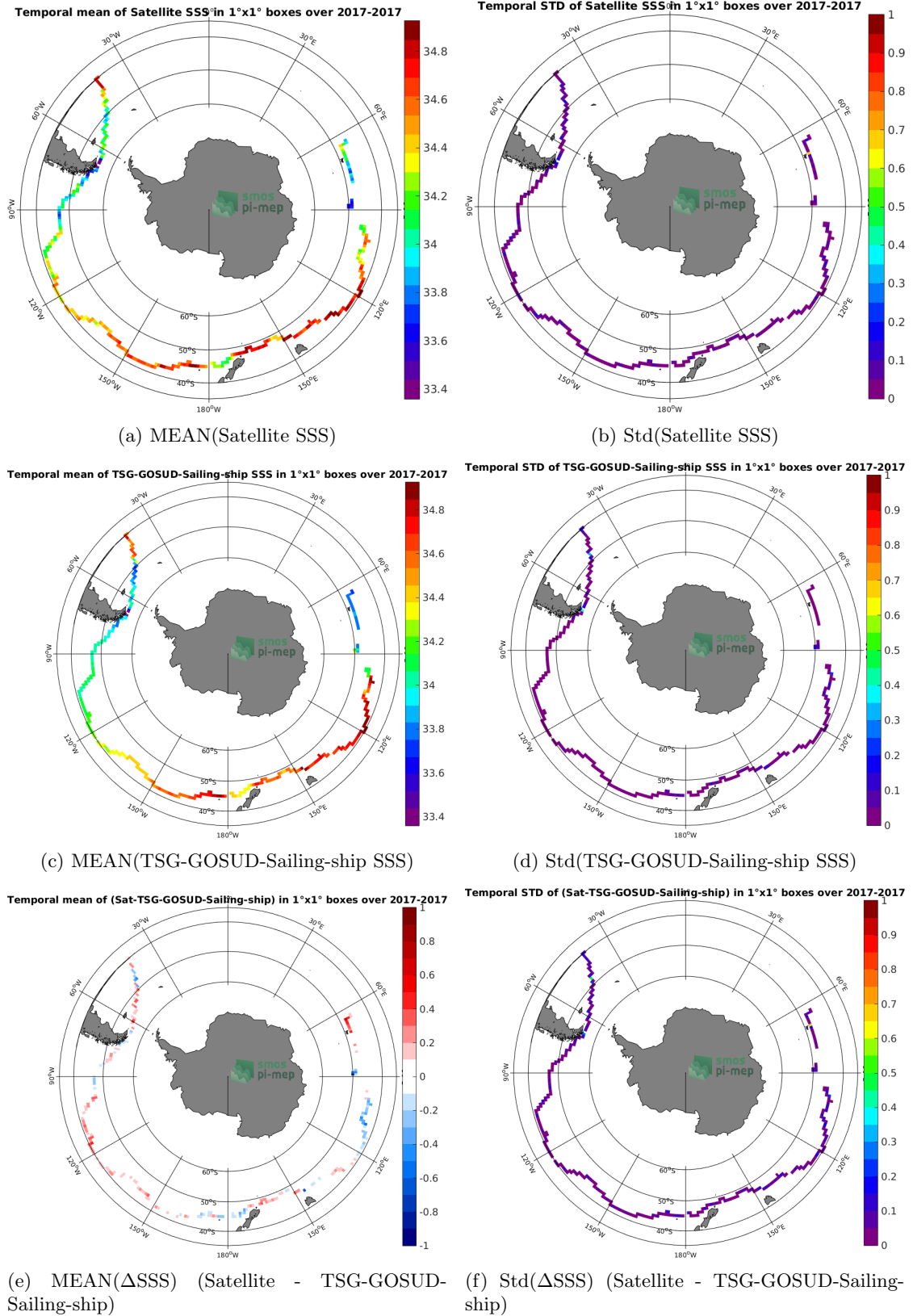
Figure 6: Temporal mean (left) and Std (right) of SSS from SMAP-L3-JPL-V4.2-MONTHLY-60KM (top), TSG-GOSUD-Sailing-ship (middle), and of \Delta SSS (Satellite - TSG-GOSUD-Sailing-ship). Only match-up pairs are used to generate these maps.
