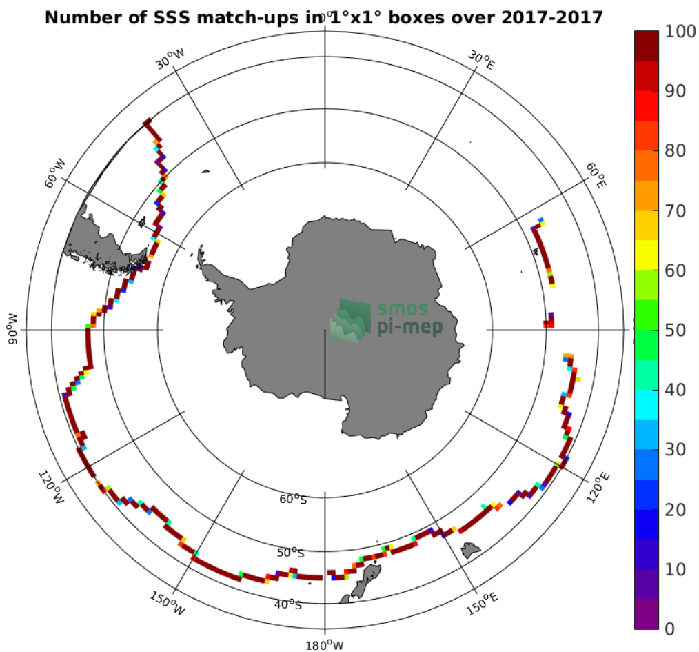
Figure 4: Number of SSS match-ups between TSG-GOSUD-Sailing-ship SSS and the SMAP-L3-JPL-V4.2-MONTHLY-60KM SSS product for the Roaring Forties and Furious Fifties Pi-MEP region over 1^\circ \times 1^\circ boxes and for the full satellite product period.
