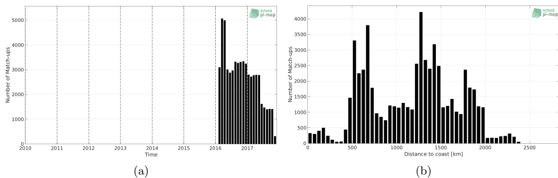
Figure 1: Number of match-ups between Surface drifters and SMAP-L3-JPL-V4.2-MONTHLY-60KM SSS as a function of time (a) and as function of the distance to coast (b) over the Roaring Forties and Furious Fifties Pi-MEP region and for the full satellite product period.
