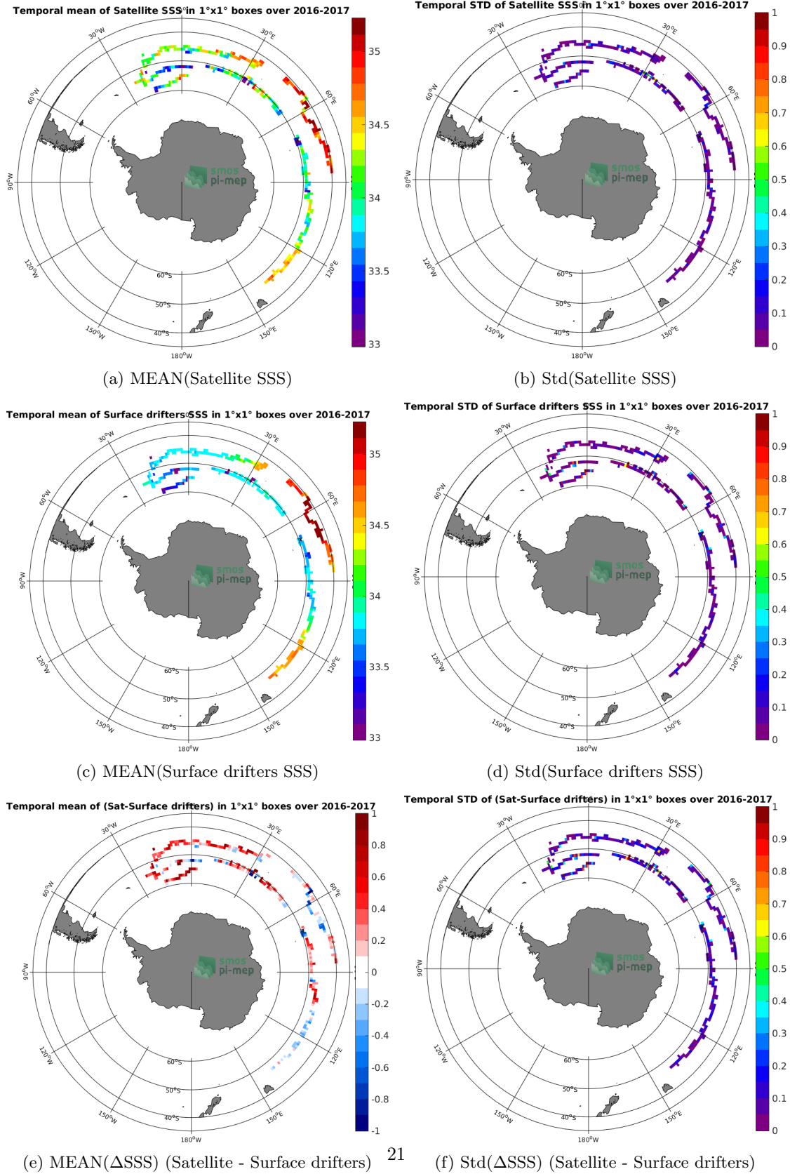
Figure 5: Temporal mean (left) and Std (right) of SSS from SMAP-L3-JPL-V4.2-MONTHLY-60KM (top), Surface drifters (middle), and of \Delta SSS (Satellite - Surface drifters). Only match-up pairs are used to generate these maps.
