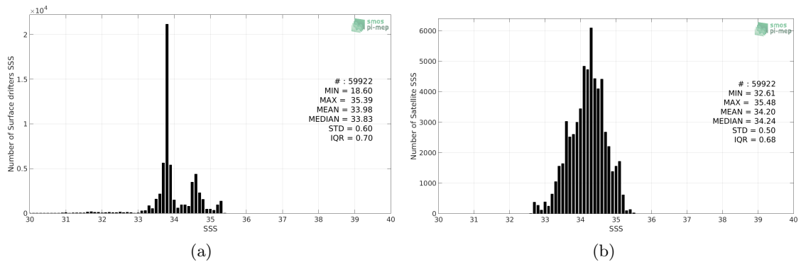
Figure 2: Histograms of SSS from Surface drifters (a) and SMAP-L3-JPL-V4.2-MONTHLY-60KM (b) considering all match-up pairs per bins of 0.1 over the Roaring Forties and Furious Fifties Pi-MEP region and for the full satellite product period.
