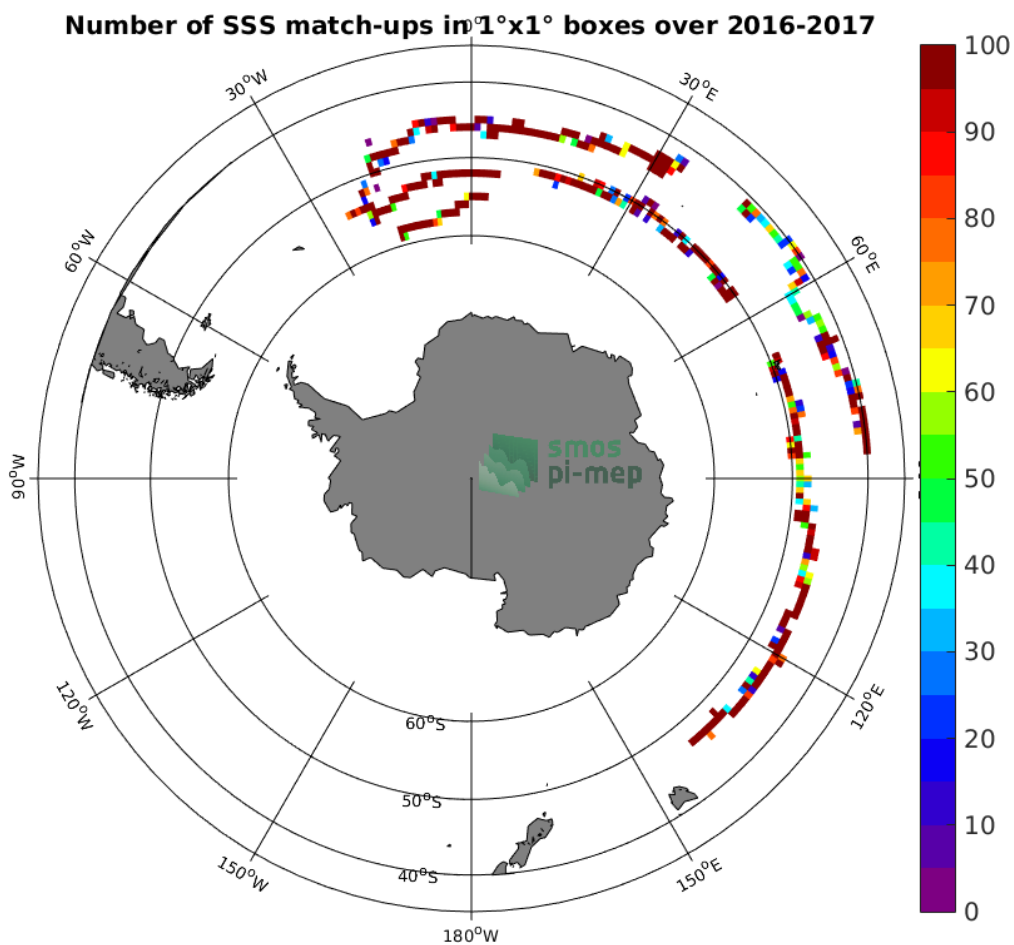
Figure 3: Number of SSS match-ups between Surface drifters SSS and the SMAP-L3-JPL-V4.2-MONTHLY-60KM SSS product for the Roaring Forties and Furious Fifties Pi-MEP region over 1°x1° boxes and for the full satellite product period.
