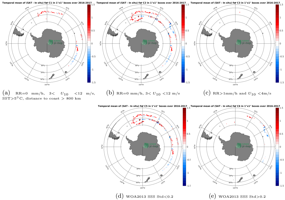
Figure 11: Temporal mean gridded over spatial boxes of size 1^\circ \times 1^\circ of \Delta SSS (SMAP-L3-JPL-V4.2-MONTHLY-60KM - Surface drifters) for 5 different subdatasets corresponding to:RR=0 mm/h, 3 < U_{10} < 12 m/s, SST >5^\circ C, distance to coast > 800 km (a), RR=0 mm/h, 3 < U_{10} < 12 m/s (b), RR >1 mm/h and U_{10} < 4 m/s (c), WOA2013 SSS Std <0.2 (d), WOA2013 SSS Std >0.2 (e).
