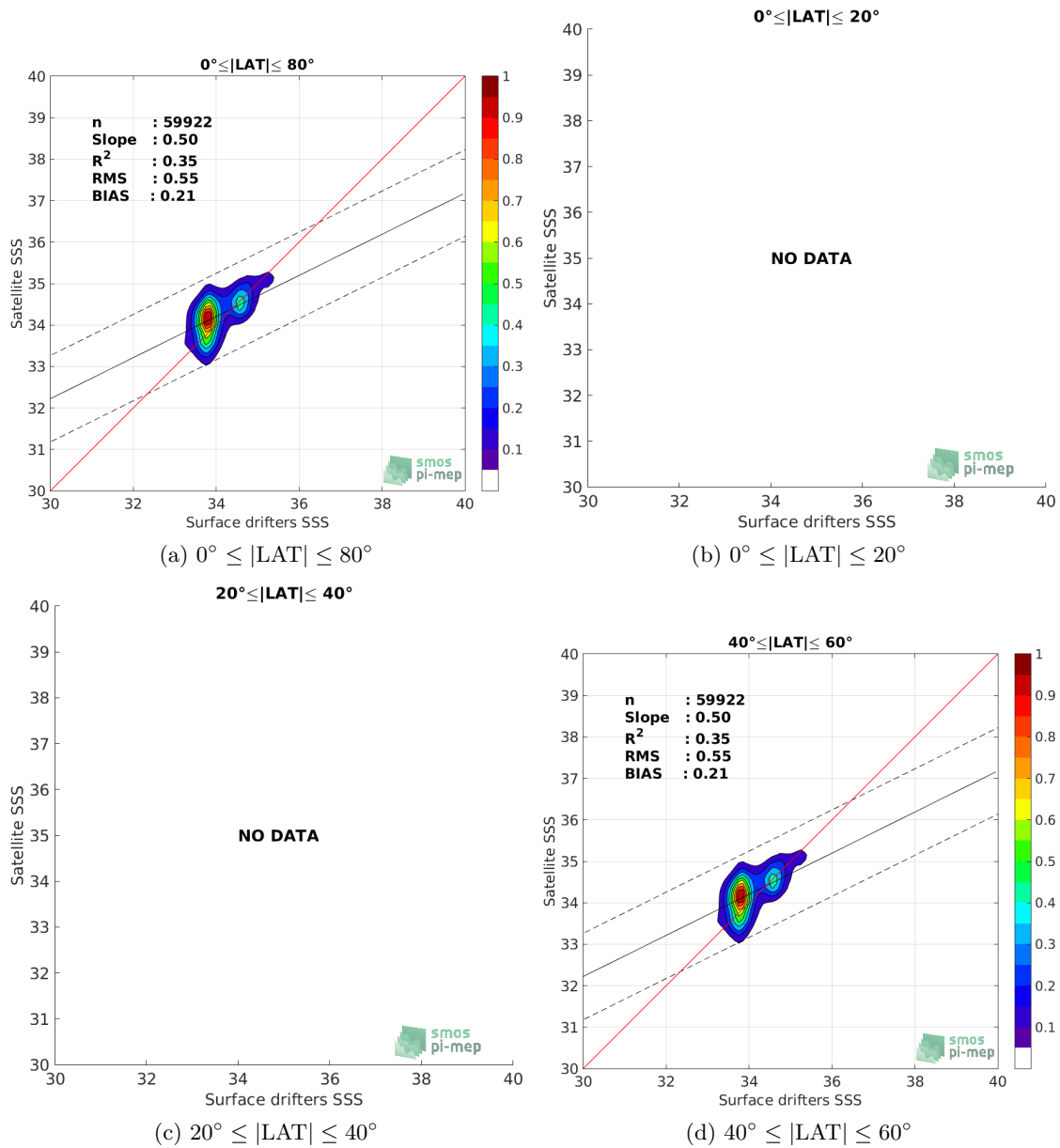
Figure 8: Contour maps of the concentration of SMAP-L3-JPL-V4.2-MONTHLY-60KM SSS (y-axis) versus Surface drifters SSS (x-axis) at match-up pairs for different latitude bands. For each plot, the red line shows x=y . The black thin and dashed lines indicate a linear fit through the data cloud and the \pm 95\% confidence levels, respectively. The number match-up pairs n , the slope and R^2 coefficient of the linear fit, the root mean square (RMS) and the mean bias between satellite and in situ data are indicated for each latitude band in each plots.
