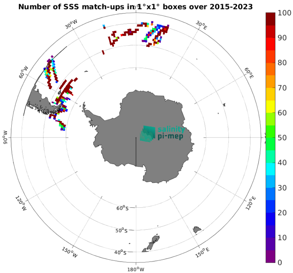
Figure 5: Number of SSS match-ups between TSG (Polarstern) SSS and the SMAP SSS L2 v6 (RSS) SSS product for the Roaring Forties and Furious Fifties Pi-MEP region over 1^\circ \times 1^\circ boxes and for the full satellite product period.
