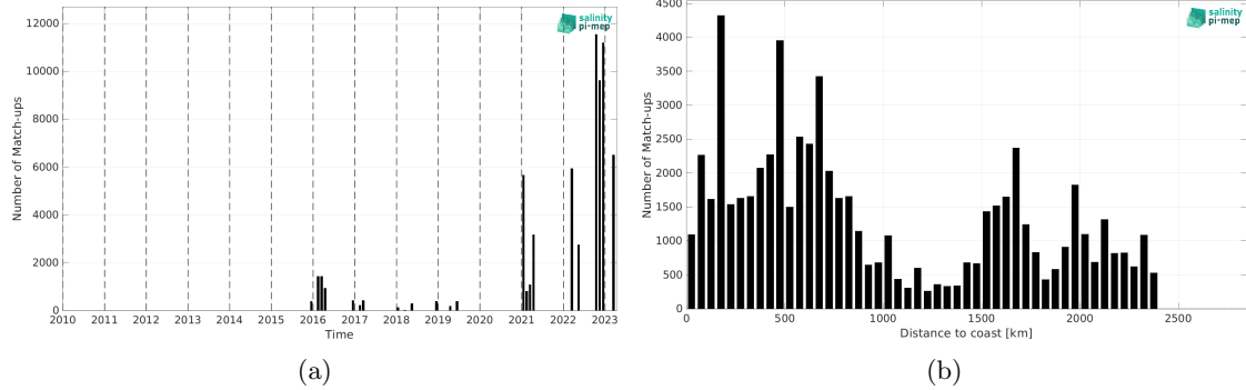
Figure 2: Number of match-ups between TSG (Polarstern) and SMAP SSS L2 v6 (RSS) SSS as a function of time (a) and as function of the distance to coast (b) over the Roaring Forties and Furious Fifties Pi-MEP region and for the full satellite product period.
