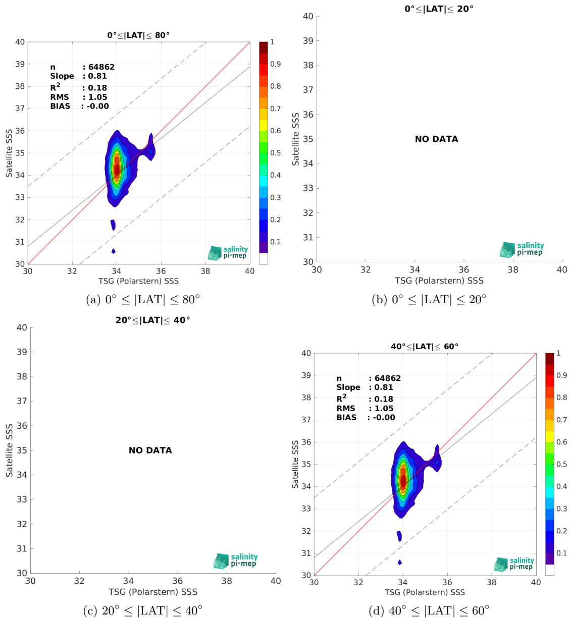
Figure 10: Contour maps of the concentration of SMAP SSS L2 v6 (RSS) SSS (y-axis) versus TSG (Polarstern) SSS (x-axis) at match-up pairs for different latitude bands. For each plot, the red line shows x=y . The black thin and dashed lines indicate a linear fit through the data cloud and the \pm 95\% confidence levels, respectively. The number match-up pairs n , the slope and R^2 coefficient of the linear fit, the root mean square (RMS) and the mean bias between satellite and in situ data are indicated for each latitude band in each plots.
