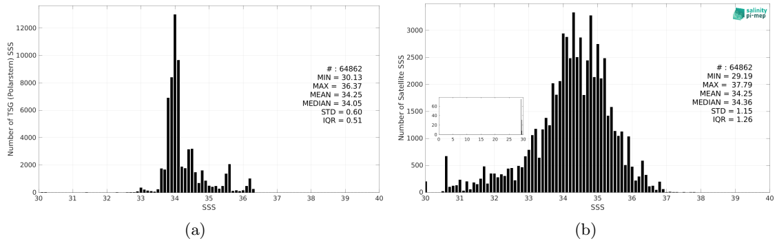
Figure 3: Histograms of SSS from TSG (Polarstern) (a) and SMAP SSS L2 v6 (RSS) (b) considering all match-up pairs per bins of 0.1 over the Roaring Forties and Furious Fifties Pi-MEP region and for the full satellite product period.
