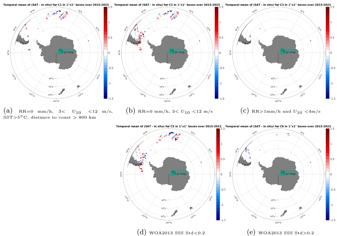
Figure 14: Temporal mean gridded over spatial boxes of size 1^\circ \times 1^\circ of \Delta SSS (SMAP SSS L2 v6 (RSS) - TSG (Polarstern)) for 5 different subdatasets corresponding to:RR=0 mm/h, 3 < U_{10} < 12 m/s, SST>5°C, distance to coast > 800 km (a), RR=0 mm/h, 3 < U_{10} < 12 m/s (b), RR>1mm/h and U_{10} < 4 m/s (c), WOA2013 SSS Std<0.2 (d), WOA2013 SSS Std>0.2 (e).
