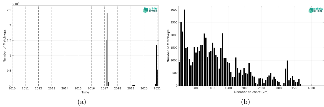
Figure 2: Number of match-ups between TSG (GOSUD-Sailing-ship) and SMAP SSS L2 v6 (RSS) SSS as a function of time (a) and as function of the distance to coast (b) over the Roaring Forties and Furious Fifties Pi-MEP region and for the full satellite product period.
