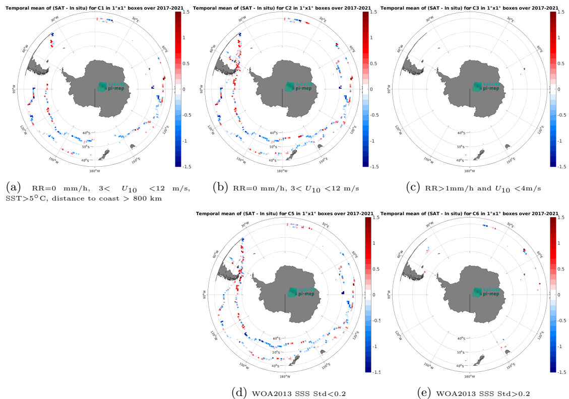
Figure 14: Temporal mean gridded over spatial boxes of size 1^\circ \times 1^\circ of \Delta\text{SSS} (SMAP SSS L2 v6 (RSS) - TSG (GOSUD-Sailing-ship)) for 5 different subdatasets corresponding to:RR=0 mm/h, 3 < U_{10} < 12 m/s, SST>5°C, distance to coast > 800 km (a), RR=0 mm/h, 3 < U_{10} < 12 m/s (b), RR>1mm/h and U_{10} < 4 m/s (c), WOA2013 SSS Std<0.2 (d), WOA2013 SSS Std>0.2 (e).
