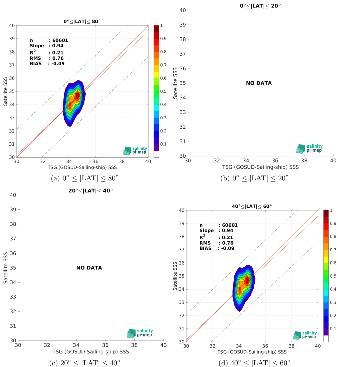
Figure 10: Contour maps of the concentration of SMAP SSS L2 v6 (RSS) SSS (y-axis) versus TSG (GOSUD-Sailing-ship) SSS (x-axis) at match-up pairs for different latitude bands. For each plot, the red line shows x=y . The black thin and dashed lines indicate a linear fit through the data cloud and the \pm 95\% confidence levels, respectively. The number match-up pairs n , the slope and R^2 coefficient of the linear fit, the root mean square (RMS) and the mean bias between satellite and in situ data are indicated for each latitude band in each plots.
