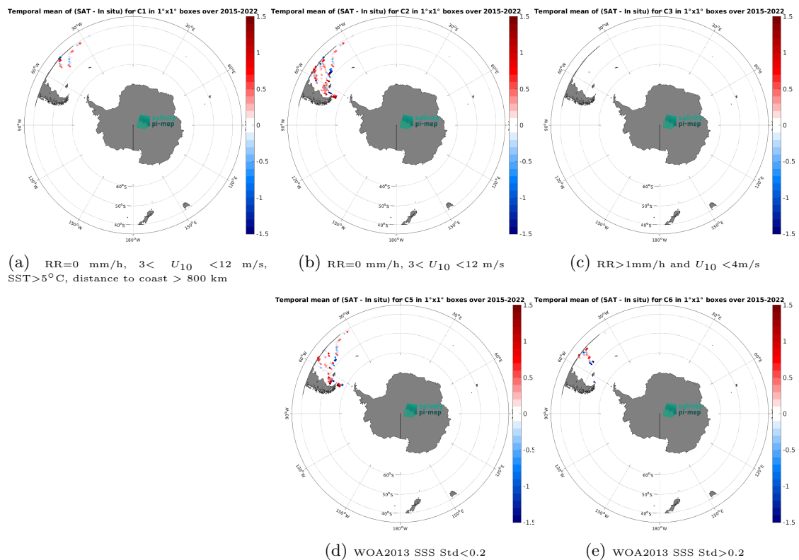
Figure 14: Temporal mean gridded over spatial boxes of size 1^\circ \times 1^\circ of \Delta SSS (SMAP SSS L2 v6 (RSS) - TSG (CSIC-UTM)) for 5 different subdatasets corresponding to:RR=0 mm/h, 3 < U_{10} < 12 m/s, SST>5°C, distance to coast > 800 km (a), RR=0 mm/h, 3 < U_{10} < 12 m/s (b), RR>1mm/h and U_{10} < 4 m/s (c), WOA2013 SSS Std<0.2 (d), WOA2013 SSS Std>0.2 (e).
