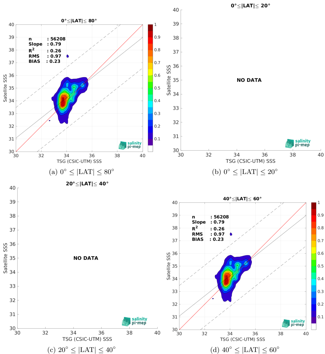
Figure 10: Contour maps of the concentration of SMAP SSS L2 v6 (RSS) SSS (y-axis) versus TSG (CSIC-UTM) SSS (x-axis) at match-up pairs for different latitude bands. For each plot, the red line shows x=y . The black thin and dashed lines indicate a linear fit through the data cloud and the \pm 95\% confidence levels, respectively. The number match-up pairs n , the slope and R^2 coefficient of the linear fit, the root mean square (RMS) and the mean bias between satellite and in situ data are indicated for each latitude band in each plot.
