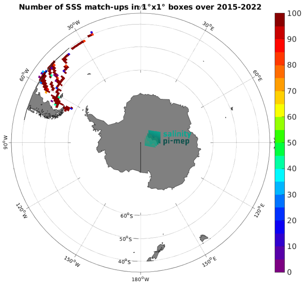
Figure 5: Number of SSS match-ups between TSG (CSIC-UTM) SSS and the SMAP SSS L2 v6 (RSS) SSS product for the Roaring Forties and Furious Fifties Pi-MEP region over 1^\circ \times 1^\circ boxes and for the full satellite product period.
