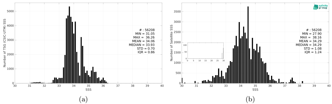
Figure 3: Histograms of SSS from TSG (CSIC-UTM) (a) and SMAP SSS L2 v6 (RSS) (b) considering all match-up pairs per bins of 0.1 over the Roaring Forties and Furious Fifties Pi-MEP region and for the full satellite product period.
