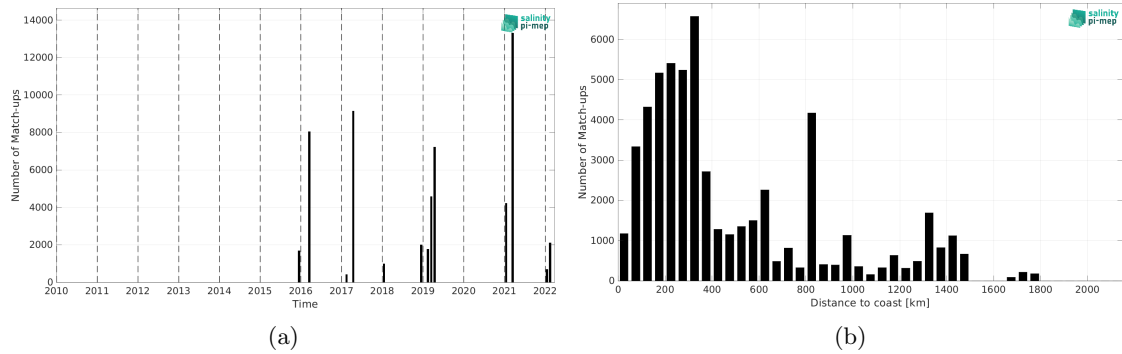
Figure 2: Number of match-ups between TSG (CSIC-UTM) and SMAP SSS L2 v6 (RSS) SSS as a function of time (a) and as function of the distance to coast (b) over the Roaring Forties and Furious Fifties Pi-MEP region and for the full satellite product period.
