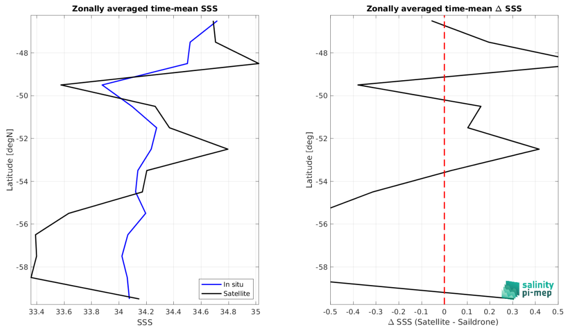
Figure 9: Left panel: Zonal mean SSS from SMAP SSS L2 v6 (RSS) satellite product (black) and from Sairdrone (blue). Right panel: Zonal mean of \Delta SSS (Satellite - Sairdrone) for all the collected Pi-MEP match-up pairs estimated over the full satellite product period.
