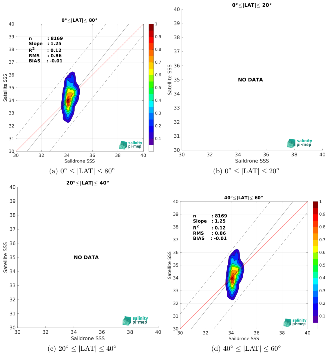
Figure 10: Contour maps of the concentration of SMAP SSS L2 v6 (RSS) SSS (y-axis) versus Saildrone SSS (x-axis) at match-up pairs for different latitude bands. For each plot, the red line shows x=y . The black thin and dashed lines indicate a linear fit through the data cloud and the \pm 95\% confidence levels, respectively. The number match-up pairs n , the slope and R^2 coefficient of the linear fit, the root mean square (RMS) and the mean bias between satellite and in situ data are indicated for each latitude band in each plots.
