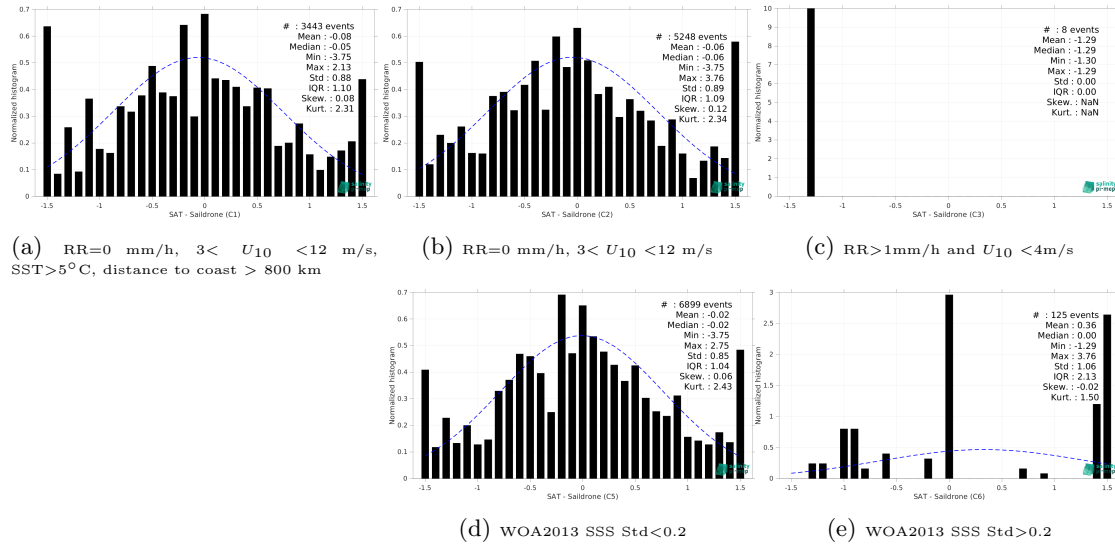
Figure 15: Normalized histogram of \Delta SSS (SMAP SSS L2 v6 (RSS) - Saildrone) for 5 different subdatasets corresponding to: RR=0 mm/h, 3 < U_{10} < 12 m/s, SST > 5°C, distance to coast > 800 km (a), RR=0 mm/h, 3 < U_{10} < 12 m/s (b), RR > 1mm/h and U_{10} < 4 m/s (c), WOA2013 SSS Std < 0.2 (d), WOA2013 SSS Std > 0.2 (e).
