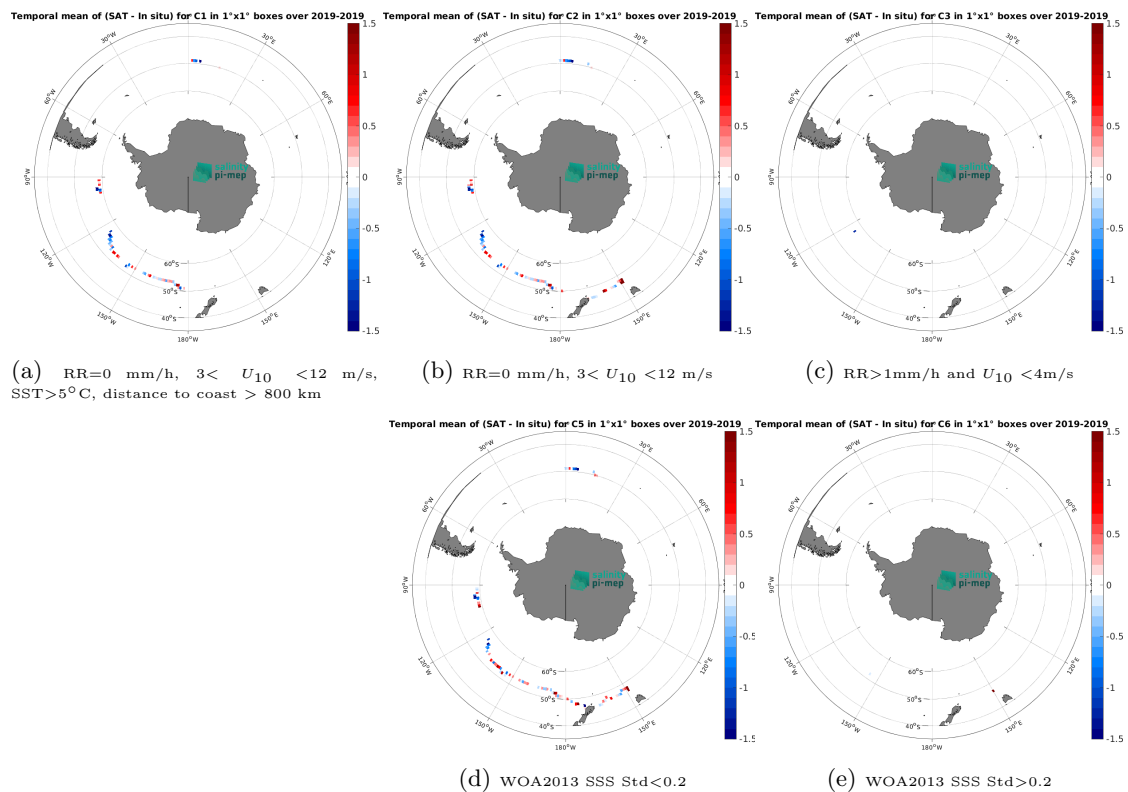
Figure 14: Temporal mean gridded over spatial boxes of size 1^\circ \times 1^\circ of \Delta\text{SSS} (SMAP SSS L2 v6 (RSS) - Saildrone) for 5 different subdatasets corresponding to:RR=0 mm/h, 3 < U_{10} < 12 m/s, SST>5°C, distance to coast > 800 km (a), RR=0 mm/h, 3 < U_{10} < 12 m/s (b), RR>1mm/h and U_{10} < 4 m/s (c), WOA2013 SSS Std<0.2 (d), WOA2013 SSS Std>0.2 (e).
