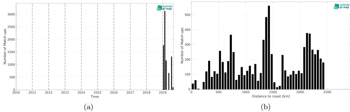
Figure 2: Number of match-ups between Saildrone and SMAP SSS L2 v6 (RSS) SSS as a function of time (a) and as function of the distance to coast (b) over the Roaring Forties and Furious Fifties Pi-MEP region and for the full satellite product period.
