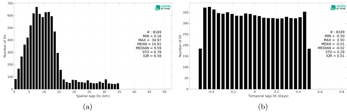
Figure 6: Histograms of the spatial (a) and temporal (b) lags between the location/time of the Saildrone measurement and the date of the corresponding SMAP SSS L2 v6 (RSS) SSS pixel.
