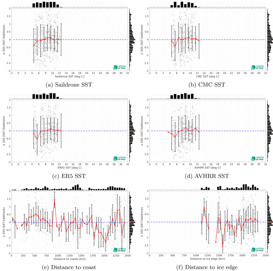
Figure 13: \Delta SSS (Satellite - Saitdrone) sorted as function of Saitdrone SST values (a), CMC SST (b), ERA5 SST (c), AVHRR SST (d), distance to coast (e) and distance to ice edge (f). In all plots the median and Std of \Delta SSS for each bin is indicated by the red curves and black vertical thick bars ( \pm 1 Std). Links to similar figures sorted as function of Sea ice fraction and in situ measurement depth .
