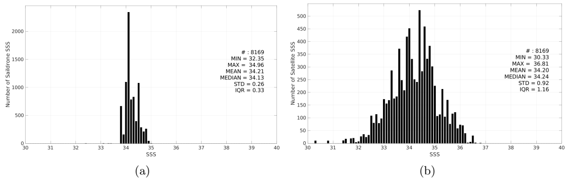
Figure 3: Histograms of SSS from Saildrone (a) and SMAP SSS L2 v6 (RSS) (b) considering all match-up pairs per bins of 0.1 over the Roaring Forties and Furious Fifties Pi-MEP region and for the full satellite product period.
