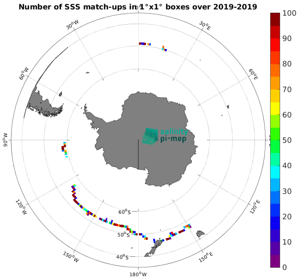
Figure 5: Number of SSS match-ups between Saildrone SSS and the SMAP SSS L2 v6 (RSS) SSS product for the Roaring Forties and Furious Fifties Pi-MEP region over 1^\circ \times 1^\circ boxes and for the full satellite product period.
