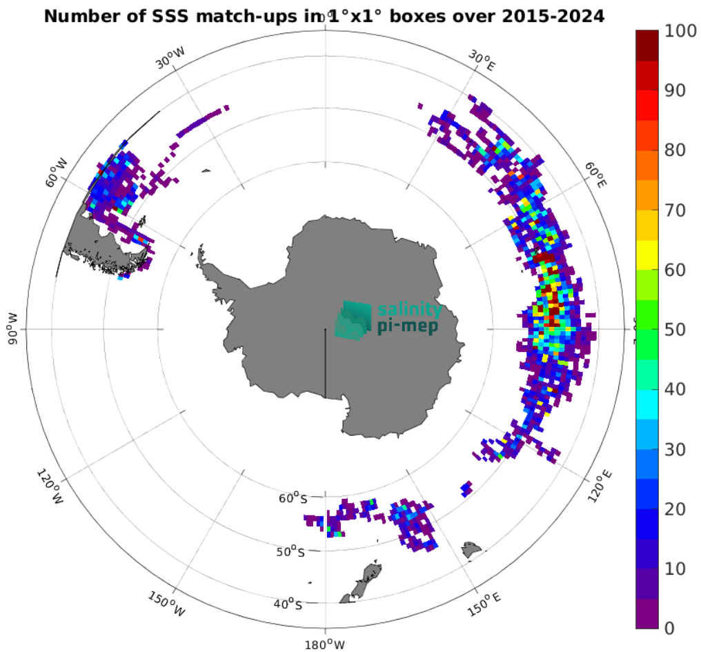
Figure 5: Number of SSS match-ups between Marine mammals SSS and the SMAP SSS L2 v6 (RSS) SSS product for the Roaring Forties and Furious Fifties Pi-MEP region over 1^\circ \times 1^\circ boxes and for the full satellite product period.
