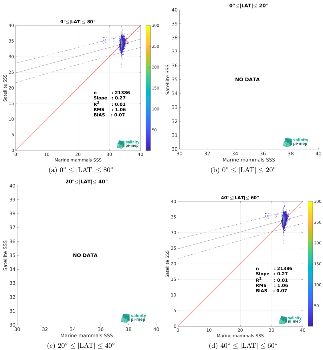
Figure 10: Contour maps of the concentration of SMAP SSS L2 v6 (RSS) SSS (y-axis) versus Marine mammals SSS (x-axis) at match-up pairs for different latitude bands. For each plot, the red line shows x=y . The black thin and dashed lines indicate a linear fit through the data cloud and the \pm 95\% confidence levels, respectively. The number match-up pairs n , the slope and R^2 coefficient of the linear fit, the root mean square (RMS) and the mean bias between satellite and in situ data are indicated for each latitude band in each plots.
