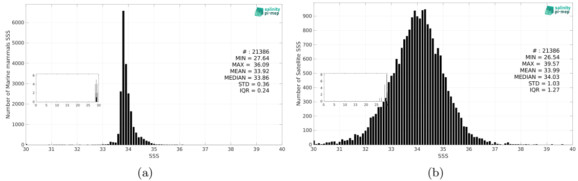
Figure 3: Histograms of SSS from Marine mammals (a) and SMAP SSS L2 v6 (RSS) (b) considering all match-up pairs per bins of 0.1 over the Roaring Forties and Furious Fifties Pi-MEP region and for the full satellite product period.
