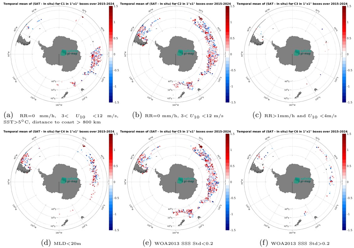
Figure 14: Temporal mean gridded over spatial boxes of size 1^\circ \times 1^\circ of \Delta SSS (SMAP SSS L2 v6 (RSS) - Marine mammals) for 6 different subdatasets corresponding to:RR=0 mm/h, 3 < U_{10} < 12 m/s, SST>5°C, distance to coast > 800 km (a), RR=0 mm/h, 3 < U_{10} < 12 m/s (b), RR>1mm/h and U_{10} < 4 m/s (c),MLD<20m (d),WOA2013 SSS Std<0.2 (e),WOA2013 SSS Std>0.2 (f).
