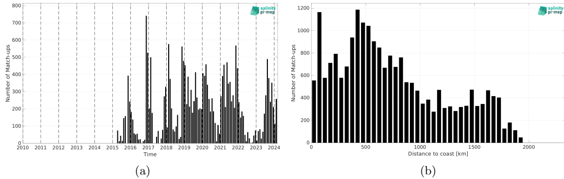
Figure 2: Number of match-ups between Marine mammals and SMAP SSS L2 v6 (RSS) SSS as a function of time (a) and as function of the distance to coast (b) over the Roaring Forties and Furious Fifties Pi-MEP region and for the full satellite product period.
