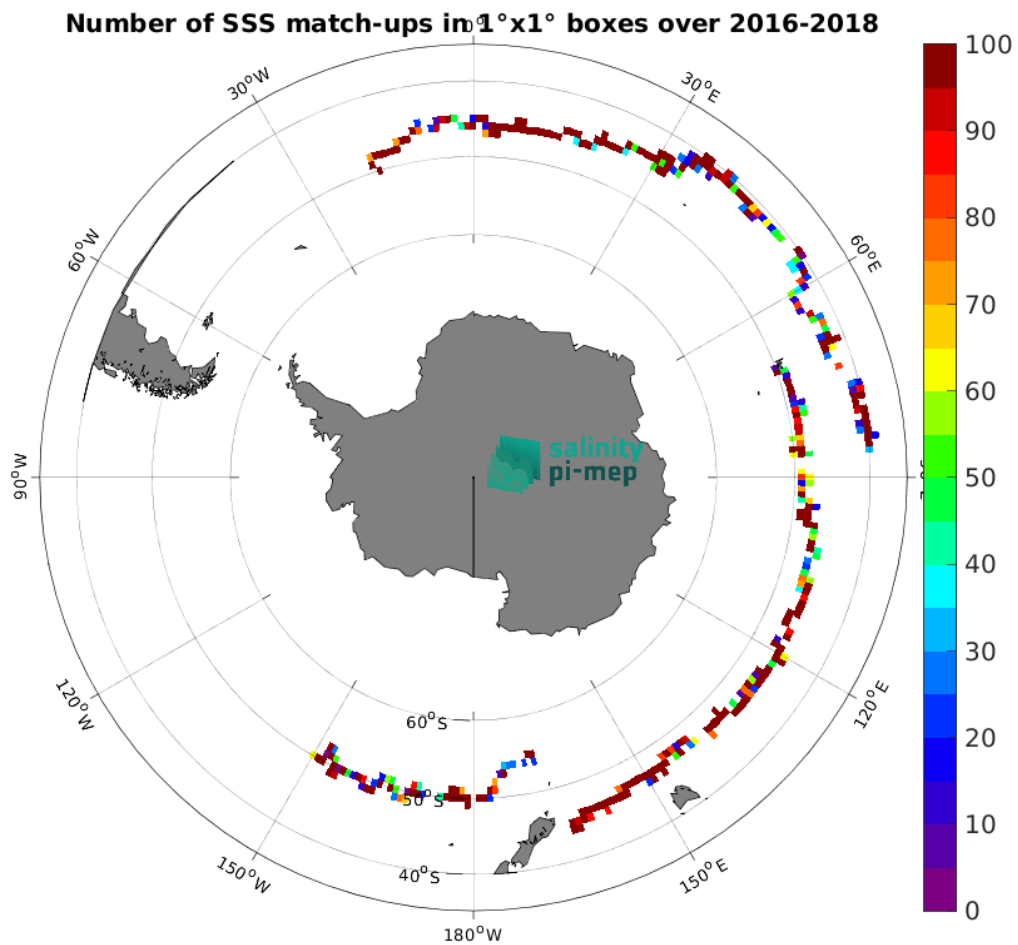
Figure 4: Number of SSS match-ups between Surface drifters SSS and the SMAP SSS L2 v6 (RSS) SSS product for the Roaring Forties and Furious Fifties Pi-MEP region over 1^\circ \times 1^\circ boxes and for the full satellite product period.
