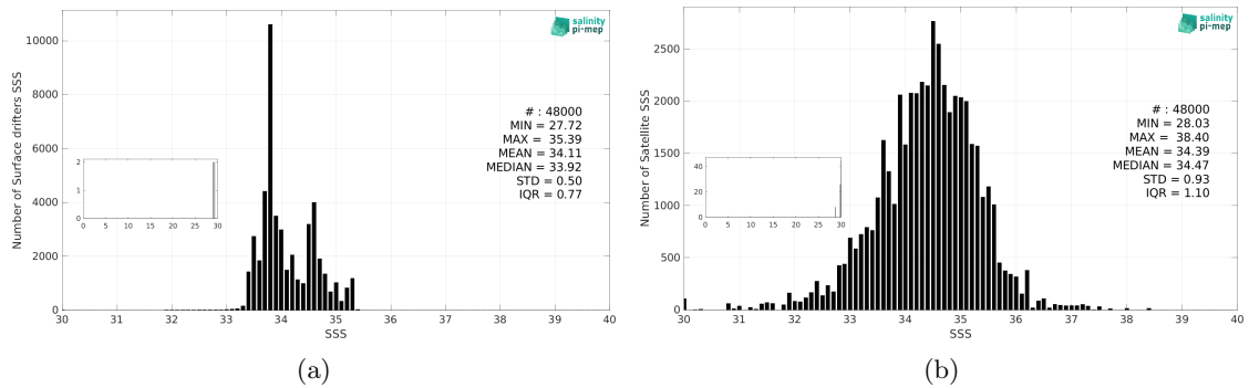
Figure 3: Histograms of SSS from Surface drifters (a) and SMAP SSS L2 v6 (RSS) (b) considering all match-up pairs per bins of 0.1 over the Roaring Forties and Furious Fifties Pi-MEP region and for the full satellite product period.
