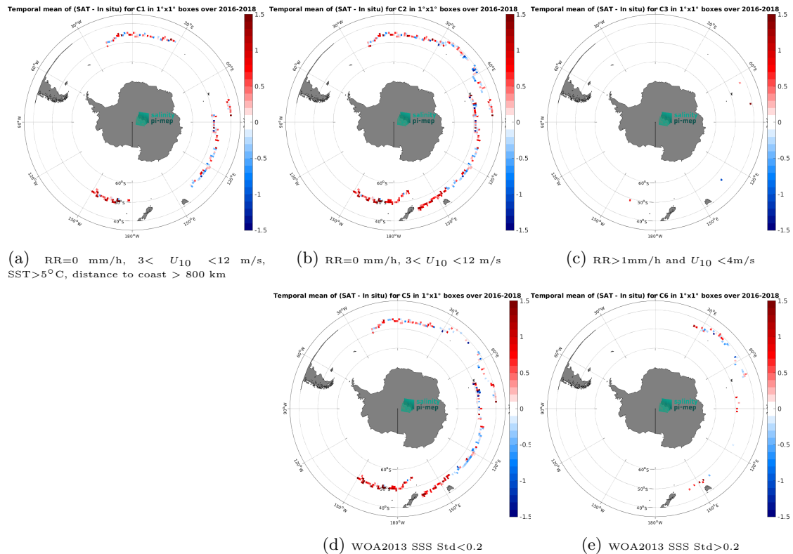
Figure 13: Temporal mean gridded over spatial boxes of size 1^\circ \times 1^\circ of \Delta SSS (SMAP SSS L2 v6 (RSS) - Surface drifters) for 5 different subdatasets corresponding to:RR=0 mm/h, 3 < U_{10} < 12 m/s, SST >5^\circ C, distance to coast > 800 km (a), RR=0 mm/h, 3 < U_{10} < 12 m/s (b), RR >1 mm/h and U_{10} < 4 m/s (c), WOA2013 SSS Std <0.2 (d), WOA2013 SSS Std >0.2 (e).
