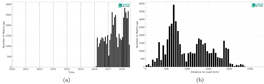
Figure 2: Number of match-ups between Surface drifters and SMAP SSS L2 v6 (RSS) SSS as a function of time (a) and as function of the distance to coast (b) over the Roaring Forties and Furious Fifties Pi-MEP region and for the full satellite product period.
