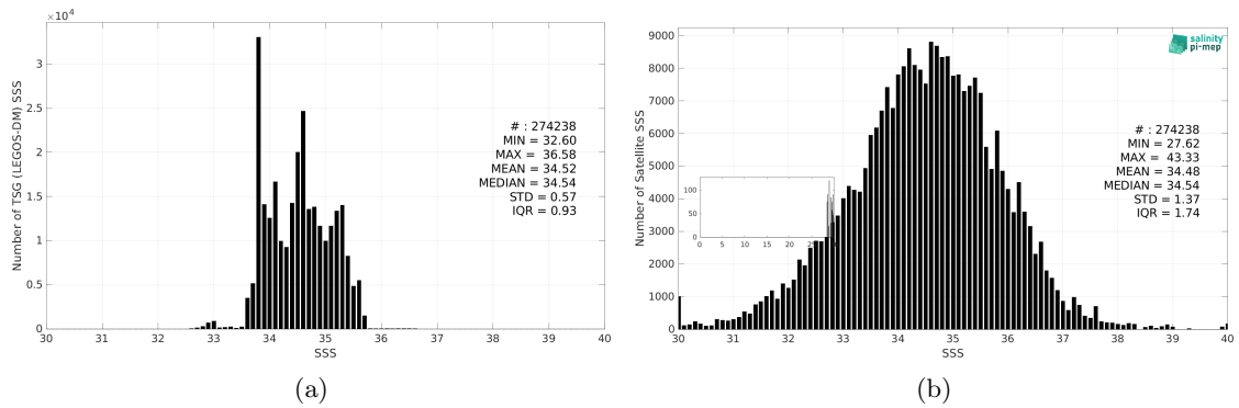
Figure 3: Histograms of SSS from TSG (LEGOS-DM) (a) and SMAP SSS L2 v6 - 40 km (RSS) (b) considering all match-up pairs per bins of 0.1 over the Roaring Forties and Furious Fifties Pi-MEP region and for the full satellite product period.
