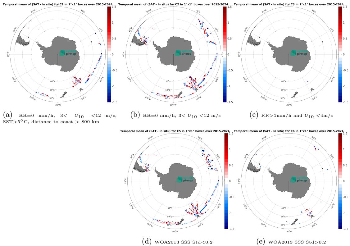
Figure 14: Temporal mean gridded over spatial boxes of size 1^\circ \times 1^\circ of \Delta SSS (SMAP SSS L2 v6 - 40 km (RSS) - TSG (LEGOS-DM)) for 5 different subdatasets corresponding to:RR=0 mm/h, 3 < U_{10} < 12 m/s, SST>5°C, distance to coast > 800 km (a), RR=0 mm/h, 3 < U_{10} < 12 m/s (b), RR>1mm/h and U_{10} < 4 m/s (c), WOA2013 SSS Std<0.2 (d), WOA2013 SSS Std>0.2 (e).
