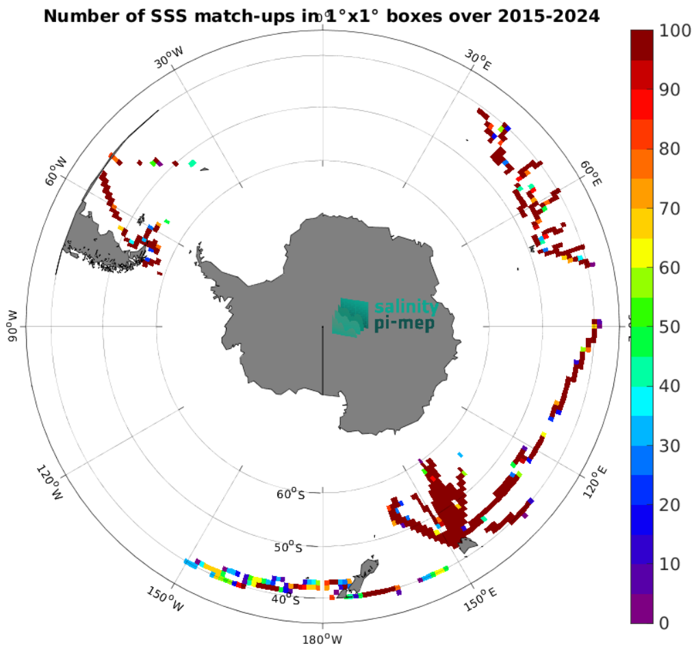
Figure 5: Number of SSS match-ups between TSG (LEGOS-DM) SSS and the SMAP SSS L2 v6 - 40 km (RSS) SSS product for the Roaring Forties and Furious Fifties Pi-MEP region over 1^\circ \times 1^\circ boxes and for the full satellite product period.
