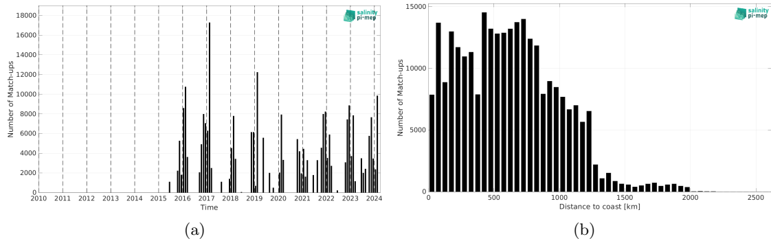
Figure 2: Number of match-ups between TSG (LEGOS-DM) and SMAP SSS L2 v6 - 40 km (RSS) SSS as a function of time (a) and as function of the distance to coast (b) over the Roaring Forties and Furious Fifties Pi-MEP region and for the full satellite product period.
