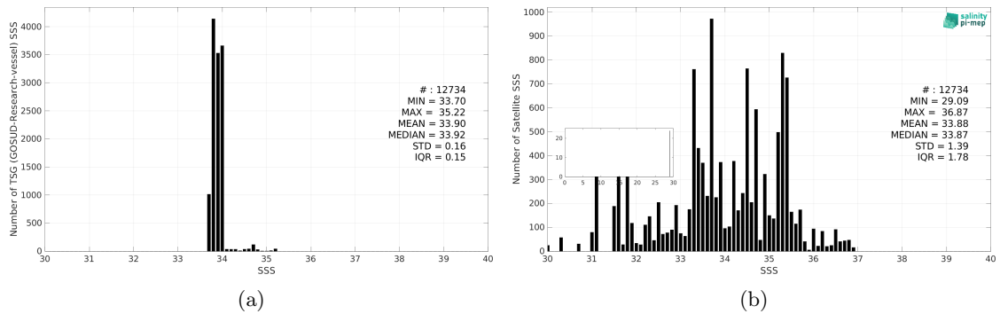
Figure 3: Histograms of SSS from TSG (GOSUD-Research-vessel) (a) and SMAP SSS L2 v6 - 40 km (RSS) (b) considering all match-up pairs per bins of 0.1 over the Roaring Forties and Furious Fifties Pi-MEP region and for the full satellite product period.
