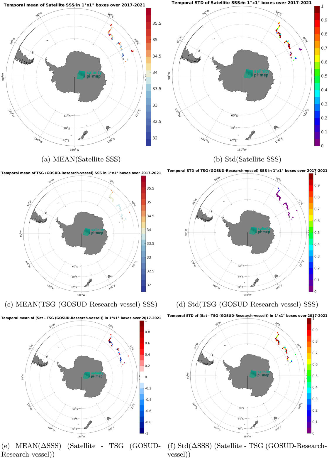
Figure 7: Temporal mean (left) and Std (right) of SSS from SMAP SSS L2 v6 - 40 km (RSS) (top), TSG (GOSUD-Research-vessel) (middle), and of \Delta SSS (Satellite - TSG (GOSUD-Research-vessel)). Only match-up pairs are used to generate these maps.
