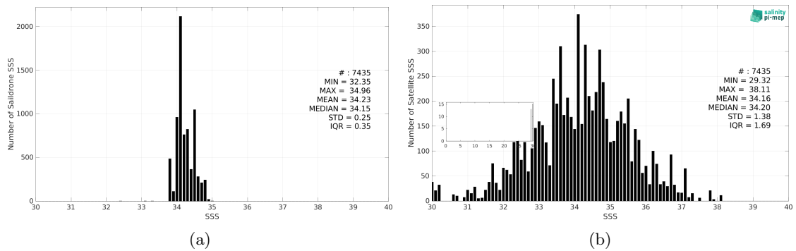
Figure 3: Histograms of SSS from Saildrone (a) and SMAP SSS L2 v6 - 40 km (RSS) (b) considering all match-up pairs per bins of 0.1 over the Roaring Forties and Furious Fifties Pi-MEP region and for the full satellite product period.
