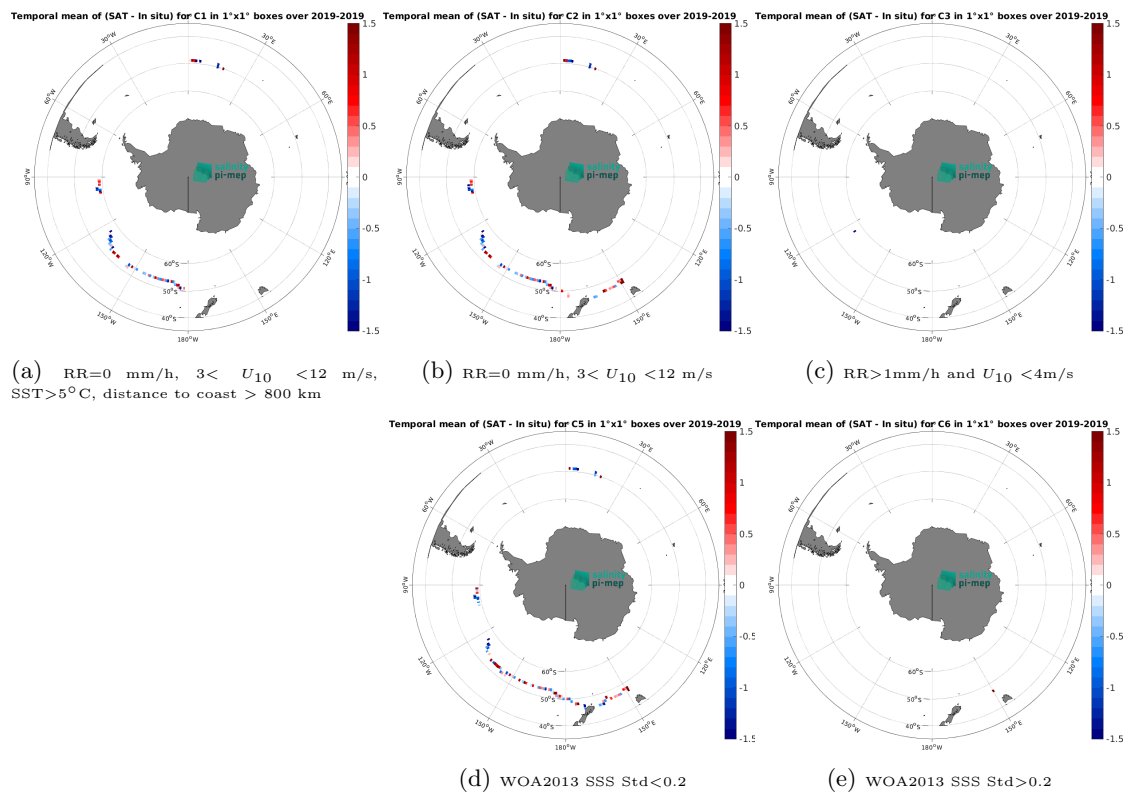
Figure 14: Temporal mean gridded over spatial boxes of size 1^\circ \times 1^\circ of \Delta SSS (SMAP SSS L2 v6 - 40 km (RSS) - Saldrone) for 5 different subdatasets corresponding to: RR=0 mm/h, 3 < U_{10} < 12 m/s, SST > 5^\circ\text{C} , distance to coast > 800 km (a), RR=0 mm/h, 3 < U_{10} < 12 m/s (b), RR > 1 mm/h and U_{10} < 4 m/s (c), WOA2013 SSS Std < 0.2 (d), WOA2013 SSS Std > 0.2 (e).
