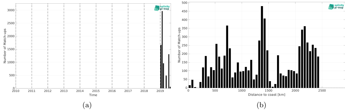
Figure 2: Number of match-ups between Saildrone and SMAP SSS L2 v6 - 40 km (RSS) SSS as a function of time (a) and as function of the distance to coast (b) over the Roaring Forties and Furious Fifties Pi-MEP region and for the full satellite product period.
