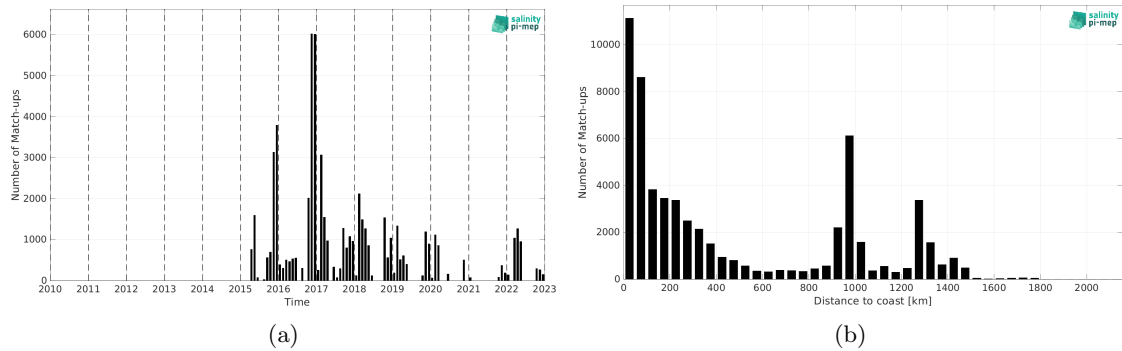
Figure 1: Number of match-ups between TSG (SAMOS) and SMAP SSS L2 v5 (RSS) SSS as a function of time (a) and as function of the distance to coast (b) over the Roaring Forties and Furious Fifties Pi-MEP region and for the full satellite product period.
