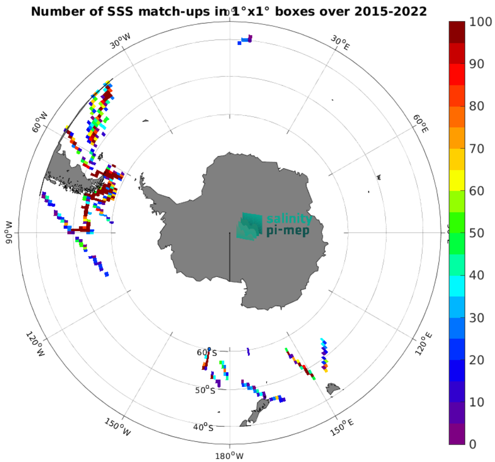
Figure 4: Number of SSS match-ups between TSG (SAMOS) SSS and the SMAP SSS L2 v5 (RSS) SSS product for the Roaring Forties and Furious Fifties Pi-MEP region over 1^\circ \times 1^\circ boxes and for the full satellite product period.
