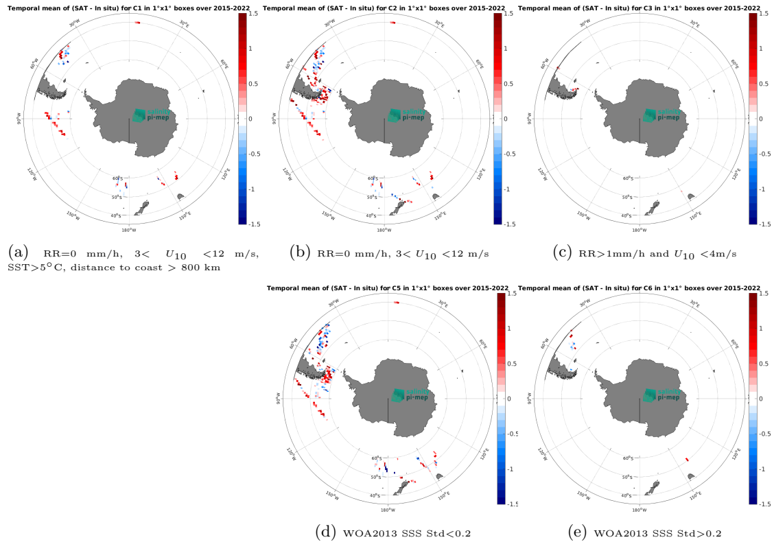
Figure 12: Temporal mean gridded over spatial boxes of size 1^{\circ}\times 1^{\circ} of \Delta\text{SSS} (SMAP SSS L2 v5 (RSS) - TSG (SAMOS)) for 5 different subdatasets corresponding to:RR=0 mm/h, 3 < U_{10} < 12 m/s, SST >5^{\circ}\text{C} , distance to coast > 800 km (a), RR=0 mm/h, 3 < U_{10} < 12 m/s (b), RR >1 mm/h and U_{10} < 4 m/s (c), WOA2013 SSS Std <0.2 (d), WOA2013 SSS Std >0.2 (e).
