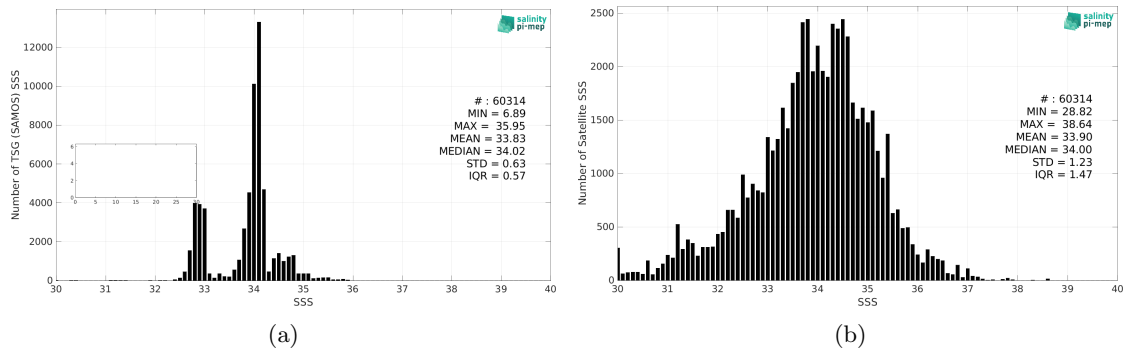
Figure 2: Histograms of SSS from TSG (SAMOS) (a) and SMAP SSS L2 v5 (RSS) (b) considering all match-up pairs per bins of 0.1 over the Roaring Forties and Furious Fifties Pi-MEP region and for the full satellite product period.
