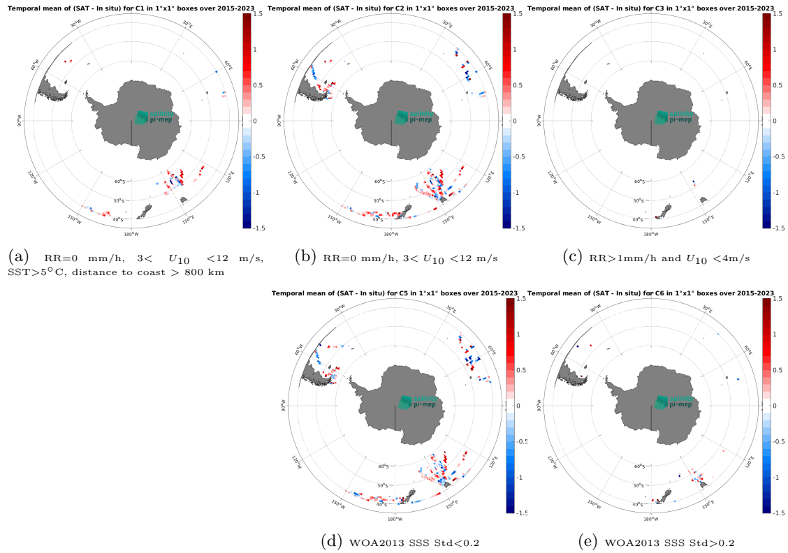
Figure 12: Temporal mean gridded over spatial boxes of size 1^{\circ}\times 1^{\circ} of \Delta\text{SSS} (SMAP SSS L2 v5 (RSS) - TSG (LEGOS-DM)) for 5 different subdatasets corresponding to: \text{RR}=0 mm/h, 3 < U_{10} < 12 m/s, \text{SST}>5^{\circ}\text{C} , distance to coast > 800 km (a), \text{RR}=0 mm/h, 3 < U_{10} < 12 m/s (b), \text{RR}>1\text{mm/h} and U_{10} < 4\text{m/s} (c), WOA2013 SSS Std < 0.2 (d), WOA2013 SSS Std > 0.2 (e).
