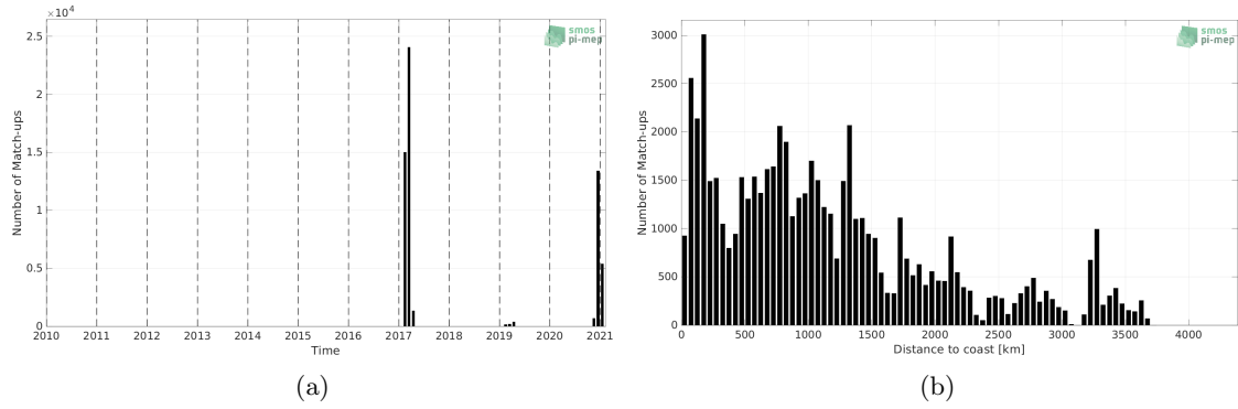
Figure 1: Number of match-ups between TSG (GOSUD-Sailing-ship) and SMAP SSS L2 v5 (RSS) SSS as a function of time (a) and as function of the distance to coast (b) over the Roaring Forties and Furious Fifties Pi-MEP region and for the full satellite product period.
