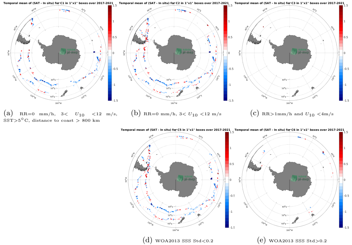
Figure 12: Temporal mean gridded over spatial boxes of size 1^\circ \times 1^\circ of \Delta SSS (SMAP SSS L2 v5 (RSS) - TSG (GOSUD-Sailing-ship)) for 5 different subdatasets corresponding to: RR=0 mm/h, 3 < U_{10} < 12 m/s, SST > 5^\circ\text{C} , distance to coast > 800 km (a), RR=0 mm/h, 3 < U_{10} < 12 m/s (b), RR > 1 mm/h and U_{10} < 4 m/s (c), WOA2013 SSS Std < 0.2 (d), WOA2013 SSS Std > 0.2 (e).
