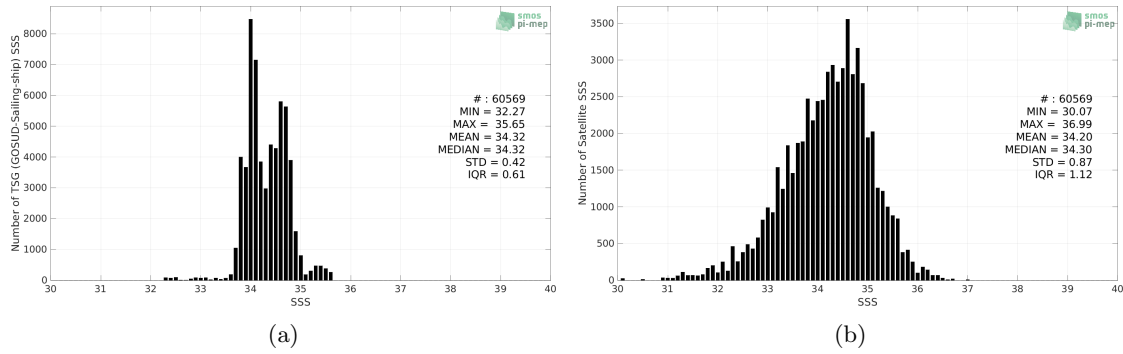
Figure 2: Histograms of SSS from TSG (GOSUD-Sailing-ship) (a) and SMAP SSS L2 v5 (RSS) (b) considering all match-up pairs per bins of 0.1 over the Roaring Forties and Furious Fifties Pi-MEP region and for the full satellite product period.
