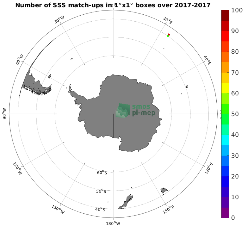
Figure 4: Number of SSS match-ups between TSG (GOSUD-Research-vessel) SSS and the SMAP SSS L2 v5 (RSS) SSS product for the Roaring Forties and Furious Fifties Pi-MEP region over 1^\circ \times 1^\circ boxes and for the full satellite product period.
