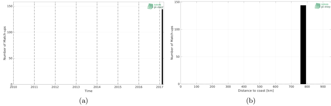
Figure 1: Number of match-ups between TSG (GOSUD-Research-vessel) and SMAP SSS L2 v5 (RSS) SSS as a function of time (a) and as function of the distance to coast (b) over the Roaring Forties and Furious Fifties Pi-MEP region and for the full satellite product period.
