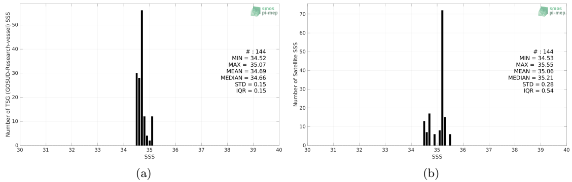
Figure 2: Histograms of SSS from TSG (GOSUD-Research-vessel) (a) and SMAP SSS L2 v5 (RSS) (b) considering all match-up pairs per bins of 0.1 over the Roaring Forties and Furious Fifties Pi-MEP region and for the full satellite product period.
