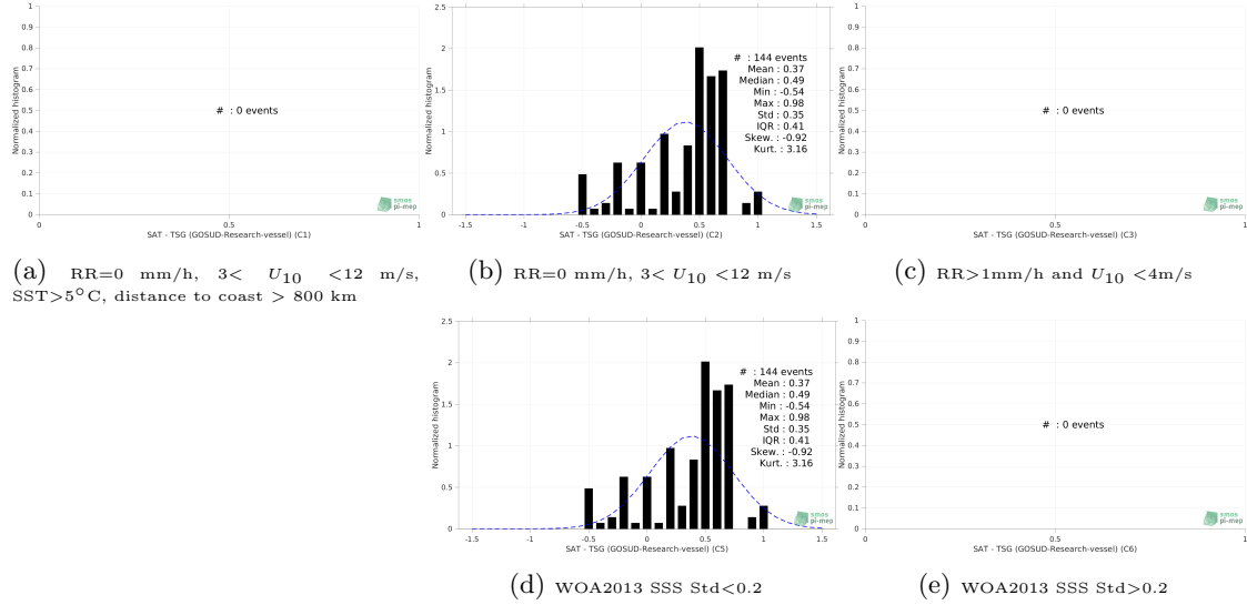
Figure 13: Normalized histogram of \Delta SSS (SMAP SSS L2 v5 (RSS) - TSG (GOSUD-Research-vessel)) for 5 different subdatasets corresponding to: RR=0 mm/h, 3 < U_{10} < 12 m/s, SST>5°C, distance to coast > 800 km (a), RR=0 mm/h, 3 < U_{10} < 12 m/s (b), RR>1mm/h and U_{10} < 4 m/s (c), WOA2013 SSS Std<0.2 (d), WOA2013 SSS Std>0.2 (e).
