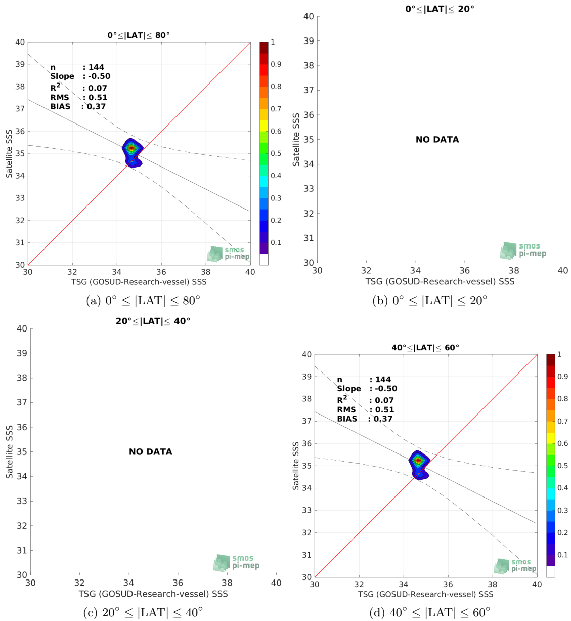
Figure 9: Contour maps of the concentration of SMAP SSS L2 v5 (RSS) SSS (y-axis) versus TSG (GOSUD-Research-vessel) SSS (x-axis) at match-up pairs for different latitude bands. For each plot, the red line shows x=y . The black thin and dashed lines indicate a linear fit through the data cloud and the \pm 95\% confidence levels, respectively. The number match-up pairs n , the slope and R^2 coefficient of the linear fit, the root mean square (RMS) and the mean bias between satellite and in situ data are indicated for each latitude band in each plots.
