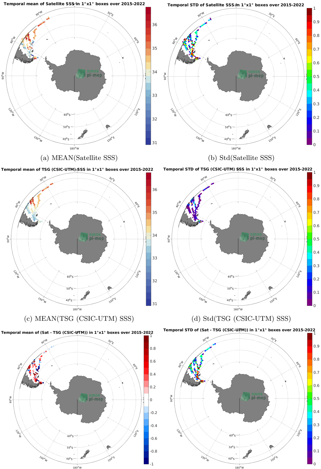
(e) MEAN( \Delta SSS) (Satellite - TSG (CSIC-UTM)) 17 (f) Std( \Delta SSS) (Satellite - TSG (CSIC-UTM))
