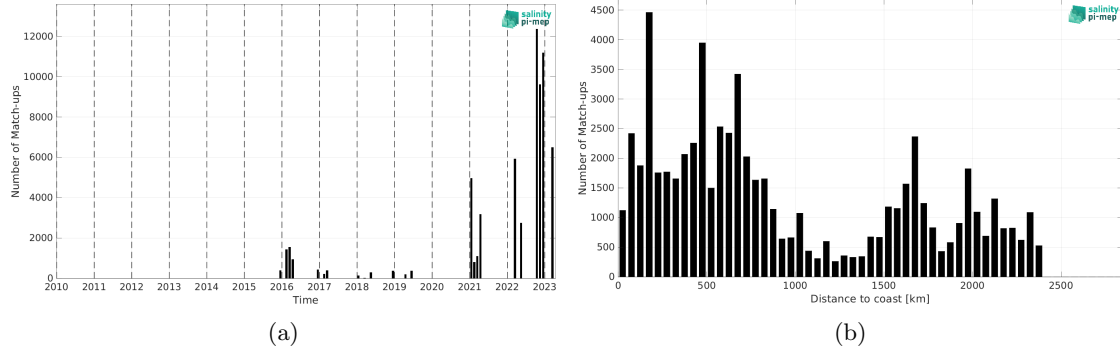
Figure 2: Number of match-ups between TSG (Polarstern) and SMAP SSS L2 v5.3 (RSS) SSS as a function of time (a) and as function of the distance to coast (b) over the Roaring Forties and Furious Fifties Pi-MEP region and for the full satellite product period.
