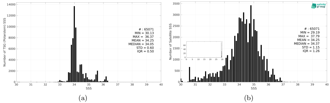
Figure 3: Histograms of SSS from TSG (Polarstern) (a) and SMAP SSS L2 v5.3 (RSS) (b) considering all match-up pairs per bins of 0.1 over the Roaring Forties and Furious Fifties Pi-MEP region and for the full satellite product period.
