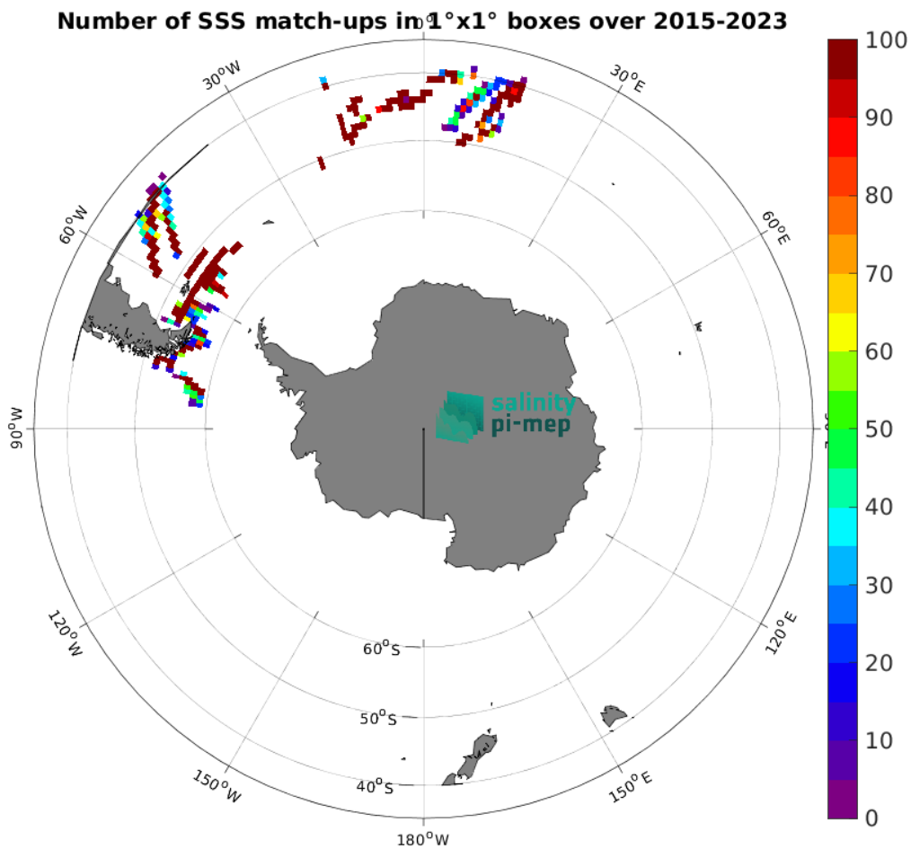
Figure 5: Number of SSS match-ups between TSG (Polarstern) SSS and the SMAP SSS L2 v5.3 (RSS) SSS product for the Roaring Forties and Furious Fifties Pi-MEP region over 1^\circ \times 1^\circ boxes and for the full satellite product period.
