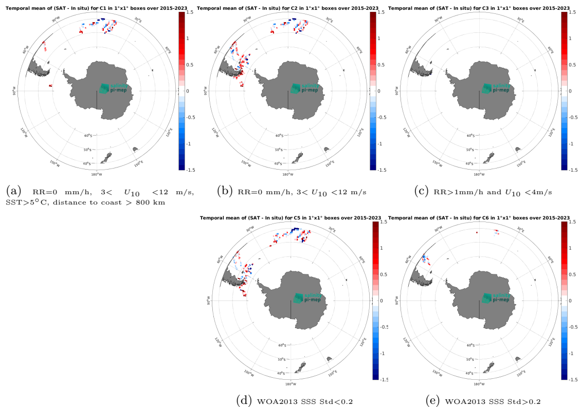
Figure 14: Temporal mean gridded over spatial boxes of size 1^\circ \times 1^\circ of \Delta SSS (SMAP SSS L2 v5.3 (RSS) - TSG (Polarstern)) for 5 different subdatasets corresponding to:RR=0 mm/h, 3 < U_{10} < 12 m/s, SST>5°C, distance to coast > 800 km (a), RR=0 mm/h, 3 < U_{10} < 12 m/s (b), RR>1mm/h and U_{10} < 4 m/s (c), WOA2013 SSS Std<0.2 (d), WOA2013 SSS Std>0.2 (e).
