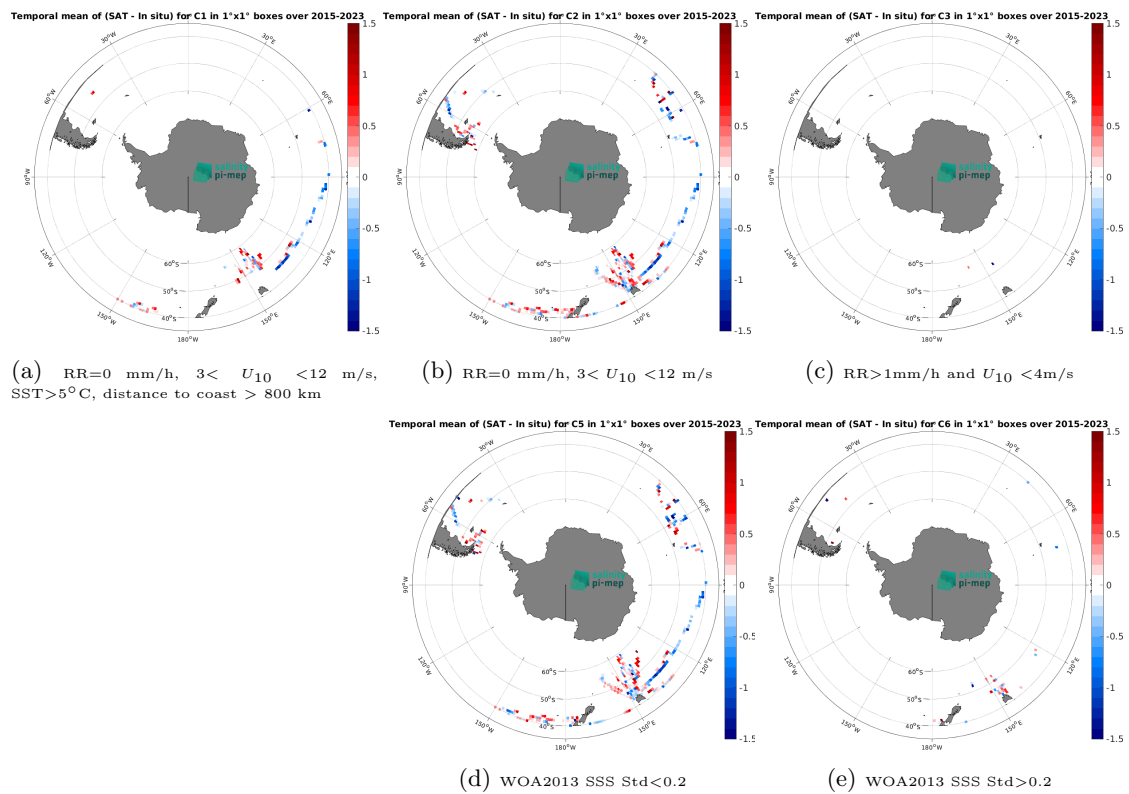
Figure 14: Temporal mean gridded over spatial boxes of size 1^\circ \times 1^\circ of \Delta SSS (SMAP SSS L2 v5.3 (RSS) - TSG (LEGOS-DM)) for 5 different subdatasets corresponding to:RR=0 mm/h, 3 < U_{10} < 12 m/s, SST >5^\circ\text{C} , distance to coast > 800 km (a), RR=0 mm/h, 3 < U_{10} < 12 m/s (b), RR >1 mm/h and U_{10} < 4 m/s (c), WOA2013 SSS Std <0.2 (d), WOA2013 SSS Std >0.2 (e).
