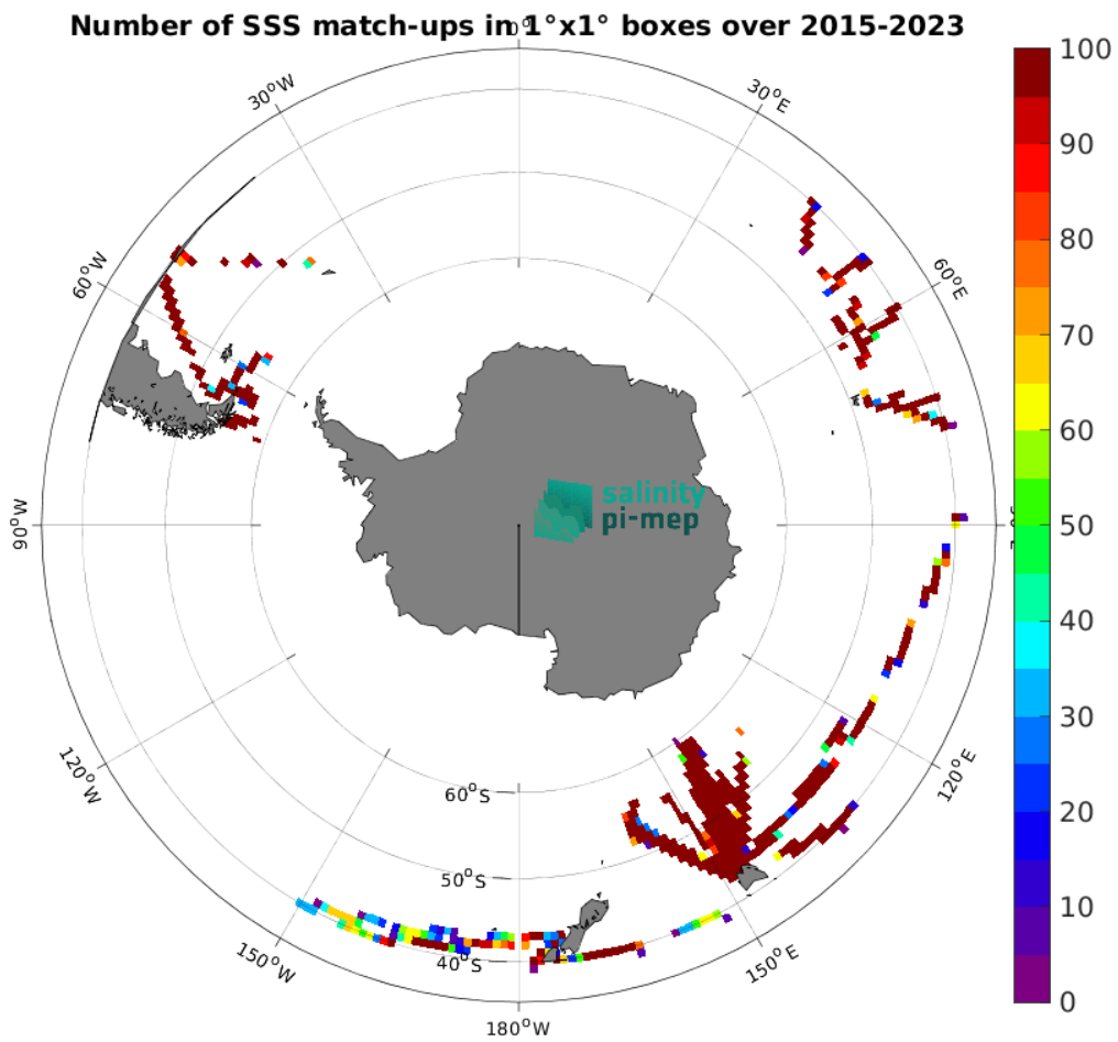
Figure 5: Number of SSS match-ups between TSG (LEGOS-DM) SSS and the SMAP SSS L2 v5.3 (RSS) SSS product for the Roaring Forties and Furious Fifties Pi-MEP region over 1^\circ \times 1^\circ boxes and for the full satellite product period.
