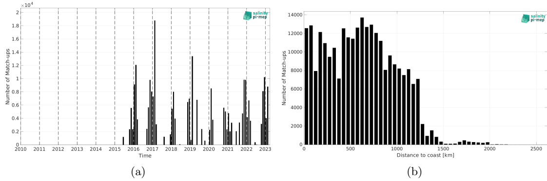
Figure 2: Number of match-ups between TSG (LEGOS-DM) and SMAP SSS L2 v5.3 (RSS) SSS as a function of time (a) and as function of the distance to coast (b) over the Roaring Forties and Furious Fifties Pi-MEP region and for the full satellite product period.
