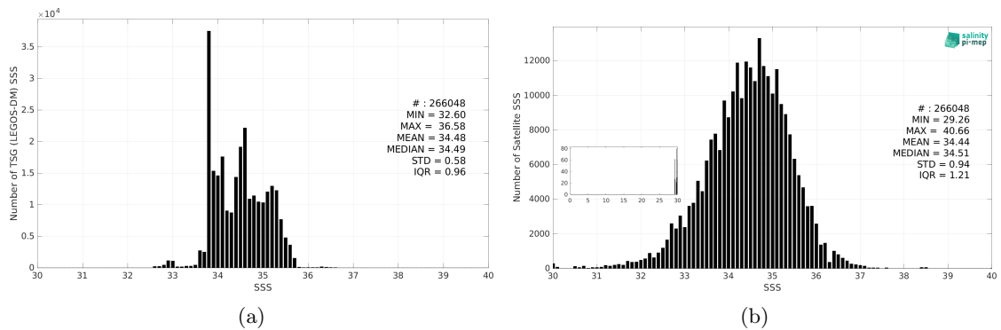
Figure 3: Histograms of SSS from TSG (LEGOS-DM) (a) and SMAP SSS L2 v5.3 (RSS) (b) considering all match-up pairs per bins of 0.1 over the Roaring Forties and Furious Fifties Pi-MEP region and for the full satellite product period.
