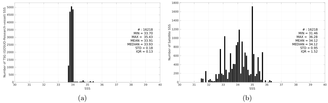
Figure 3: Histograms of SSS from TSG (GOSUD-Research-vessel) (a) and SMAP SSS L2 v5.3 (RSS) (b) considering all match-up pairs per bins of 0.1 over the Roaring Forties and Furious Fifties Pi-MEP region and for the full satellite product period.
