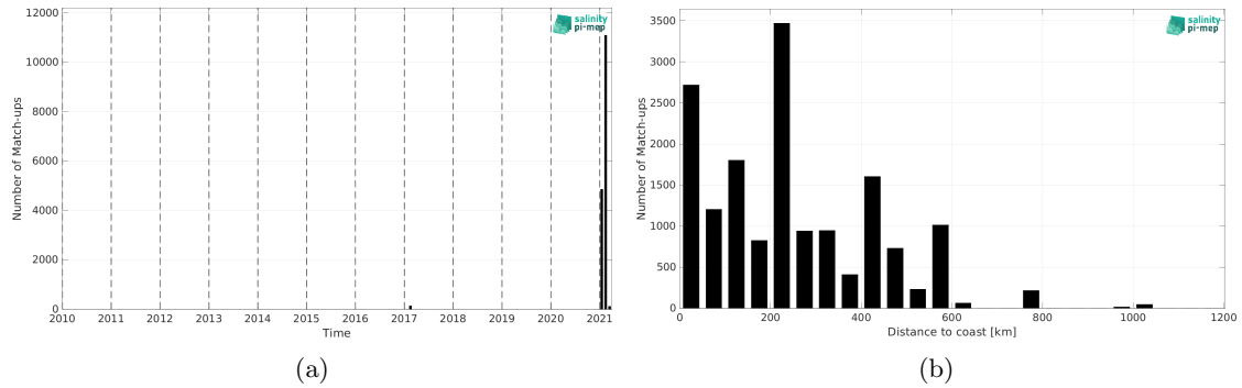
Figure 2: Number of match-ups between TSG (GOSUD-Research-vessel) and SMAP SSS L2 v5.3 (RSS) SSS as a function of time (a) and as function of the distance to coast (b) over the Roaring Forties and Furious Fifties Pi-MEP region and for the full satellite product period.
