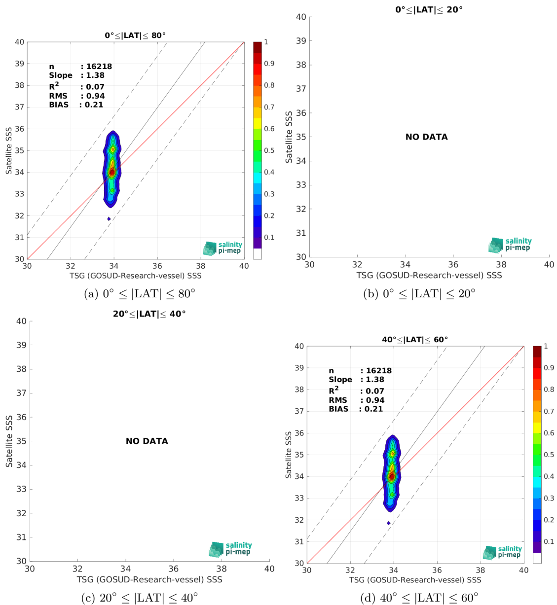
Figure 10: Contour maps of the concentration of SMAP SSS L2 v5.3 (RSS) SSS (y-axis) versus TSG (GOSUD-Research-vessel) SSS (x-axis) at match-up pairs for different latitude bands. For each plot, the red line shows x=y . The black thin and dashed lines indicate a linear fit through the data cloud and the \pm 95\% confidence levels, respectively. The number match-up pairs n , the slope and R^2 coefficient of the linear fit, the root mean square (RMS) and the mean bias between satellite and in situ data are indicated for each latitude band in each plots.
