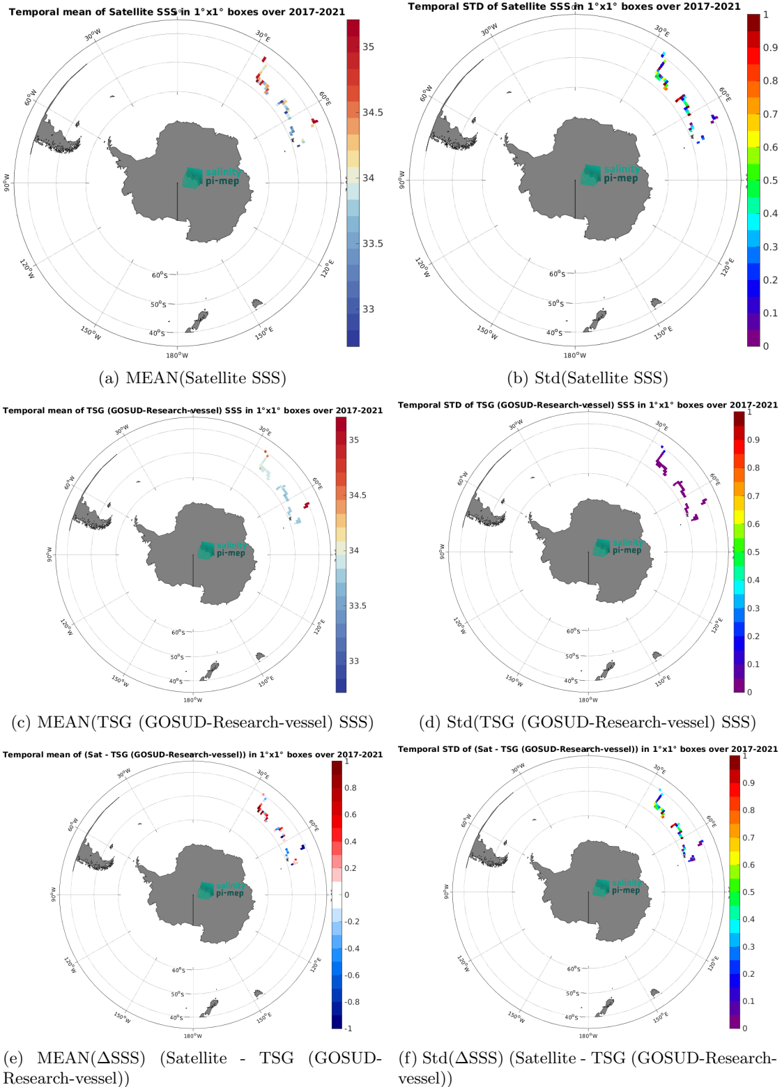
Figure 7: Temporal mean (left) and Std (right) of SSS from SMAP SSS L2 v5.3 (RSS) (top), TSG (GOSUD-Research-vessel) (middle), and of \Delta SSS (Satellite - TSG (GOSUD-Research-vessel)). Only match-up pairs are used to generate these maps.
