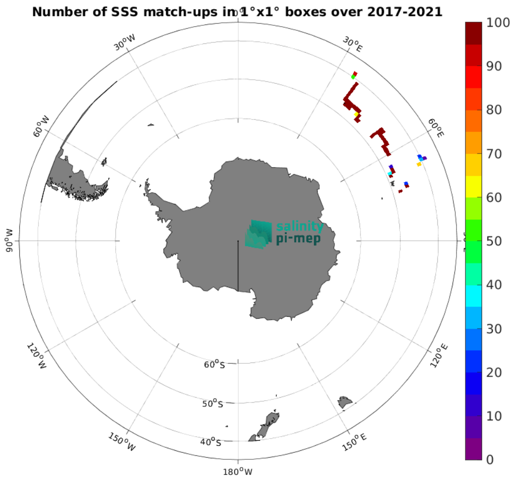
Figure 5: Number of SSS match-ups between TSG (GOSUD-Research-vessel) SSS and the SMAP SSS L2 v5.3 (RSS) SSS product for the Roaring Forties and Furious Fifties Pi-MEP region over 1^\circ \times 1^\circ boxes and for the full satellite product period.
