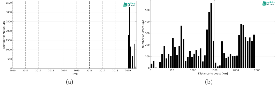
Figure 2: Number of match-ups between Saildrone and SMAP SSS L2 v5.3 (RSS) SSS as a function of time (a) and as function of the distance to coast (b) over the Roaring Forties and Furious Fifties Pi-MEP region and for the full satellite product period.
