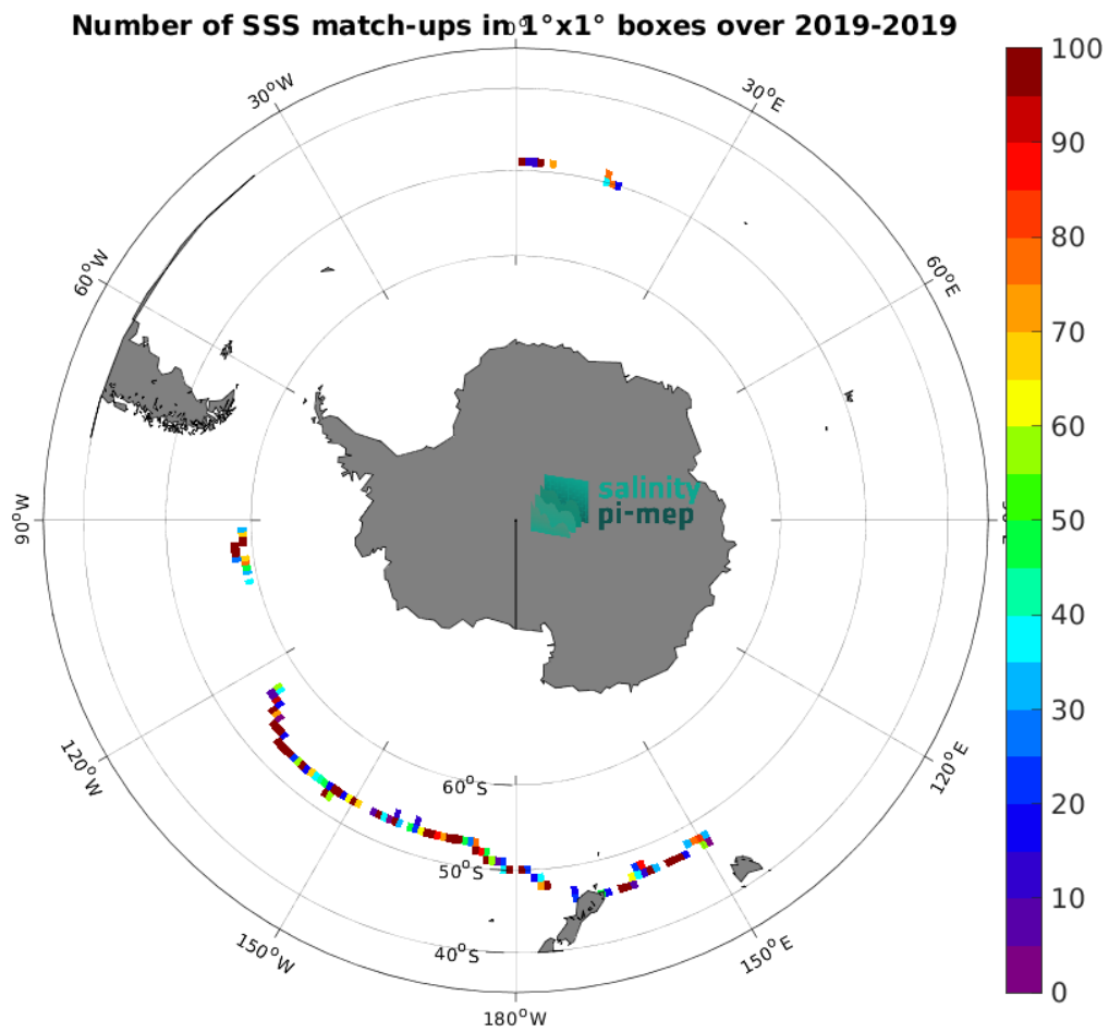
Figure 5: Number of SSS match-ups between Saildrone SSS and the SMAP SSS L2 v5.3 (RSS) SSS product for the Roaring Forties and Furious Fifties Pi-MEP region over 1^\circ \times 1^\circ boxes and for the full satellite product period.
