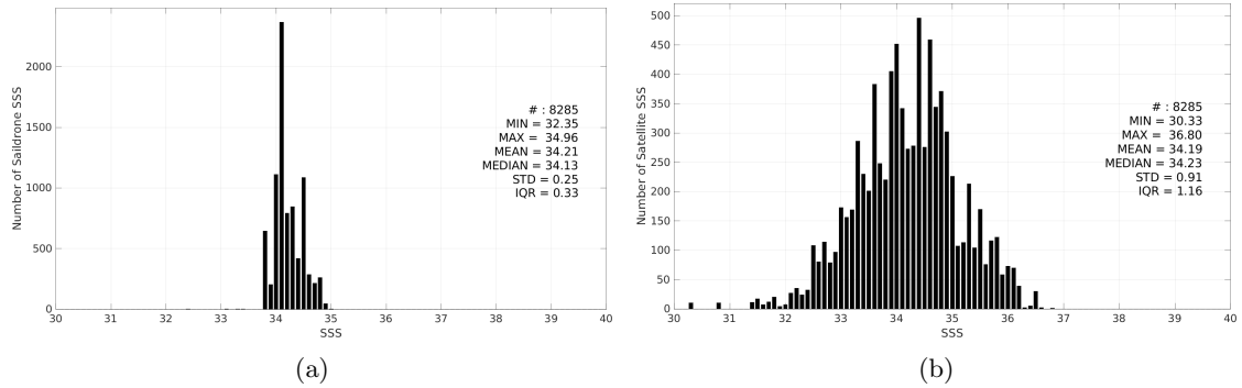
Figure 3: Histograms of SSS from Saildrone (a) and SMAP SSS L2 v5.3 (RSS) (b) considering all match-up pairs per bins of 0.1 over the Roaring Forties and Furious Fifties Pi-MEP region and for the full satellite product period.
