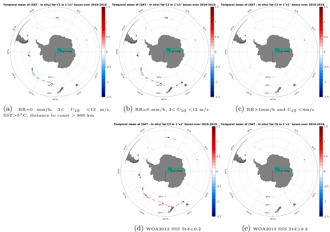
Figure 14: Temporal mean gridded over spatial boxes of size 1^\circ \times 1^\circ of \Delta SSS (SMAP SSS L2 v5.3 (RSS) - Saildrone) for 5 different subdatasets corresponding to:RR=0 mm/h, 3 < U_{10} < 12 m/s, SST>5°C, distance to coast > 800 km (a), RR=0 mm/h, 3 < U_{10} < 12 m/s (b), RR>1mm/h and U_{10} < 4 m/s (c), WOA2013 SSS Std<0.2 (d), WOA2013 SSS Std>0.2 (e).
