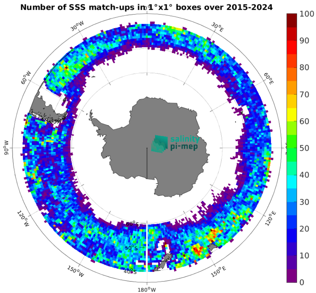
Figure 5: Number of SSS match-ups between Argo SSS and the SMAP SSS L2 v5.3 (RSS) SSS product for the Roaring Forties and Furious Fifties Pi-MEP region over 1^\circ \times 1^\circ boxes and for the full satellite product period.
