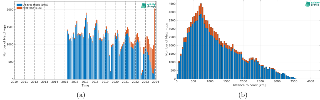
Figure 2: Number of match-ups between Argo and SMAP SSS L2 v5.3 (RSS) SSS as a function of time (a) and as function of the distance to coast (b) over the Roaring Forties and Furious Fifties Pi-MEP region and for the full satellite product period.
