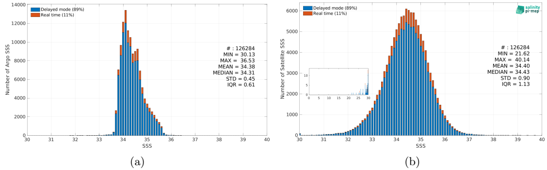
Figure 3: Histograms of SSS from Argo (a) and SMAP SSS L2 v5.3 (RSS) (b) considering all match-up pairs per bins of 0.1 over the Roaring Forties and Furious Fifties Pi-MEP region and for the full satellite product period.
