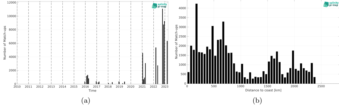
Figure 2: Number of match-ups between TSG (Polarstern) and SMAP SSS L2 v5.3 - 40 km (RSS) SSS as a function of time (a) and as function of the distance to coast (b) over the Roaring Forties and Furious Fifties Pi-MEP region and for the full satellite product period.
