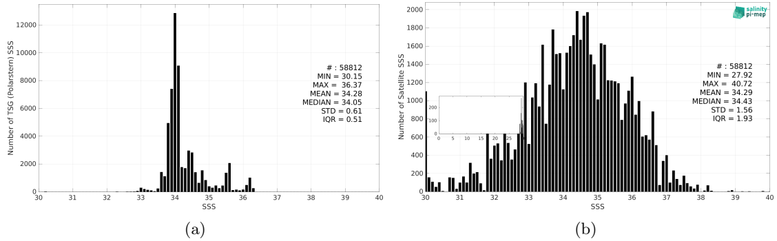
Figure 3: Histograms of SSS from TSG (Polarstern) (a) and SMAP SSS L2 v5.3 - 40 km (RSS) (b) considering all match-up pairs per bins of 0.1 over the Roaring Forties and Furious Fifties Pi-MEP region and for the full satellite product period.
