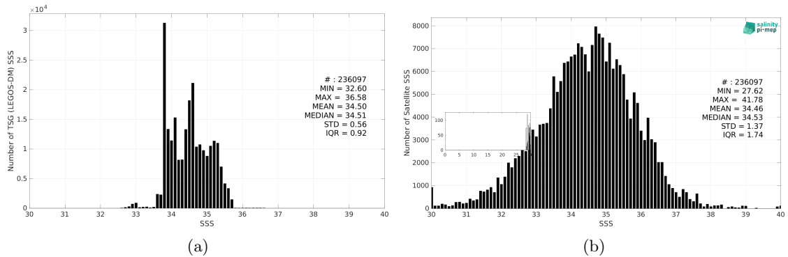
Figure 3: Histograms of SSS from TSG (LEGOS-DM) (a) and SMAP SSS L2 v5.3 - 40 km (RSS) (b) considering all match-up pairs per bins of 0.1 over the Roaring Forties and Furious Fifties Pi-MEP region and for the full satellite product period.
