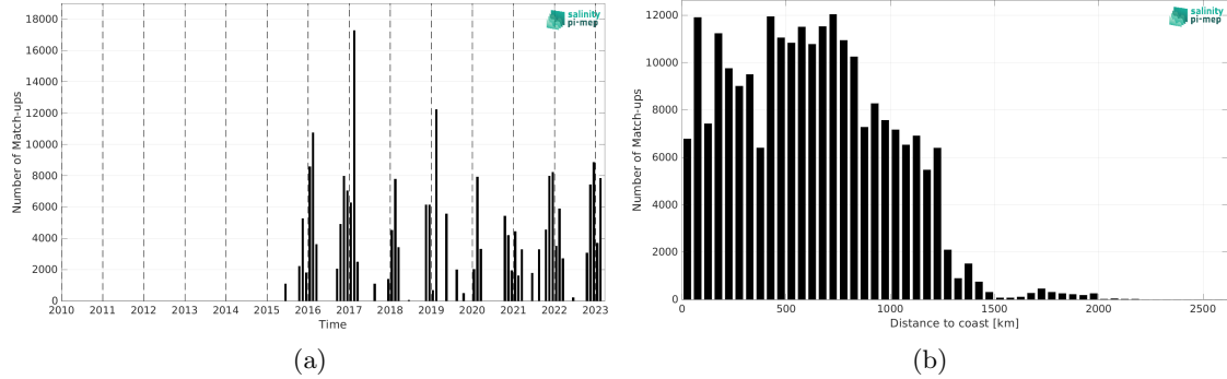
Figure 2: Number of match-ups between TSG (LEGOS-DM) and SMAP SSS L2 v5.3 - 40 km (RSS) SSS as a function of time (a) and as function of the distance to coast (b) over the Roaring Forties and Furious Fifties Pi-MEP region and for the full satellite product period.
