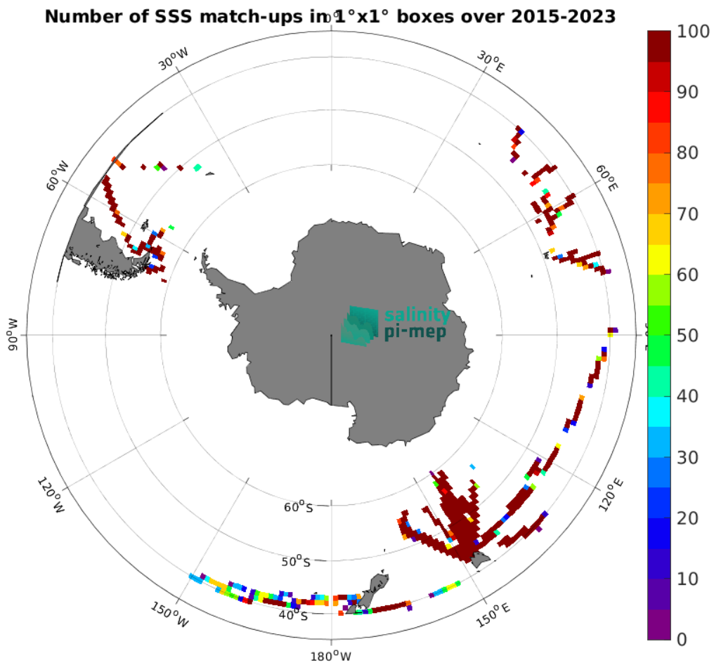
Figure 5: Number of SSS match-ups between TSG (LEGOS-DM) SSS and the SMAP SSS L2 v5.3 - 40 km (RSS) SSS product for the Roaring Forties and Furious Fifties Pi-MEP region over 1^\circ \times 1^\circ boxes and for the full satellite product period.
