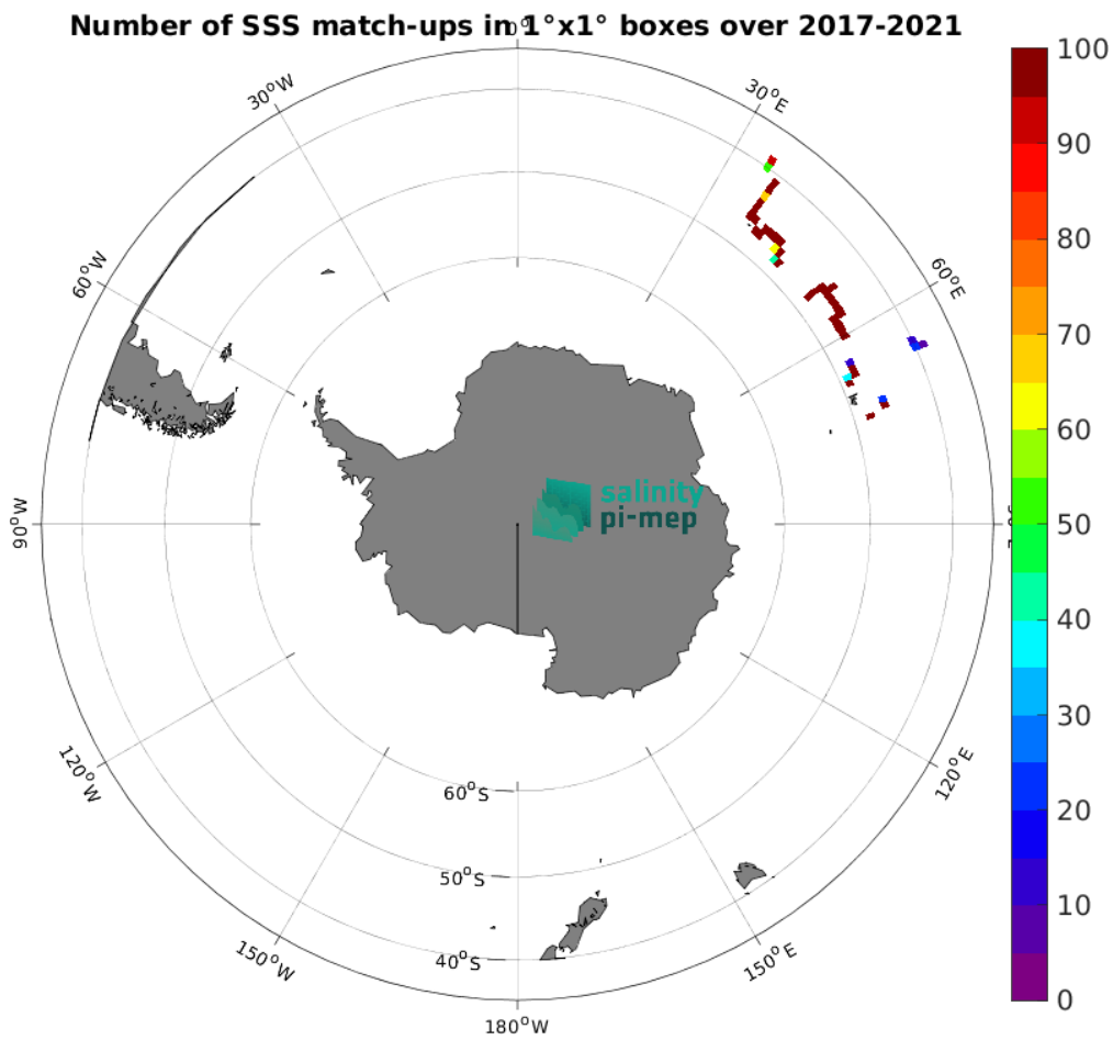
Figure 5: Number of SSS match-ups between TSG (GOSUD-Research-vessel) SSS and the SMAP SSS L2 v5.3 - 40 km (RSS) SSS product for the Roaring Forties and Furious Fifties Pi-MEP region over 1^\circ \times 1^\circ boxes and for the full satellite product period.
