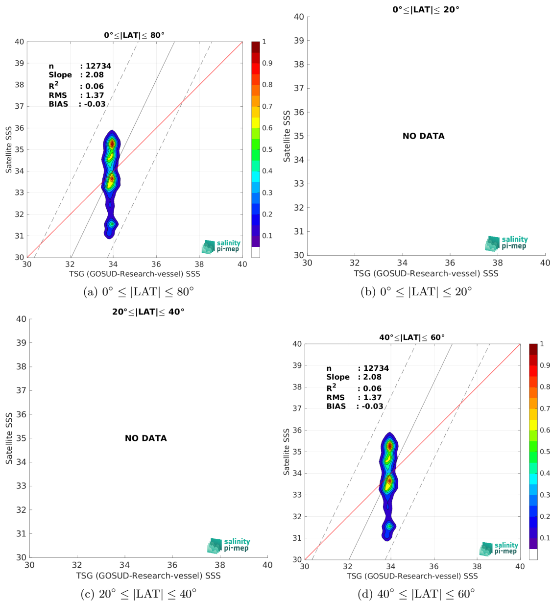
Figure 10: Contour maps of the concentration of SMAP SSS L2 v5.3 - 40 km (RSS) SSS (y-axis) versus TSG (GOSUD-Research-vessel) SSS (x-axis) at match-up pairs for different latitude bands. For each plot, the red line shows x=y . The black thin and dashed lines indicate a linear fit through the data cloud and the \pm 95\% confidence levels, respectively. The number match-up pairs n , the slope and R^2 coefficient of the linear fit, the root mean square (RMS) and the mean bias between satellite and in situ data are indicated for each latitude band in each plot.
