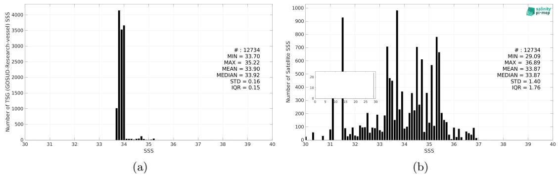
Figure 3: Histograms of SSS from TSG (GOSUD-Research-vessel) (a) and SMAP SSS L2 v5.3 - 40 km (RSS) (b) considering all match-up pairs per bins of 0.1 over the Roaring Forties and Furious Fifties Pi-MEP region and for the full satellite product period.
