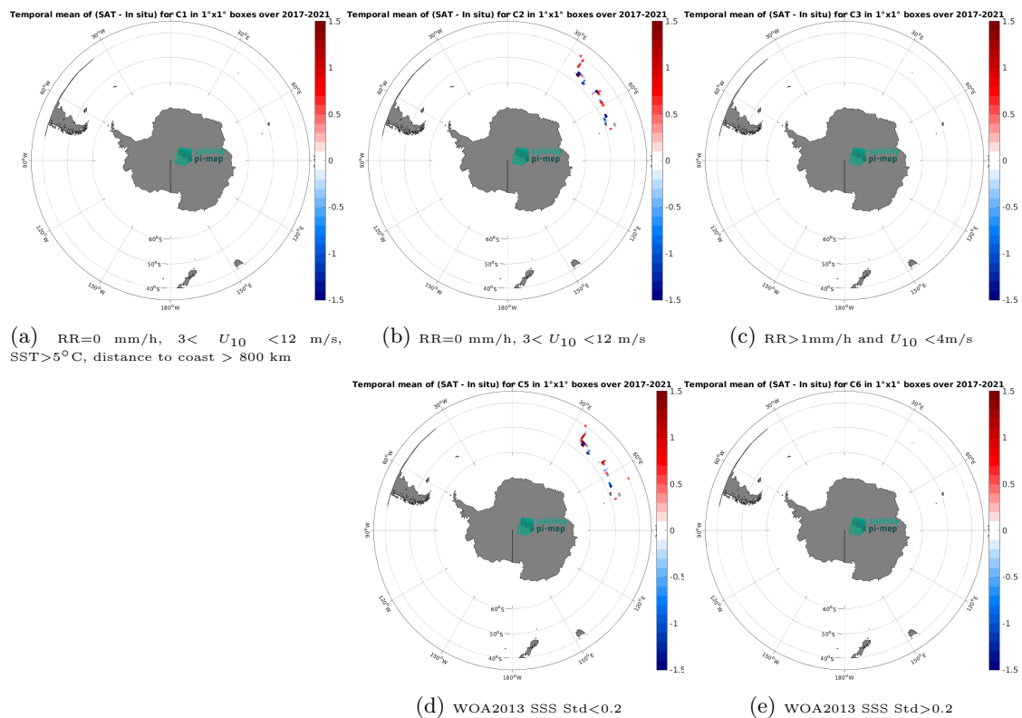
Figure 14: Temporal mean gridded over spatial boxes of size 1^\circ \times 1^\circ of \Delta SSS (SMAP SSS L2 v5.3 - 40 km (RSS) - TSG (GOSUD-Research-vessel)) for 5 different subdatasets corresponding to:RR=0 mm/h, 3 < U_{10} < 12 m/s, SST>5°C, distance to coast > 800 km (a), RR=0 mm/h, 3 < U_{10} < 12 m/s (b), RR>1mm/h and U_{10} < 4 m/s (c), WOA2013 SSS Std<0.2 (d), WOA2013 SSS Std>0.2 (e).
