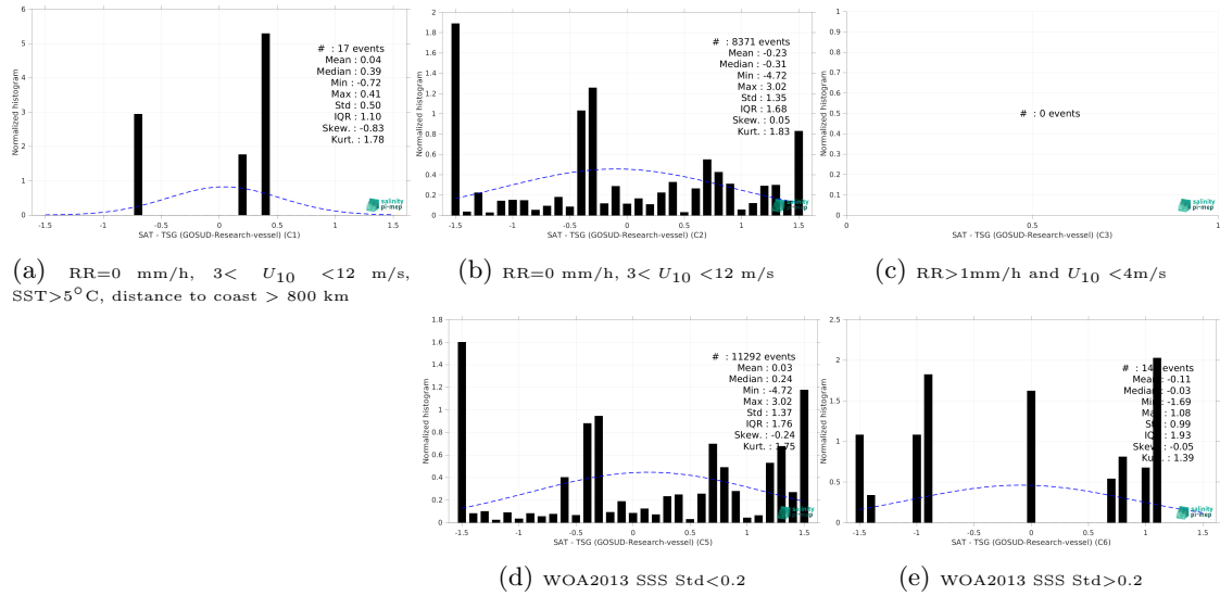
Figure 15: Normalized histogram of \Delta\text{SSS} (SMAP SSS L2 v5.3 - 40 km (RSS) - TSG (GOSUD-Research-vessel)) for 5 different subdatasets corresponding to: RR=0 mm/h, 3 < U_{10} < 12 m/s, SST > 5^{\circ}\text{C} , distance to coast > 800 km (a), RR=0 mm/h, 3 < U_{10} < 12 m/s (b), RR > 1\text{mm/h} and U_{10} < 4\text{m/s} (c), WOA2013 SSS Std < 0.2 (d), WOA2013 SSS Std > 0.2 (e).
