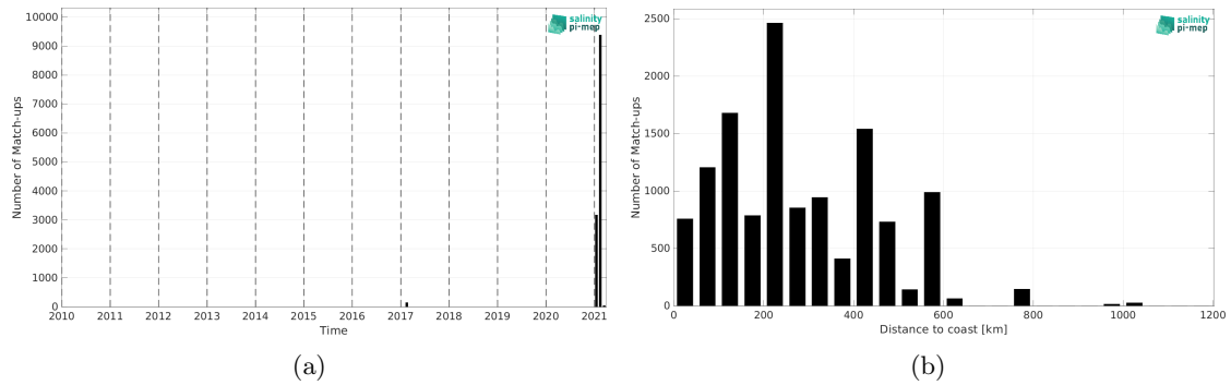
Figure 2: Number of match-ups between TSG (GOSUD-Research-vessel) and SMAP SSS L2 v5.3 - 40 km (RSS) SSS as a function of time (a) and as function of the distance to coast (b) over the Roaring Forties and Furious Fifties Pi-MEP region and for the full satellite product period.
