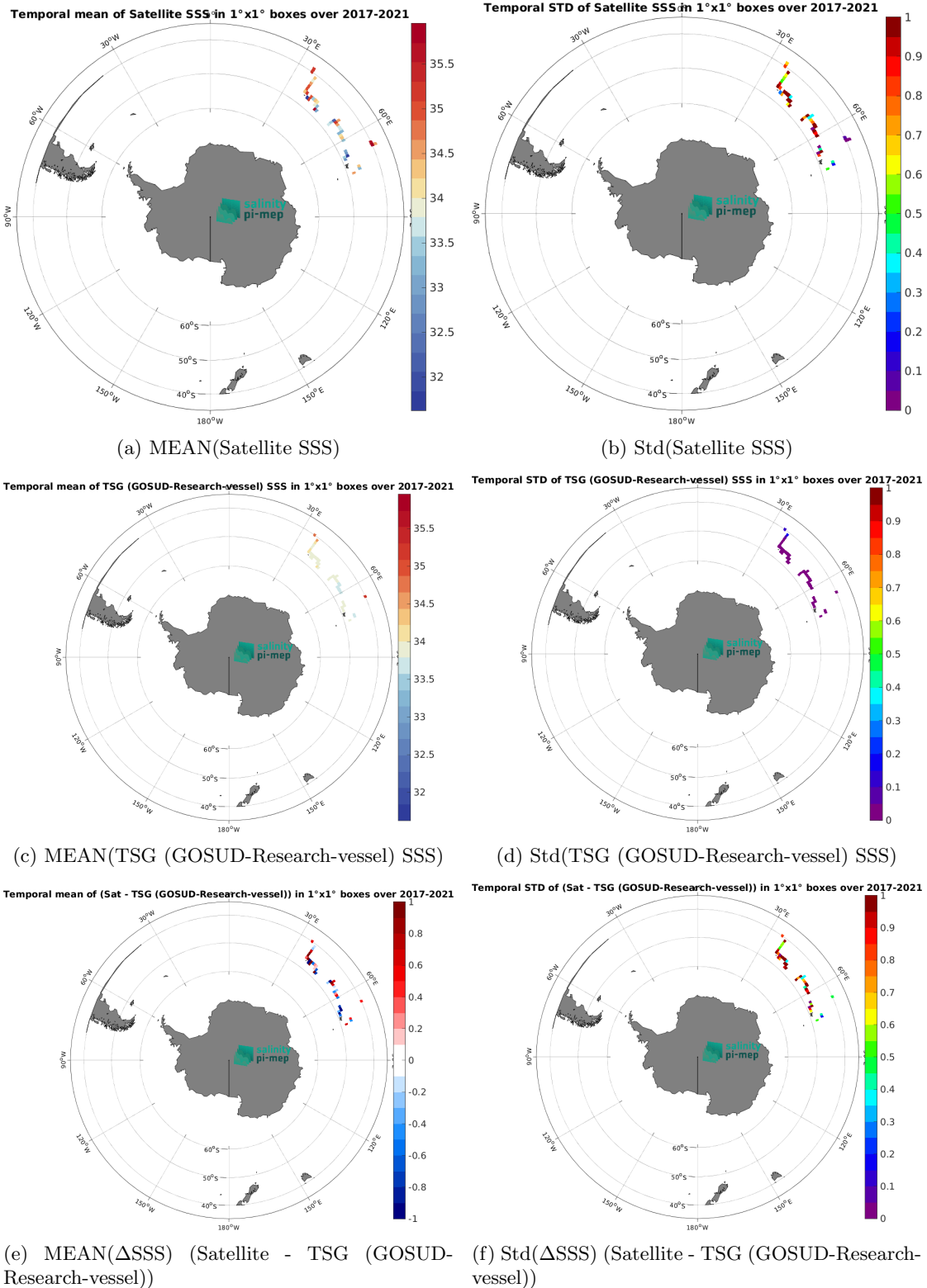
Figure 7: Temporal mean (left) and Std (right) of SSS from SMAP SSS L2 v5.3 - 40 km (RSS) (top), TSG (GOSUD-Research-vessel) (middle), and of \Delta SSS (Satellite - TSG (GOSUD-Research-vessel)). Only match-up pairs are used to generate these maps.
