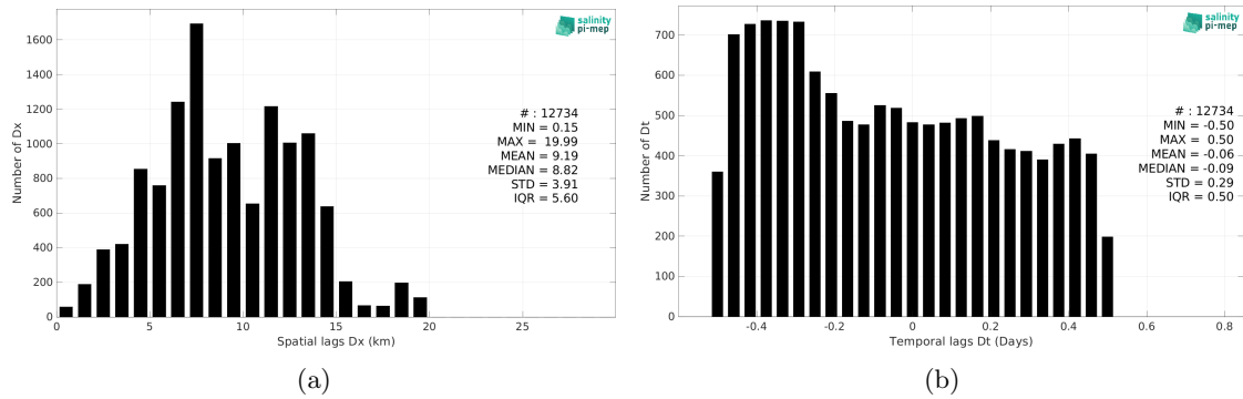
Figure 6: Histograms of the spatial (a) and temporal (b) lags between the location/time of the TSG (GOSUD-Research-vessel) measurement and the date of the corresponding SMAP SSS L2 v5.3 - 40 km (RSS) SSS pixel.
